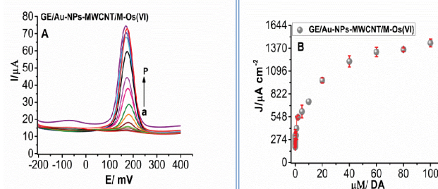
Figure 7 (A) DPV of GE/AuNPs-MWCNT/Man-Os (VI) tmen was measured at the DA concentration range from (a-p) 0.001 pM-100 \mu\text{M} in the presence of excess concentration of (5 mM AA and 0.5 mM UA). (B) Current density plot of the GE/AuNPs-MWCNT/Man-Os (VI) tmen via different concentration of DA at 10 mV/s scan rate, vs. Ag|AgCl|(KCl sat.).
