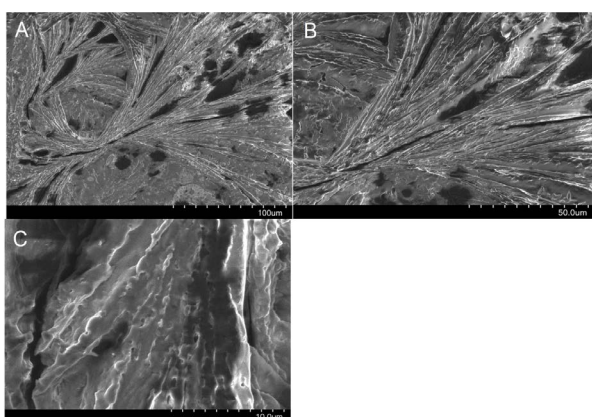
Figure 5C (C) SEM-images of modified GE/AuNPs-MWCNTs/Man-Os (VI) tmen at different magnifications. (A) 500 X, (B) 1000 X, (C) 5000 X. 1 mg/ml concentration solution of AuNPs-MWCNTs at 5000 accelerated voltage.
