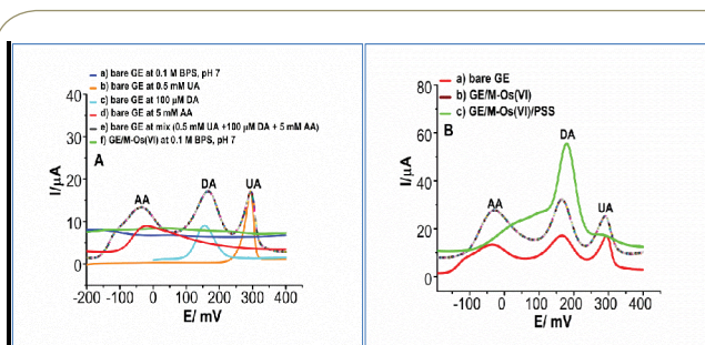
Figure 3 (A) DPV measurements of bare GE in PBS 0.1 M, pH 7 (blue line), bare GE in 0.5 mM UA (orange line), bare GE in 100 \mu M DA (cyan line), bare GE in 5 mM AA (red line), bare GE in the mixture of a solution (0.5 mM UA+100 \mu M DA+5 mM AA) (Increment: mixture of gray line), GE/Man-Os (VI) tmen in PBS 0.1 M, pH 7 (green line). (B) Bare GE at mix (100 \mu M DA+5 mM AA+0.5 mM UA) (a: red line), GE/Man-Os (VI) tmen in a solution mixture of (100 \mu M DA+5 mM AA+0.5 mM UA) (b: mixture of gray color ), GE/Man-Os (VI) tmen/PSS in the mixture of (100 \mu M DA+5 mM AA+0.5 mM UA) (c: green line), at 10 mV/s scan rate vs. Ag| AgCl| (KCl sat.) reference electrode.
