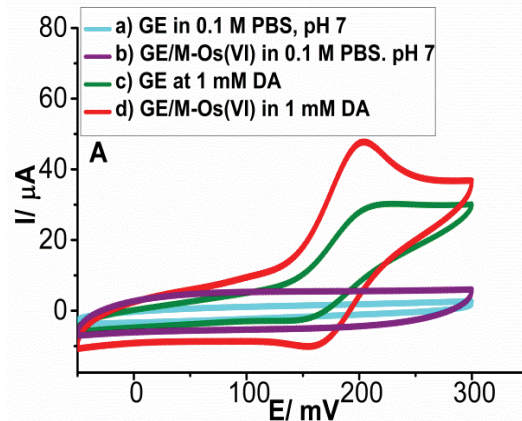
Figure 1 (A) Cyclic voltammograms of bare GE at PBS 0.1\text{ M} , pH 7 (a: cyan), GE/Man-Os (VI) tmen in PBS 0.1\text{ M} pH 7 (b: violet), bare GE in 1\text{ mM} DA (c: green), and GE/Man-Os (VI) tmen with 1\text{ mM} DA (d: red), at 10\text{ mV/s} scan rate vs. \text{Ag}|\text{AgCl}| \text{KCl}_{\text{sat}} reference electrode.
