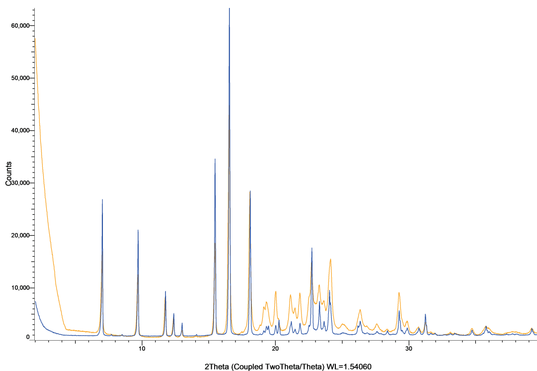
Figure S47: XRPD patterns of etorixcoxib powder (blue) and milled etorixcoxib powder (orange).
