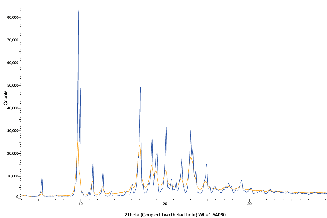
Figure S39: XRPD patterns of candesartan cilexetil powder (blue) and milled candesartan cilexetil powder (orange).
