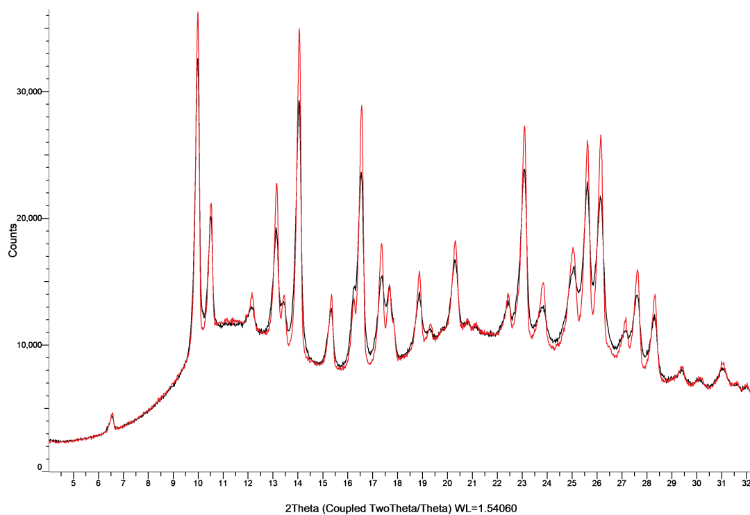
Figure S16: XRPD patterns of deferasirox with PVP K25 in co-milled mixtures (black) and physical mixtures (red).
