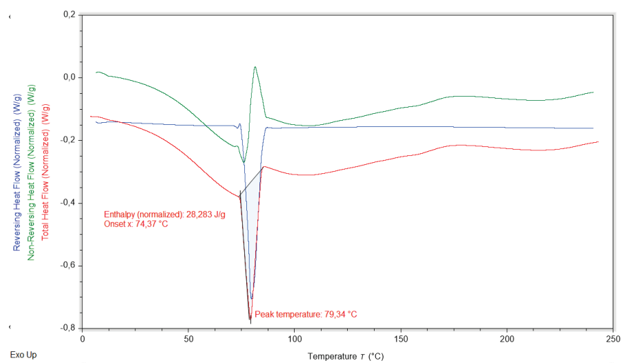
Figure S96: Thermograms illustrating the thermal behavior of fenofibrate co-milled with croscarmellose sodium at a 1:2 (w/w) ratio after 5 min of co-milling, measured after 3 months of storage.
