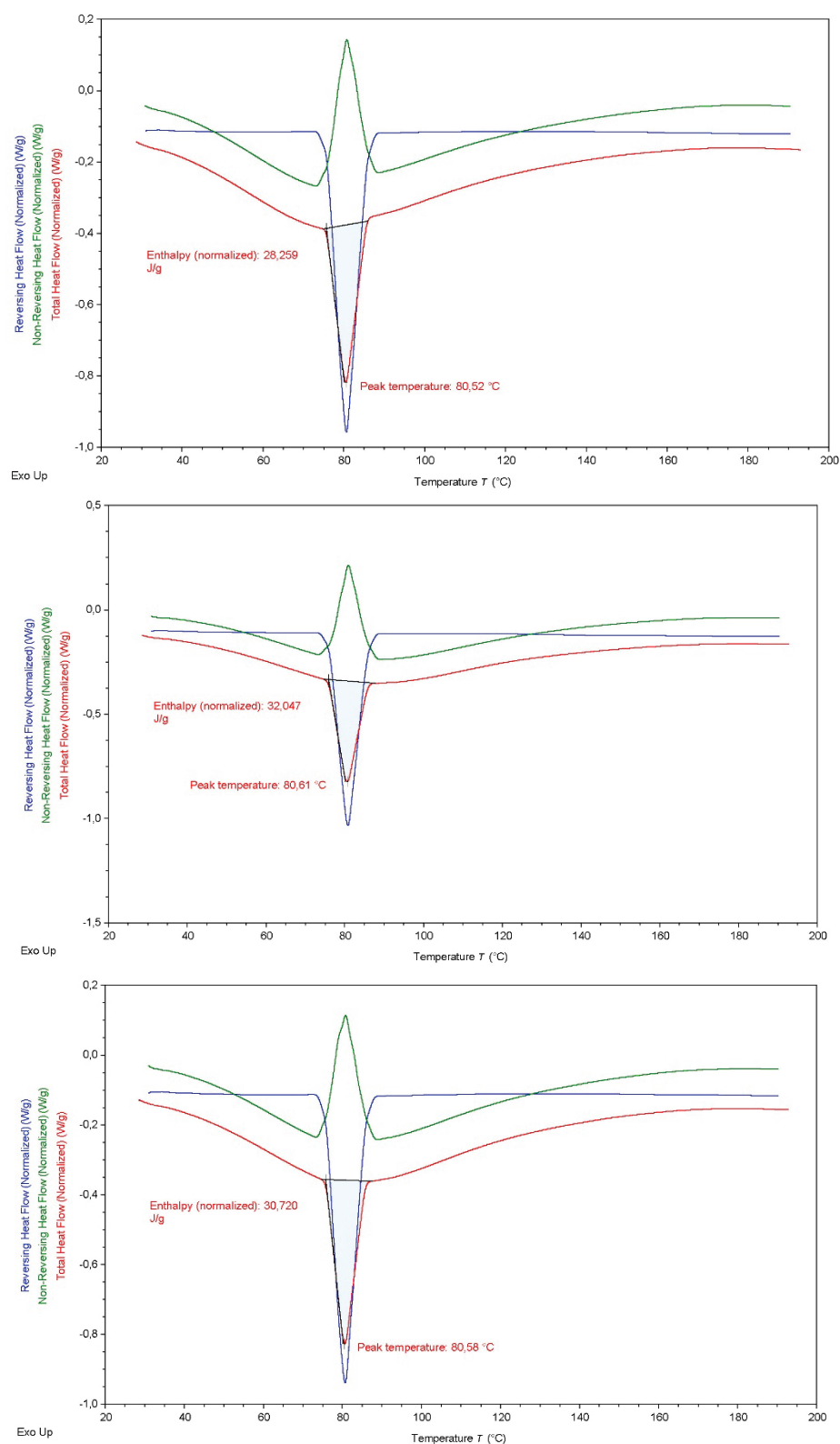
Figure S79: Thermograms illustrating the thermal behavior of fenofibrate co-milled with croscarmellose sodium at a 1:2 (w/w) ratio after 15 s of co-milling, measured freshly after preparation.
