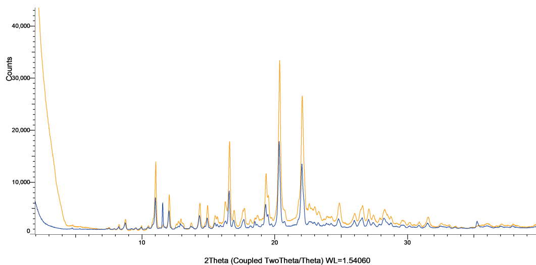
Figure S38: XRPD patterns of aripiprazole powder (blue) and milled aripiprazole powder (orange).
