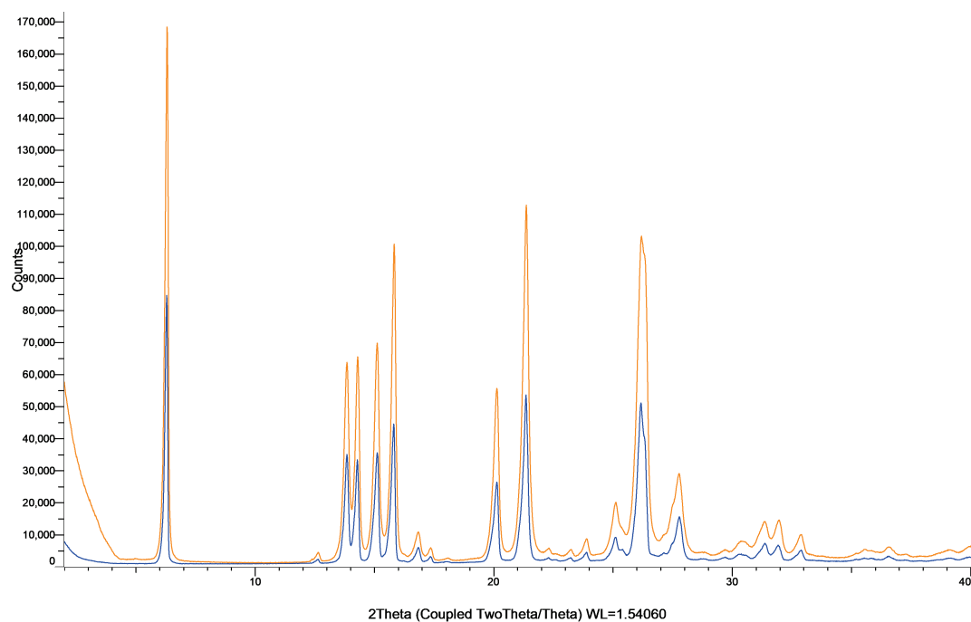
Figure S54: XRPD patterns of mefenamic acid powder (blue) and milled mefenamic acid powder (orange).
