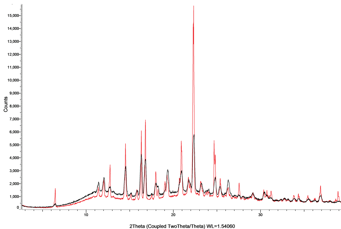
Figure S21: XRPD patterns of fenofibrate with PVP K25 in co-milled mixtures (black) and physical mixtures (red).
