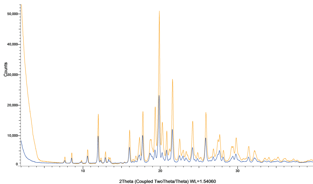
Figure S60: XRPD patterns of sorafenib powder (blue) and milled sorafenib powder (orange).
