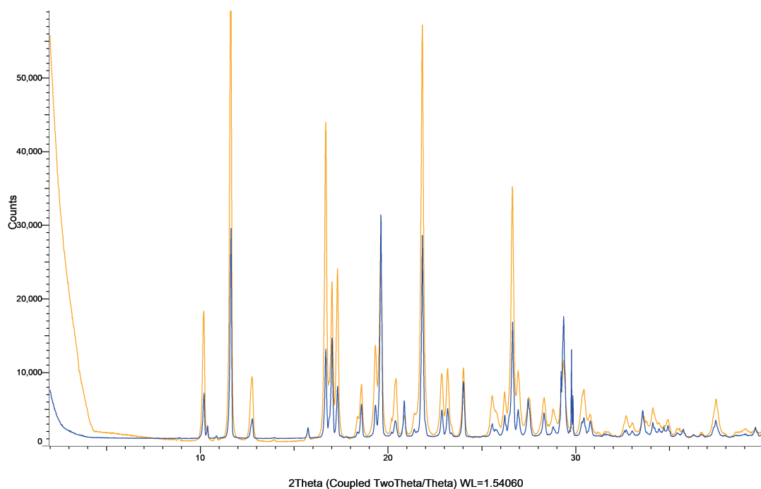
Figure S53: XRPD patterns of indomethacin powder (blue) and milled indomethacin powder (orange).
