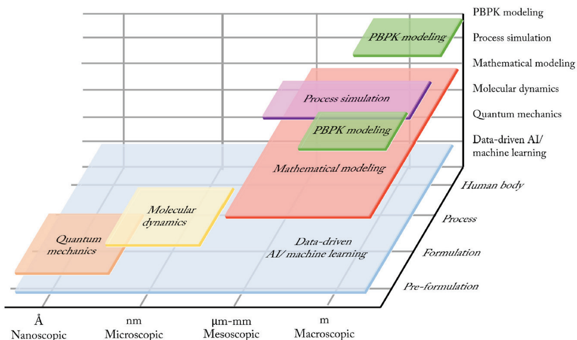
Figure 1-8: Schematic overview of computational pharmaceuticals, extracted from (Wang et al., 2021). The x-axis represents spatial scale from nanoscopic (Å) to macroscopic (m) levels while the y-axis reflects stages of pharmaceutical development, from pre-formulation to modelling of performance in humans. The z-axis shows the types of computational approaches used, including quantum mechanics, molecular dynamics, mathematical and process modelling, PBPK modelling, and data-driven AI or machine learning, each mapped to the scales and processes where they are most applicable,
