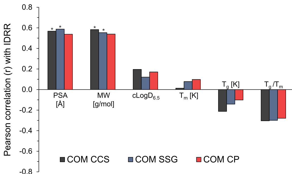
Figure 4-4: Pearson correlations of different single drug properties with the Intrinsic dissolution rate ratio (IDRR), which describes the ratio of the IDR of a co-milled drug divided by the IDR of unmilled drug powder. Following abbreviations were used: Polar Surface Area (PSA); Molecular Weight (MW);
