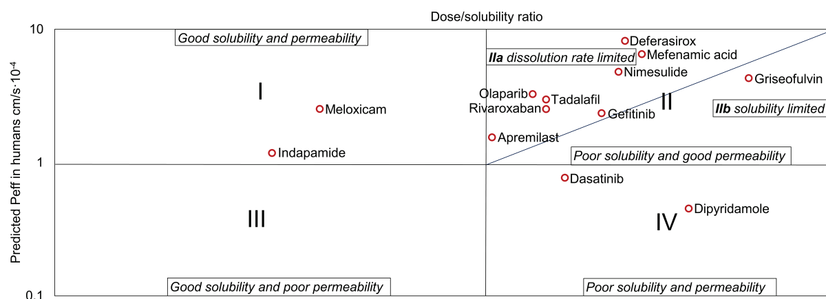
Figure 4-5: The drugs examined in this study were categorised according to the refined Developability Classification System. Usual doses of these compounds in marketed orally administered drug formulations were used to classify the compounds.
