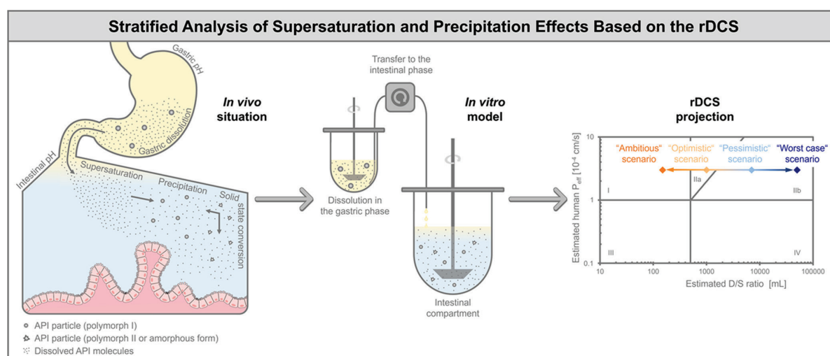
Figure 1-3: Schematic representation of the analysis of supersaturation and precipitation effects based on the rDCS, extracted from (Beran et al., 2024b). The in vivo situation involves drug dissolution in the stomach, supersaturation upon intestinal transfer, and potential precipitation. These processes are simulated using a two-stage in vitro dissolution model. Experimentally derived measured gastric solubility, intestinal solubility, maximum intestinal supersaturation, and average intestinal drug concentration allow the projection of different scenarios into the rDCS diagram to support formulation strategy decisions.
