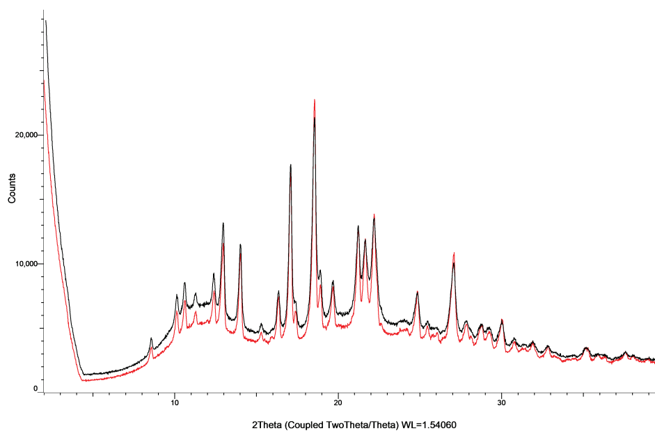
Figure S7: XRPD patterns of apixaban with PVP K25 in co-milled mixtures (black) and physical mixtures (red).
