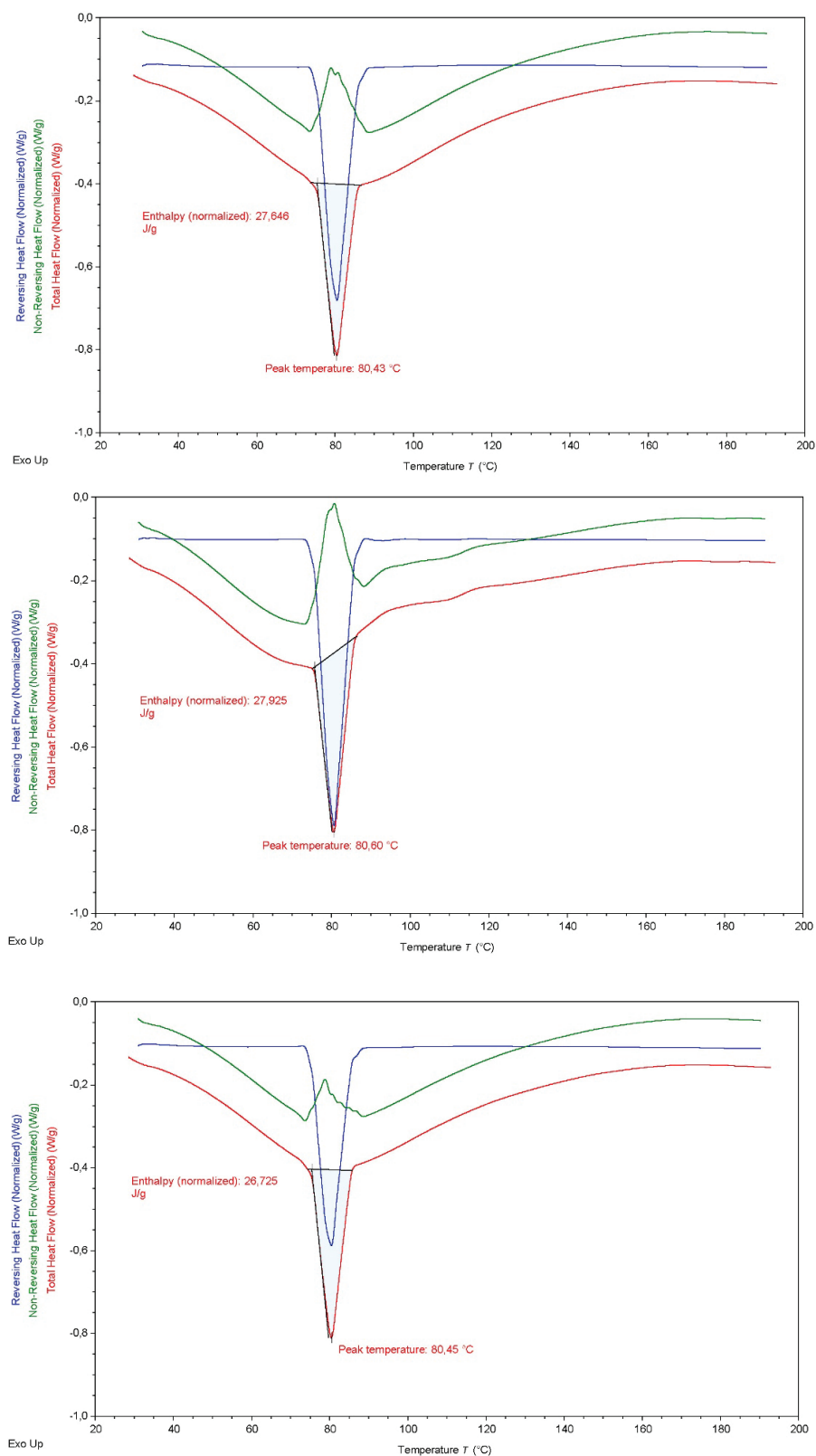
Figure S89: Thermograms illustrating the thermal behavior of fenofibrate co-milled with croscarmellose sodium at a 1:2 (w/w) ratio after 60 min of co-milling, measured freshly after preparation.
