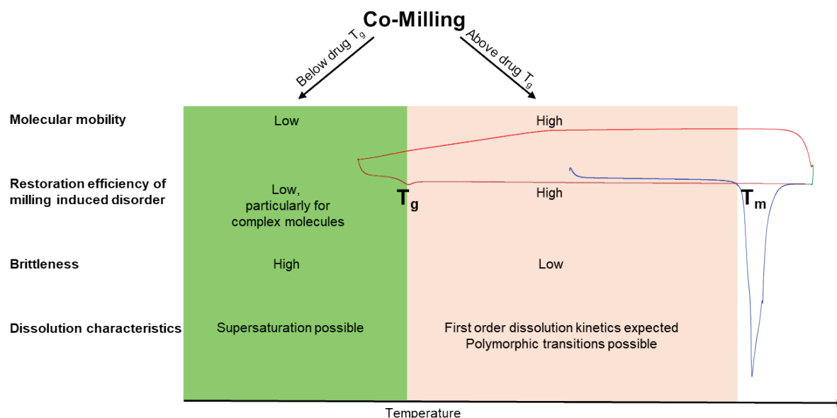
Figure 6-4: Schematic representation of the relationship of the drug glass transition temperature ( T_g ) to the co-milling temperature. Co-milling below T_g , a low molecular mobility and high brittleness favour the retention of milling-induced disorder is expected, especially in structurally complex molecules, enabling supersaturation in dissolution. Co-milling above drug T_g , an increased molecular mobility is promotes the restoration of crystallinity with first-order dissolution kinetics expected. The diagram highlights the critical role of T_g in determining whether co-milling results in stabilized disorder or structural reorganization, and thus its impact on dissolution enhancement. The thermogram is an example of a drug after and quench cooling cycle and serves as a visual orientation for the locations of the T_g and T_m .
