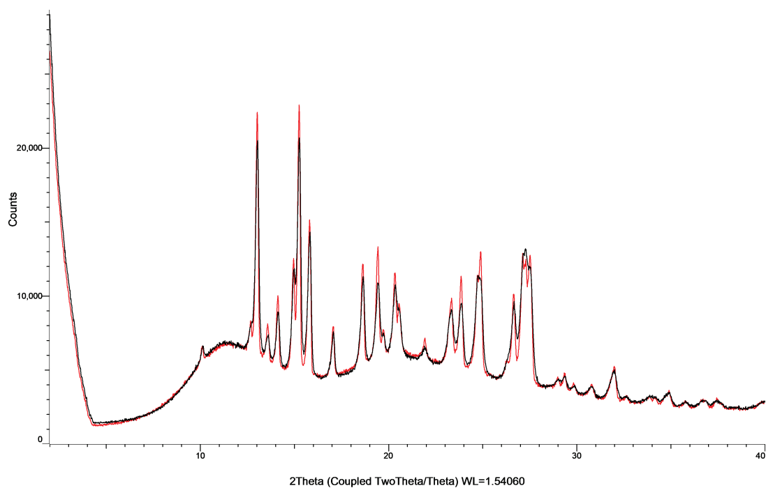
Figure S11: XRPD patterns of carbamazepine with PVP K25 in co-milled mixtures (black) and physical mixtures (red).
