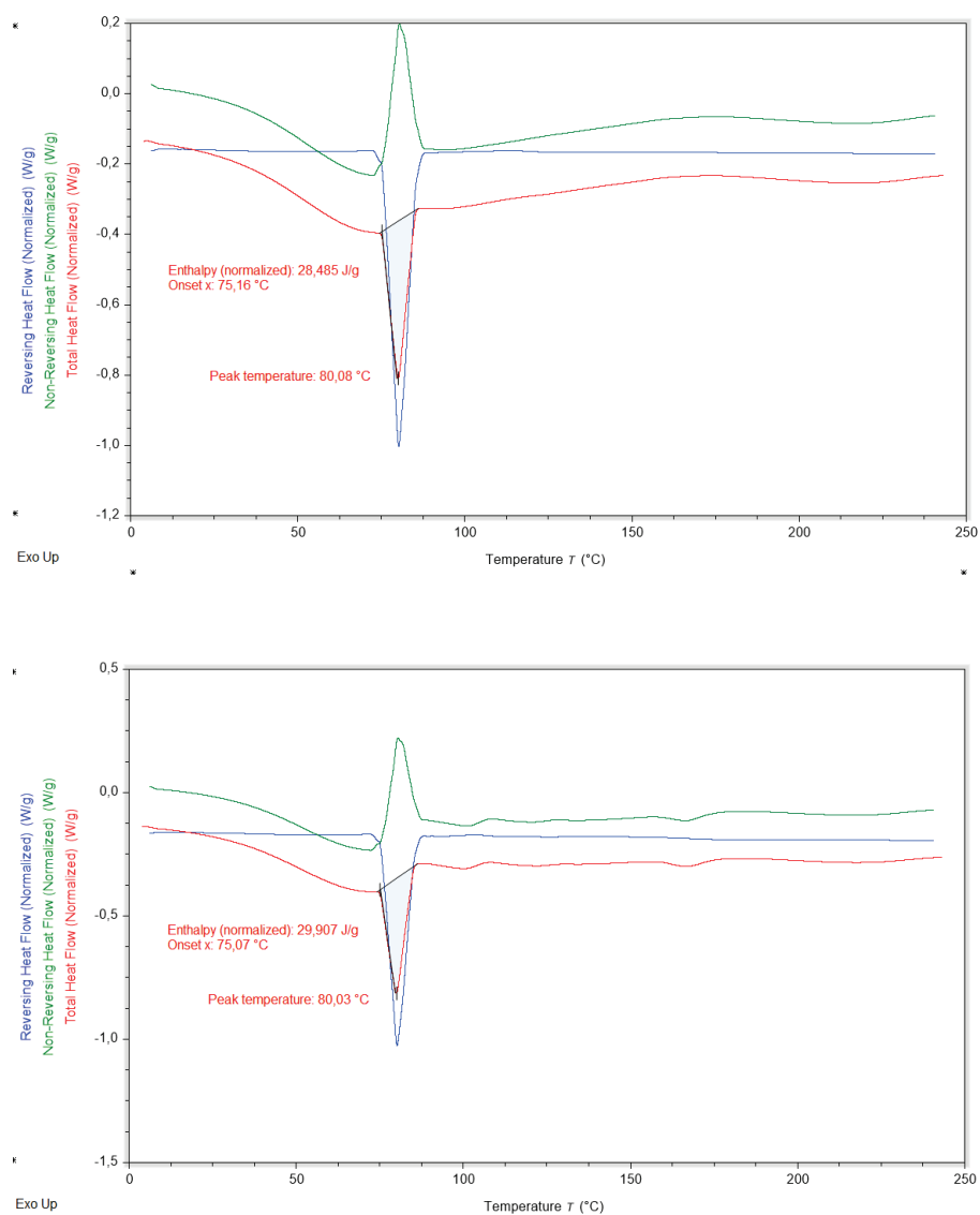
Figure S92: Thermograms illustrating the thermal behavior of fenofibrate co-milled with croscarmellose sodium at a 1:2 (w/w) ratio after 45 s of co-milling, measured after 3 months of storage.
