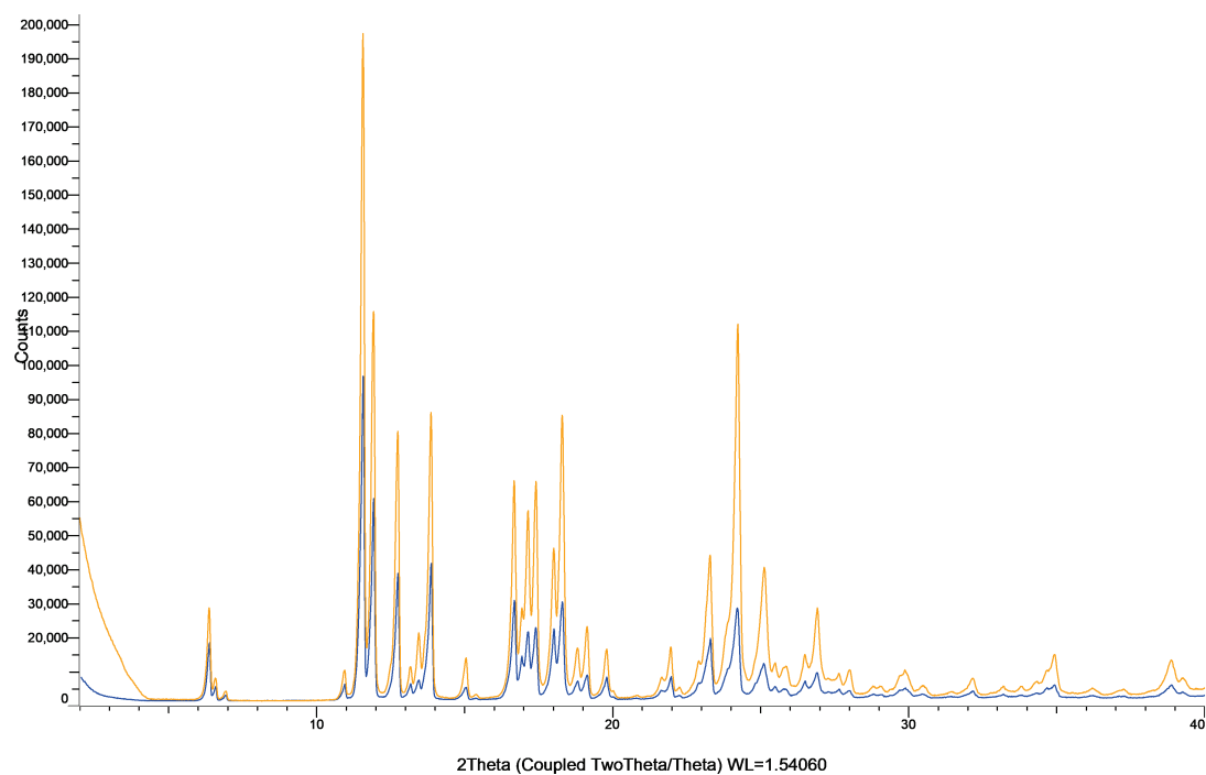
Figure S50: XRPD patterns of gemfibrozil powder (blue) and milled gemfibrozil powder (orange).
