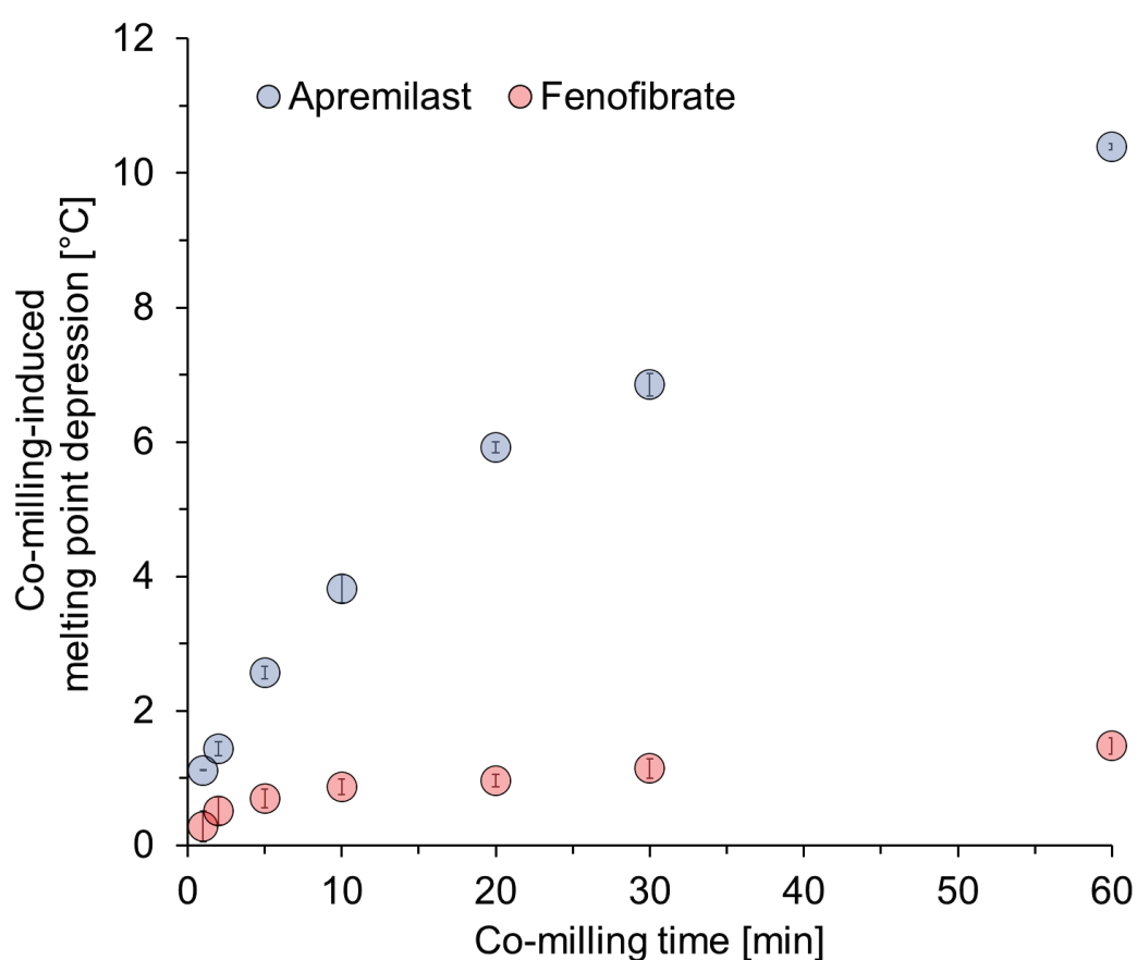
Figure 3-6: Melting point depression, extracted from the onset of the drug melting peak, of co-milled apremilast (high- T_g glass former) and fenofibrate (low- T_g glass former) ( n = 3 ) after various co-milling process duration.
