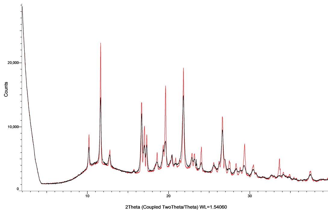
Figure S25: XRPD patterns of indomethacin with PVP K25 in co-milled mixtures (black) and physical mixtures (red).
