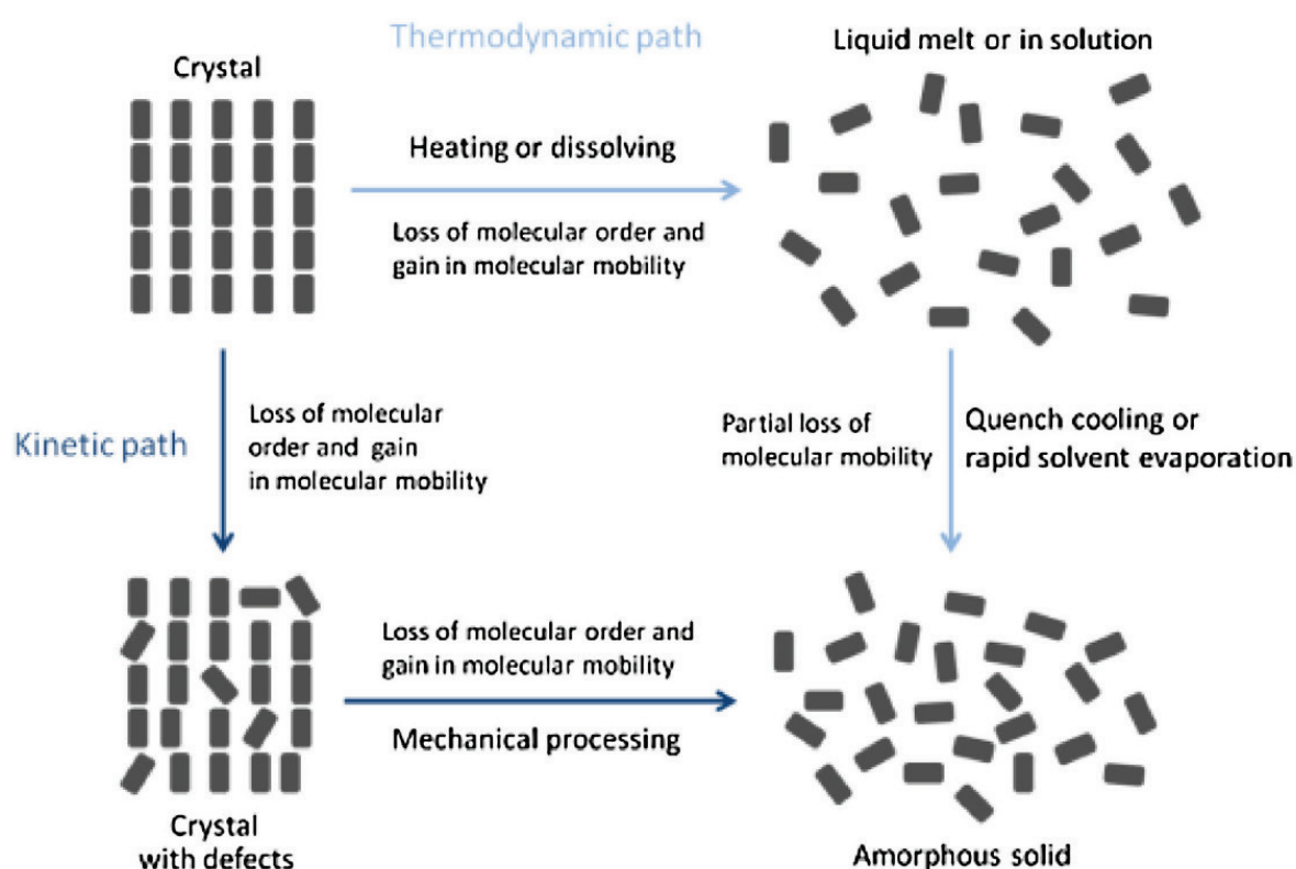
Figure 1-5: Schematic representation of transformation routes from a crystal to an amorphous solid, extracted from (Blaabjerg et al., 2017a). A crystal can lose its crystalline order via mechanical processing (milling) on the kinetic pathway or on the thermodynamic pathway by quench cooling the melt or rapid solvent evaporation.
