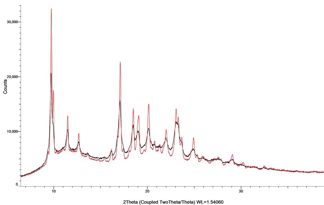
Figure S10: XRPD patterns of candesartan cilexetil with PVP K25 in co-milled mixtures (black) and physical mixtures (red).
