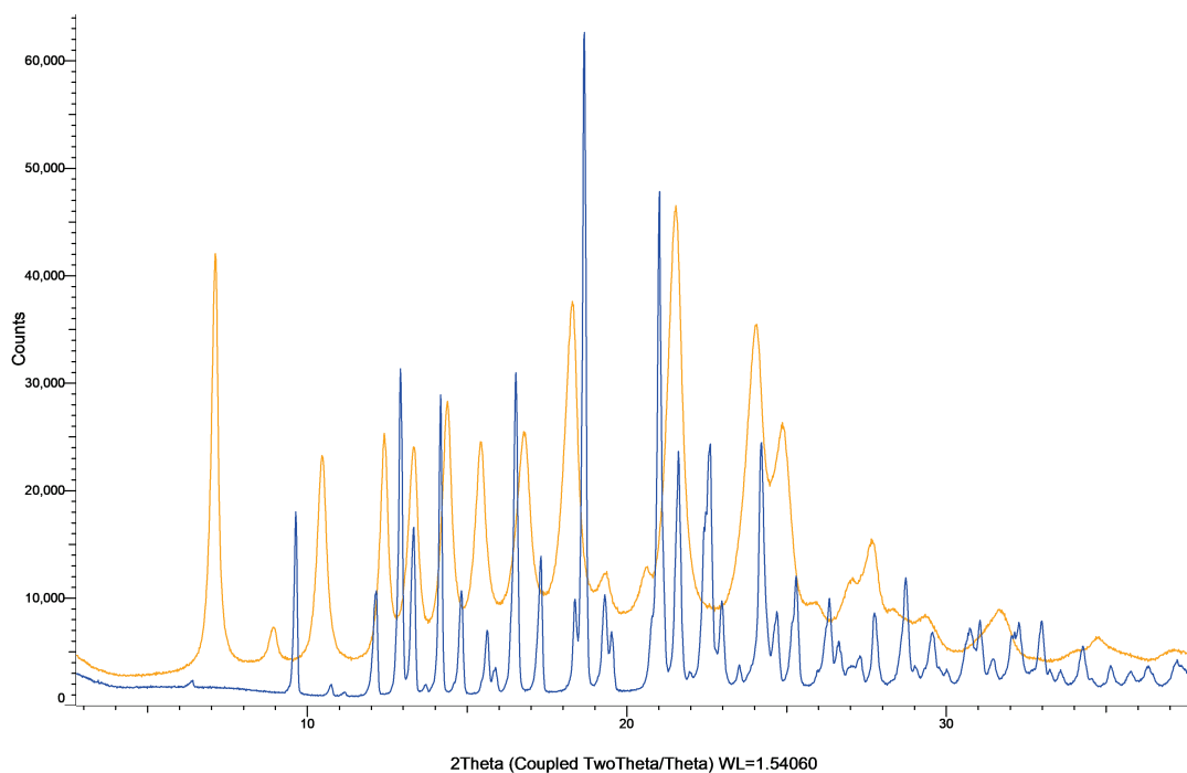
Figure S46: XRPD patterns of enzalutamide powder (blue) and milled enzalutamide powder (orange).
