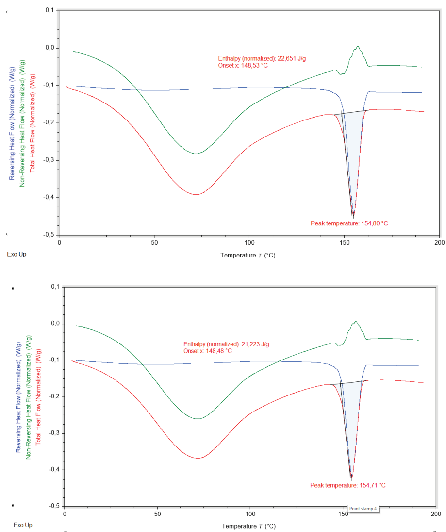
Figure S74: Thermograms illustrating the thermal behavior of apremilast co-milled with croscarmellose sodium at a 1:2 (w/w) ratio after 10 min of co-milling, measured after 3 months of storage.
