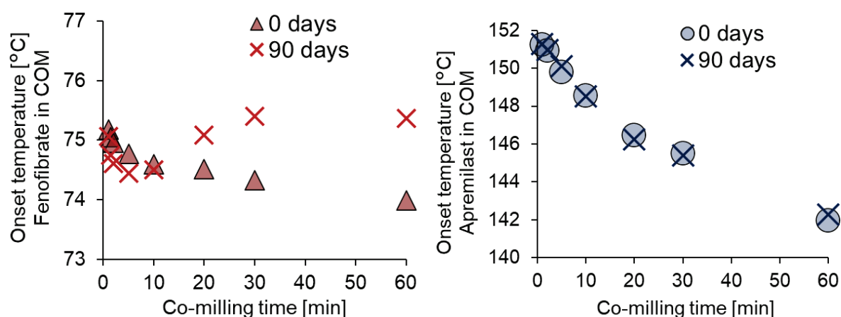
Figure 3-8: Stability study of co-milled drugs using the melting point depression approach. Depicted are onset temperatures of co-milled drugs directly after preparation and after 90 days of storage under closed conditions, 20°C and 40% relative humidity.
