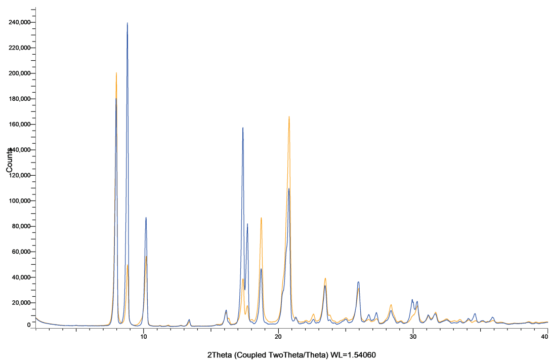
Figure S45: XRPD patterns of dipyridamole powder (blue) and milled dipyridamole powder (orange).
