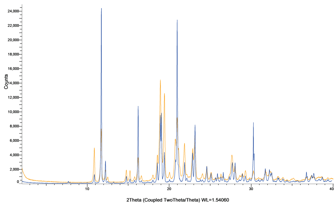
Figure S51: XRPD patterns of glibenclamide powder (blue) and milled glibenclamide powder (orange).
