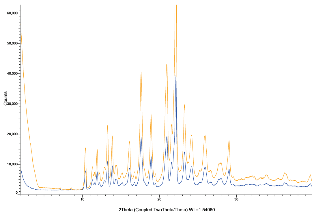
Figure S57: XRPD patterns of olaparib powder (blue) and milled olaparib powder (orange).
