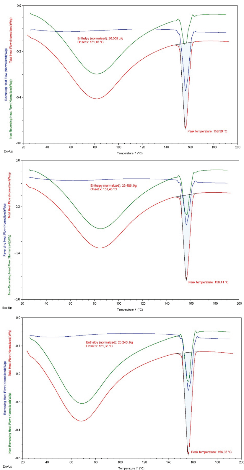
Figure S63: Thermograms illustrating the thermal behavior of apremilast co-milled with croscarmellose sodium at a 1:2 (w/w) ratio after 1 min of co-milling, measured freshly after preparation.
