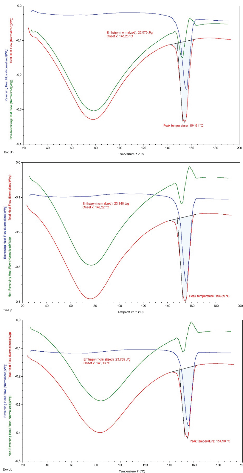
Figure S66: Thermograms illustrating the thermal behavior of apremilast co-milled with croscarmellose sodium at a 1:2 (w/w) ratio after 10 min of co-milling, measured freshly after preparation.
