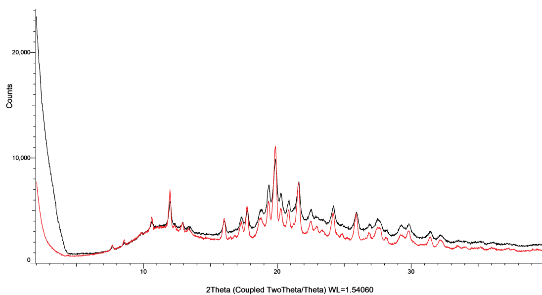
Figure S32: XRPD patterns of sorafenib with PVP K25 in co-milled mixtures (black) and physical mixtures (red).
