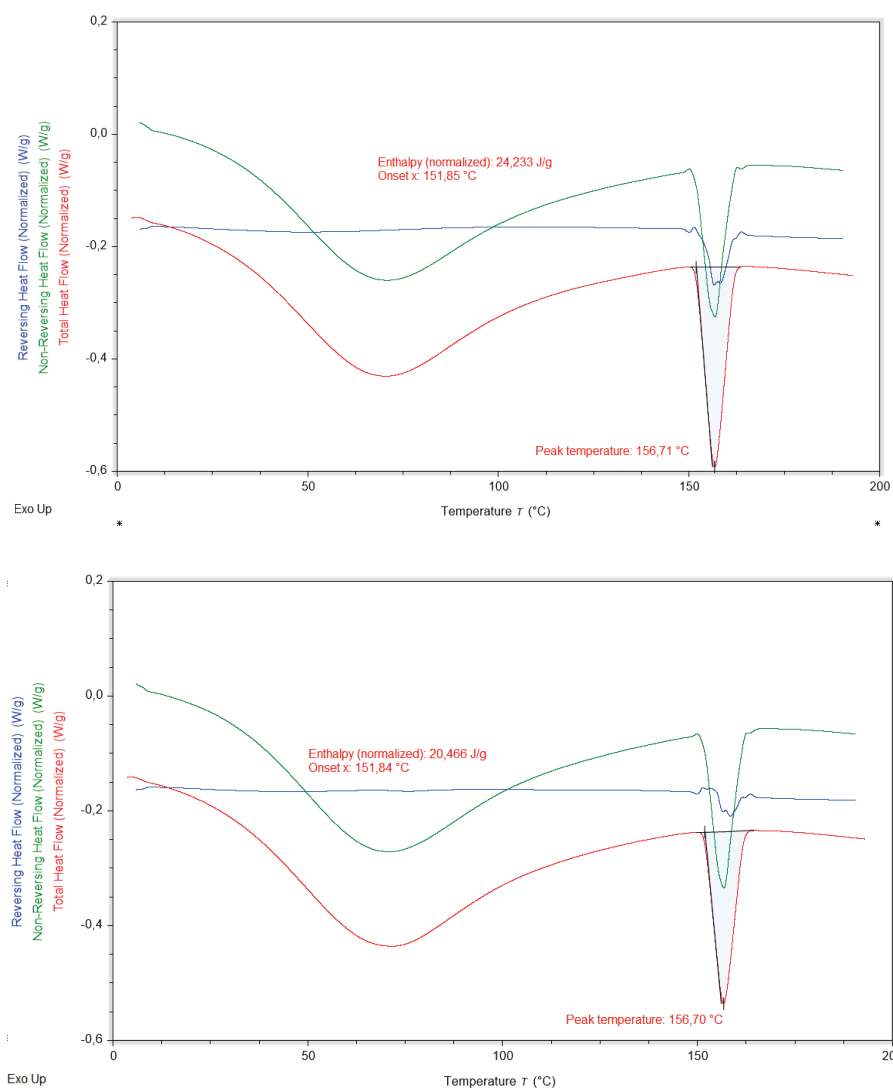
Figure S70: Thermograms illustrating the thermal behavior of apremilast blended (not milled) with croscarmellose sodium at a 1:2 (w/w), measured after 3 months of storage.
