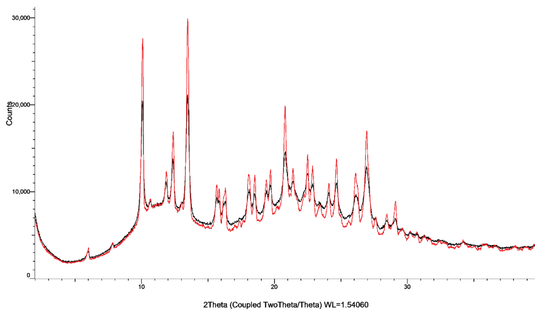
Figure S8: XRPD patterns of apremilast with PVP K25 in co-milled mixtures (black) and physical mixtures (red).
