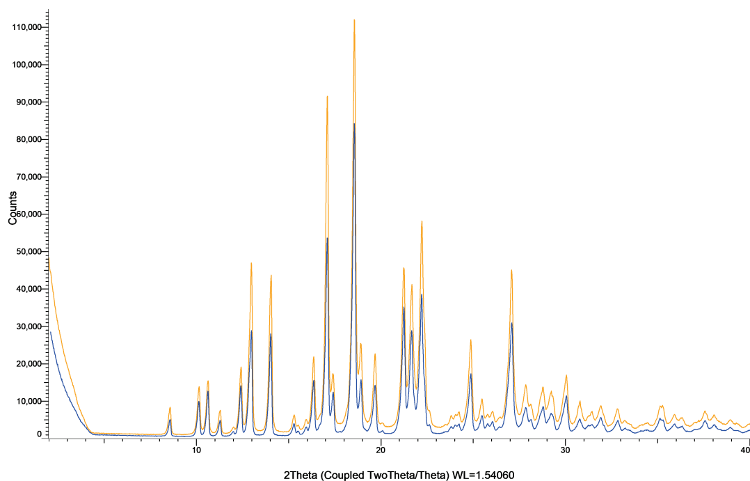
Figure S36: XRPD patterns of apixaban powder (blue) and milled apixaban powder (orange).
