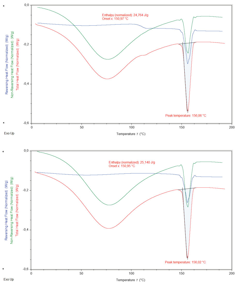
Figure S72: Thermograms illustrating the thermal behavior of apremilast co-milled with croscarmellose sodium at a 1:2 (w/w) ratio after 2 min of co-milling, measured after 3 months of storage.
