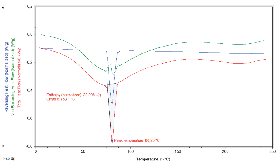
Figure S6601: Thermograms illustrating the thermal behavior of fenofibrate co-milled with croscarmellose sodium at a 1:2 (w/w) ratio after 60 min of co-milling, measured after 3 months of storage.
