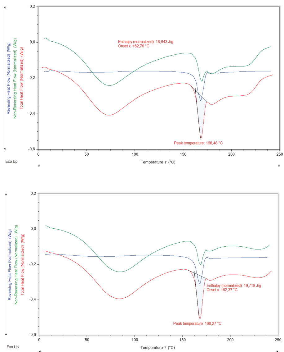
Figure S98: Thermograms illustrating the thermal behavior of fenofibrate co-milled with croscarmellose sodium at a 1:2 (w/w) ratio after 15 min of co-milling, measured after 3 months of storage.
