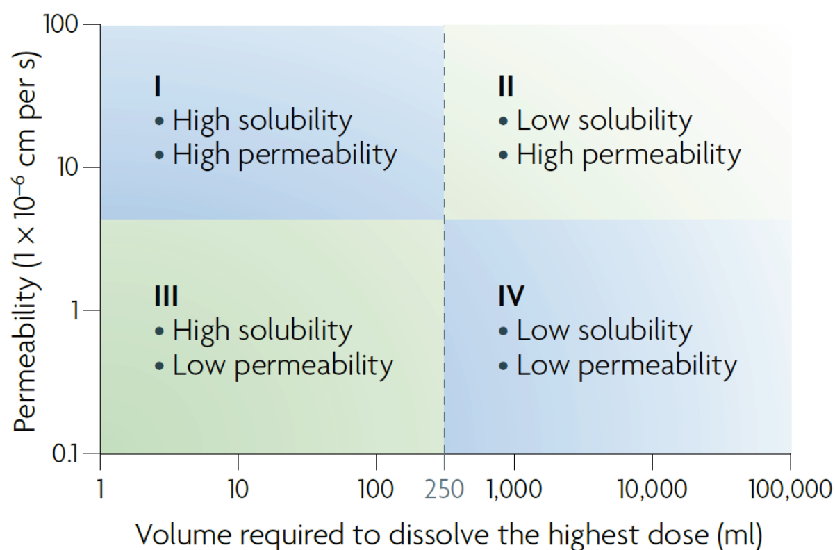
Figure 1-1: The Biopharmaceutics Classification System as proposed from (Amidon et al., 1995), adapted from (Rautio et al., 2008). Drugs are classified according to the lowest volume to dissolve the highest dose over the pH range from 1 – 7.5 (x-axis). Hence, for drugs with pH-dependent solubility, classification is based on the lowest solubility observed across the pH range (worst-case scenario). The permeability can be assessed by either in vitro assays as depicted on the y-axis or by in vivo bioavailability determination.
