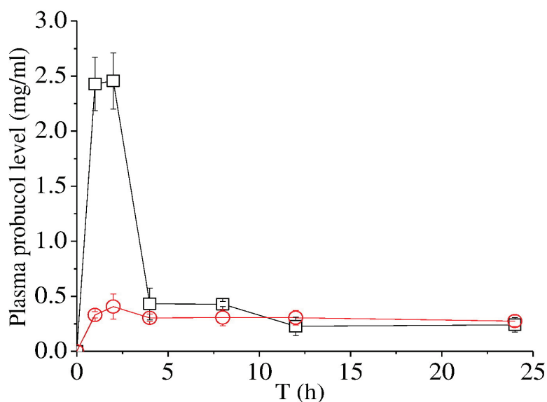
Figure 1-7: Example of a mechanically activated formulation that successfully enhanced the in vivo bioavailability of a poorly water-soluble drug. Depicted are plasma concentrations of orally administered probucol in rats ( n = 6 ), extracted from (Li et al., 2017). The black squares represent the dry milled ternary complex of probucol with the hydrophilic polymer Kollidon® VA64 and the non-ionic surfactant Cremophor® RH40, while the red cycles show the plasma concentration of the marketed formulation.
