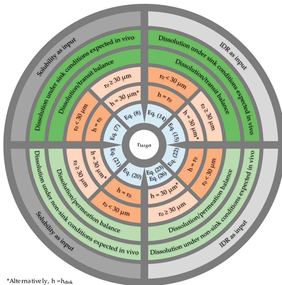
Figure 1-2: The “decision wheel” for the calculation of the target particle radius to overcome dissolution rate limited absorption, extracted from (Beran et al., 2023). The decision process begins with either solubility or intrinsic dissolution rate (IDR) as input (outer ring), followed by an assessment of whether sink or non-sink conditions are expected in vivo.
