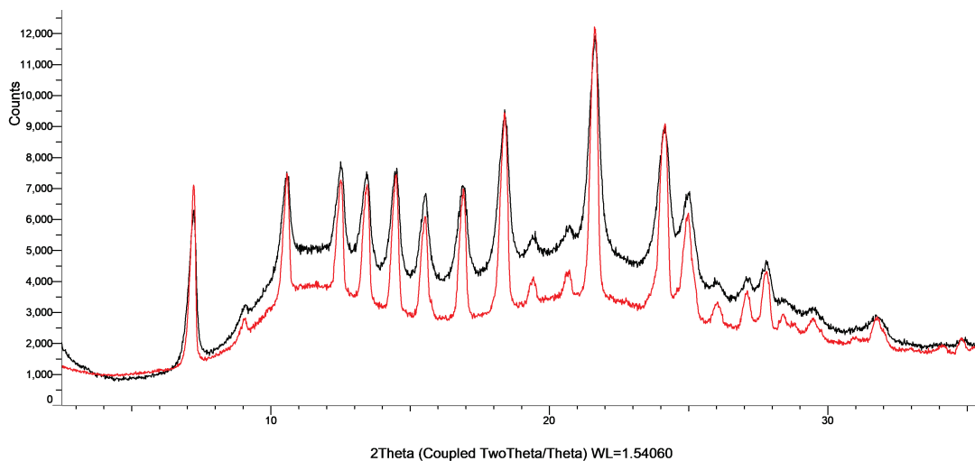
Figure S33: XRPD patterns of tadalafil with PVP K25 in co-milled mixtures (black) and physical mixtures (red).
