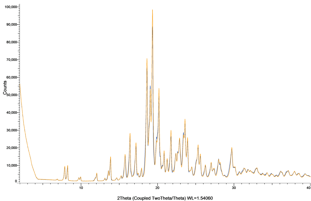
Figure S48: XRPD patterns of ezetimibe powder (blue) and milled ezetimibe powder (orange).
