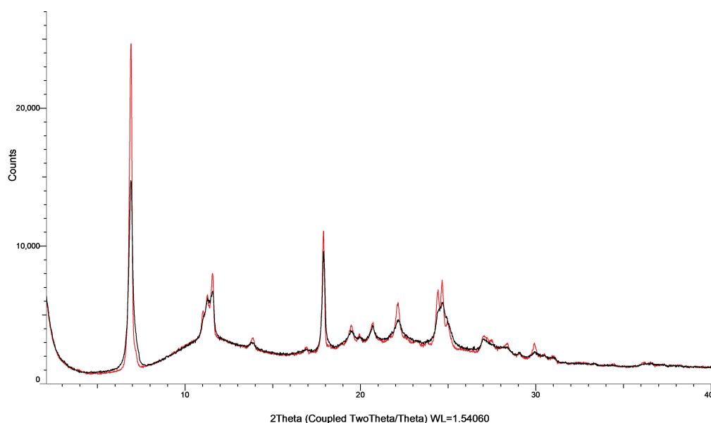
Figure S6: XRPD patterns of albendazole with PVP K25 in co-milled mixtures (black) and physical mixtures (red)
