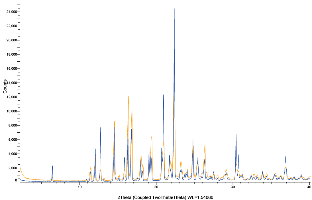
Figure S49: XRPD patterns of fenofibrate powder (blue) and milled fenofibrate powder (orange).
