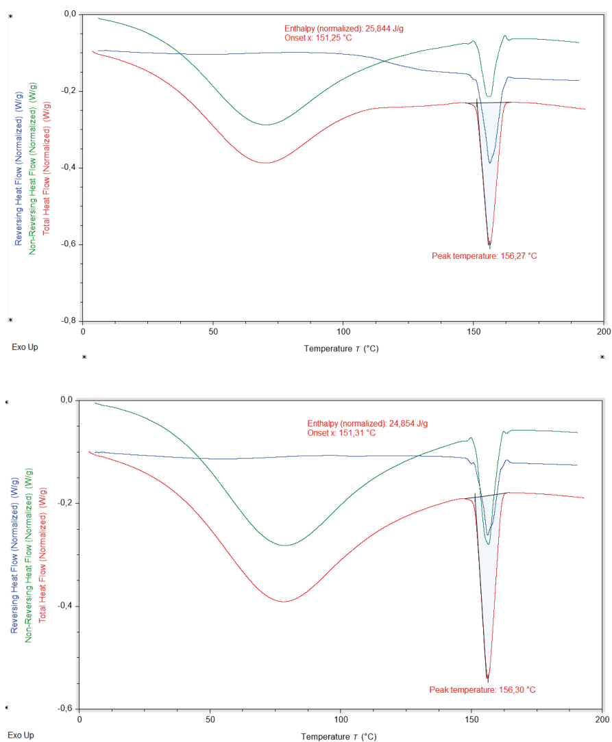
Figure S71: Thermograms illustrating the thermal behavior of apremilast co-milled with croscarmellose sodium at a 1:2 (w/w) ratio after 1 min of co-milling, measured after 3 months of storage.
