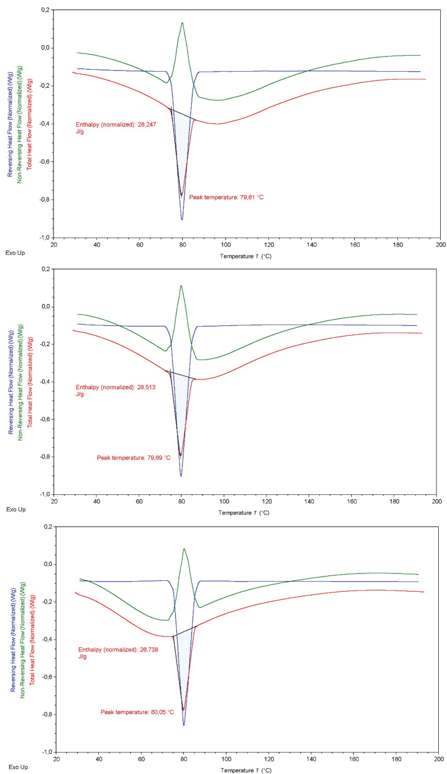
Figure S87: Thermograms illustrating the thermal behavior of fenofibrate co-milled with croscarmellose sodium at a 1:2 (w/w) ratio after 20 min of co-milling, measured freshly after preparation.
