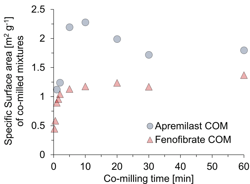
Figure S663: Relationship between Co-milling time and the specific surface area of co-milled mixtures.
