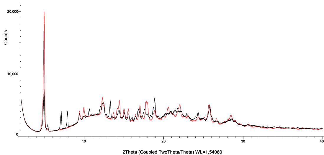
Figure S13: XRPD patterns of ceritinib with PVP K25 in co-milled mixtures (black) and physical mixtures (red).
