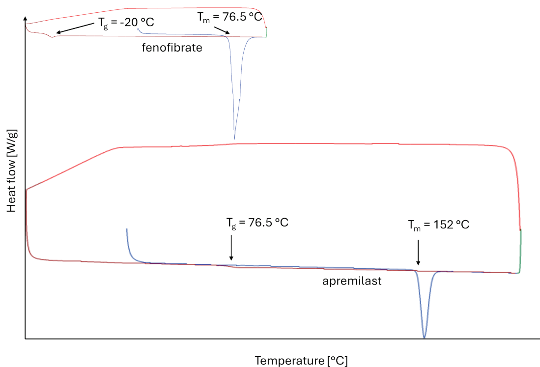
Figure 3-3: Glass forming ability class determinations of apremilast and fenofibrate. The glass transition temperatures ( T_g ) were extracted by using the midpoint of the thermal event from the quenched cooled melt and the onset of the melting peak was used to determine the melting point ( T_m ).
