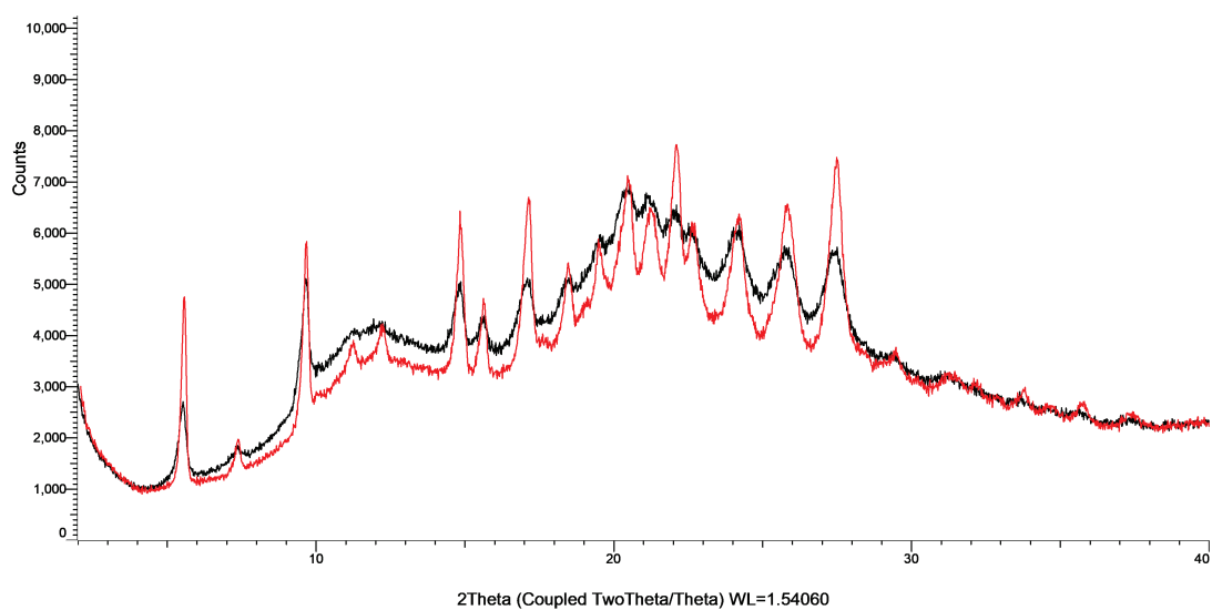
Figure S27: XRPD patterns of nilotinib with PVP K25 in co-milled mixtures (black) and physical mixtures (red).
