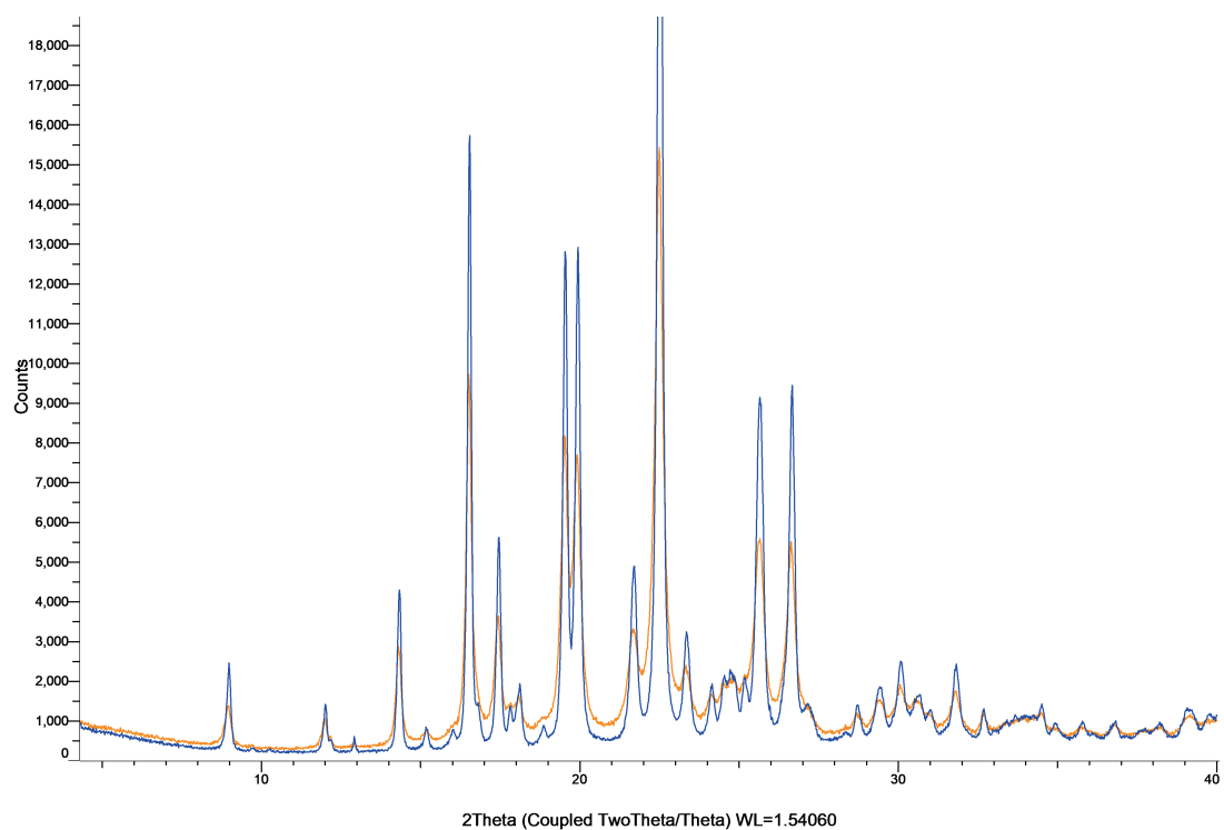
Figure S58: XRPD patterns of rivaroxaban powder (blue) and milled rivaroxaban powder (orange).
