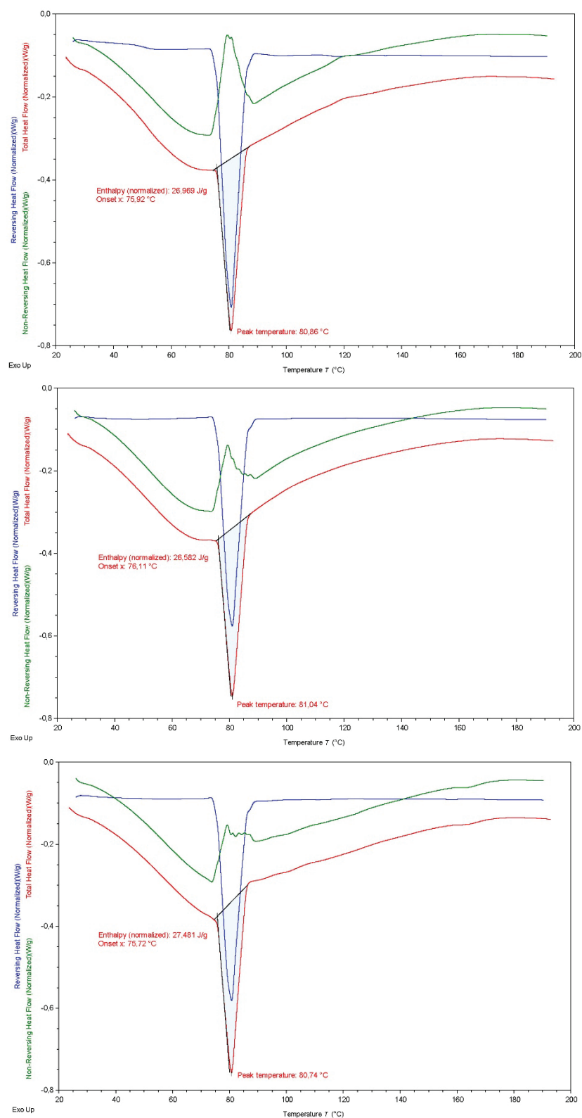
Figure S83: Thermograms illustrating the thermal behavior of fenofibratet co-milled with croscarmellose sodium at a 1:2 (w/w) ratio after 1.5 min of co-milling, measured freshly after preparation.
