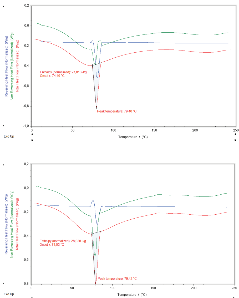
Figure S97: Thermograms illustrating the thermal behavior of fenofibrate co-milled with croscarmellose sodium at a 1:2 (w/w) ratio after 10 min of co-milling, measured after 3 months of storage.
