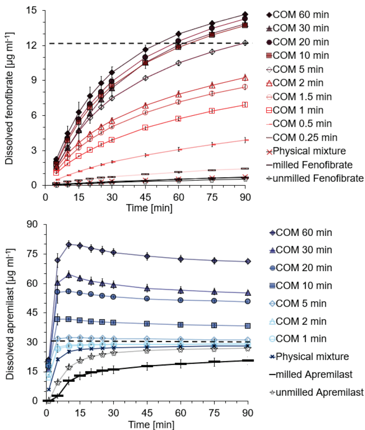
Figure 3-4: Dissolution profiles of fenofibrate and apremilast as unmilled drugs, milled drugs, physically blended and co-milled mixtures (COM) at different milling times with croscarmellose sodium in a drug to excipient ratio of 1:2 (w/w) ( n = 4 ). The black dotted line expresses the equilibrium solubility of the respective drugs in the used medium FaSSIF V1 at 37°C.
