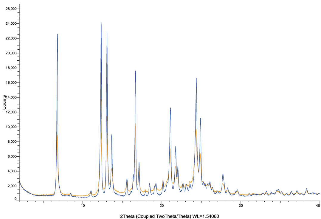
Figure S39: XRPD patterns of dasatinib powder (blue) and milled dasatinib powder (orange).
