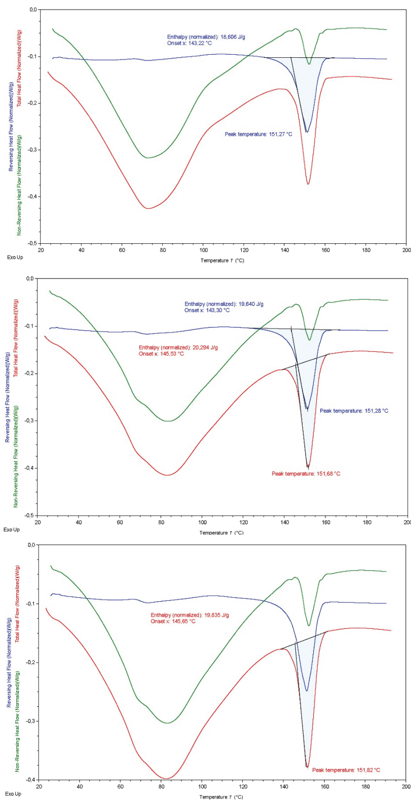
Figure S68: Thermograms illustrating the thermal behavior of apremilast co-milled with croscarmellose sodium at a 1:2 (w/w) ratio after 30 min of co-milling, measured freshly after preparation.
