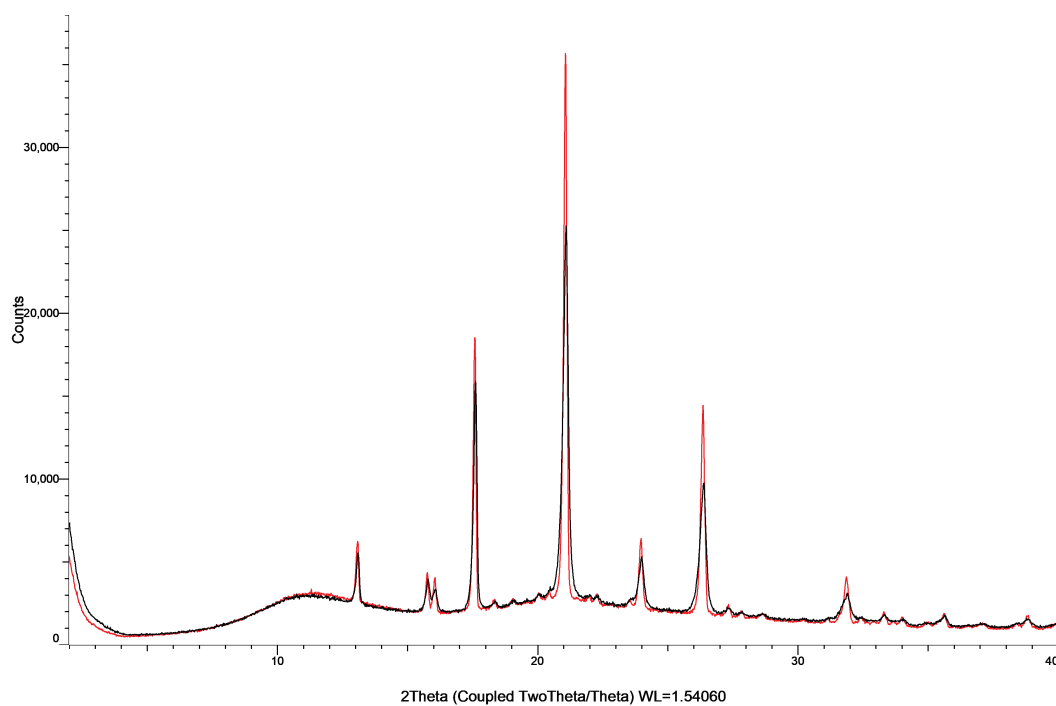
Figure S34: XRPD patterns of thiabendazole with PVP K25 in co-milled mixtures (black) and physical mixtures (red).
