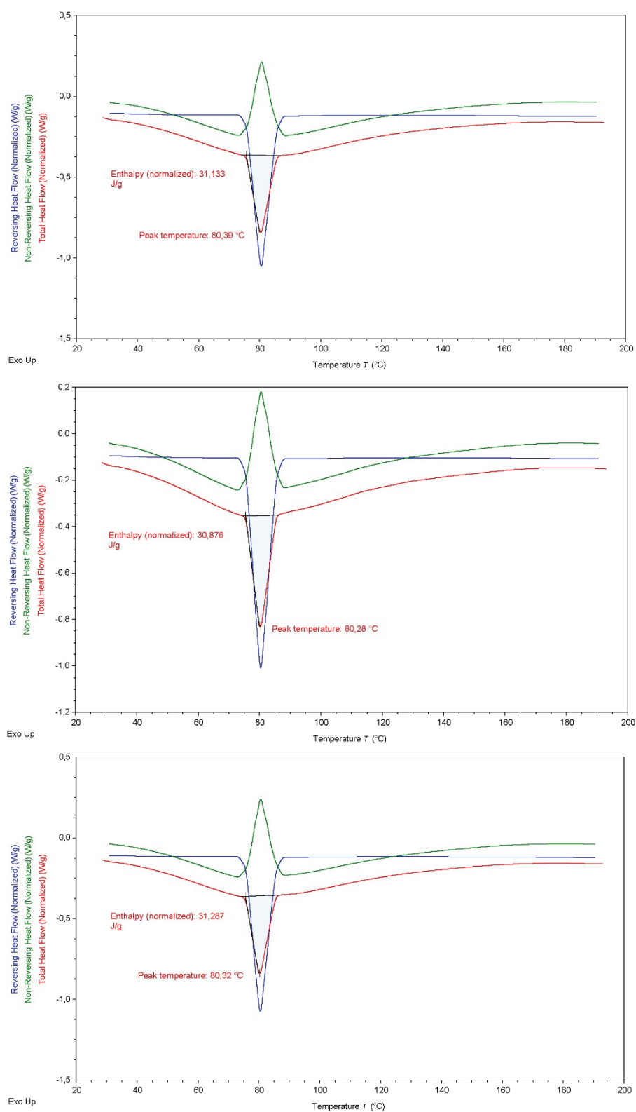
Figure S80: Thermograms illustrating the thermal behavior of fenofibrate co-milled with croscarmellose sodium at a 1:2 (w/w) ratio after 30 s of co-milling, measured freshly after preparation.
