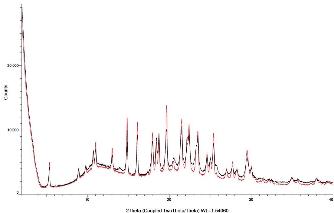
Figure S12: XRPD patterns of celecoxib with PVP K25 in co-milled mixtures (black) and physical mixtures (red).
