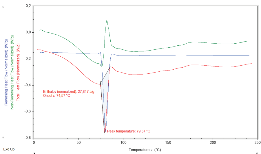
Figure S95: Thermograms illustrating the thermal behavior of fenofibrate co-milled with croscarmellose sodium at a 1:2 (w/w) ratio after 120 s of co-milling, measured after 3 months of storage.
