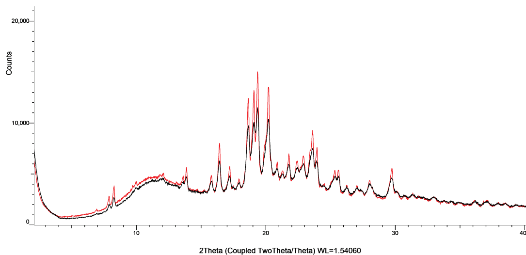
Figure S20: XRPD patterns of ezetimibe with PVP K25 in co-milled mixtures (black) and physical mixtures (red).
