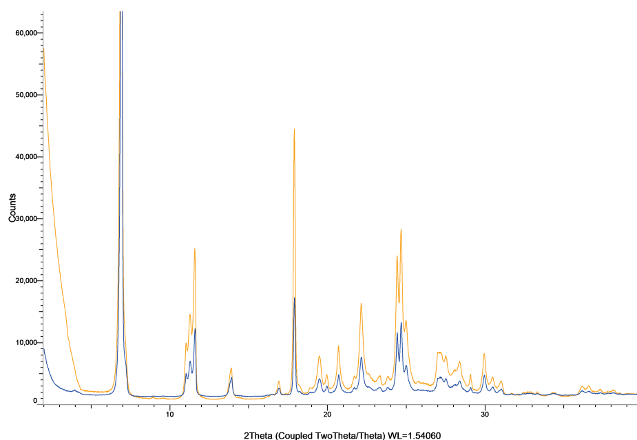
Figure S35: XRPD patterns of albendazole powder (blue) and milled albendazole powder (orange).
