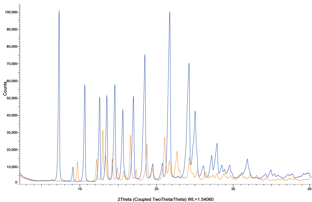
Figure S61: XRPD patterns of tadalafil powder (blue) and milled tadalafil powder (orange).
