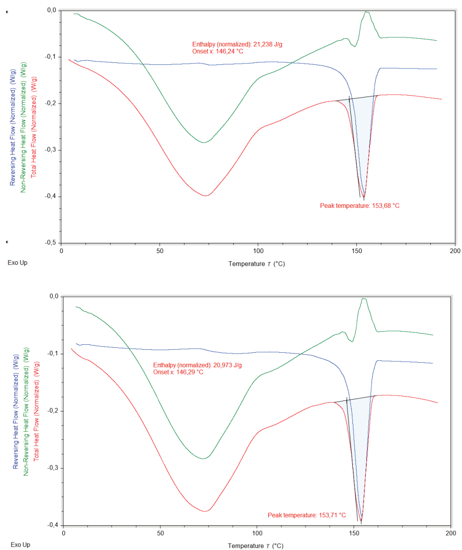
Figure S75: Thermograms illustrating the thermal behavior of apremilast co-milled with croscarmellose sodium at a 1:2 (w/w) ratio after 20 min of co-milling, measured after 3 months of storage.
