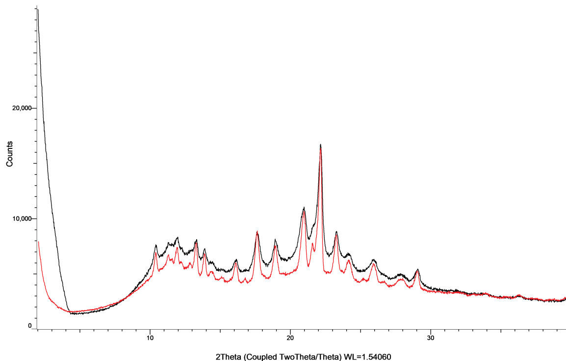
Figure S29: XRPD patterns of olaparib with PVP K25 in co-milled mixtures (black) and physical mixtures (red).
