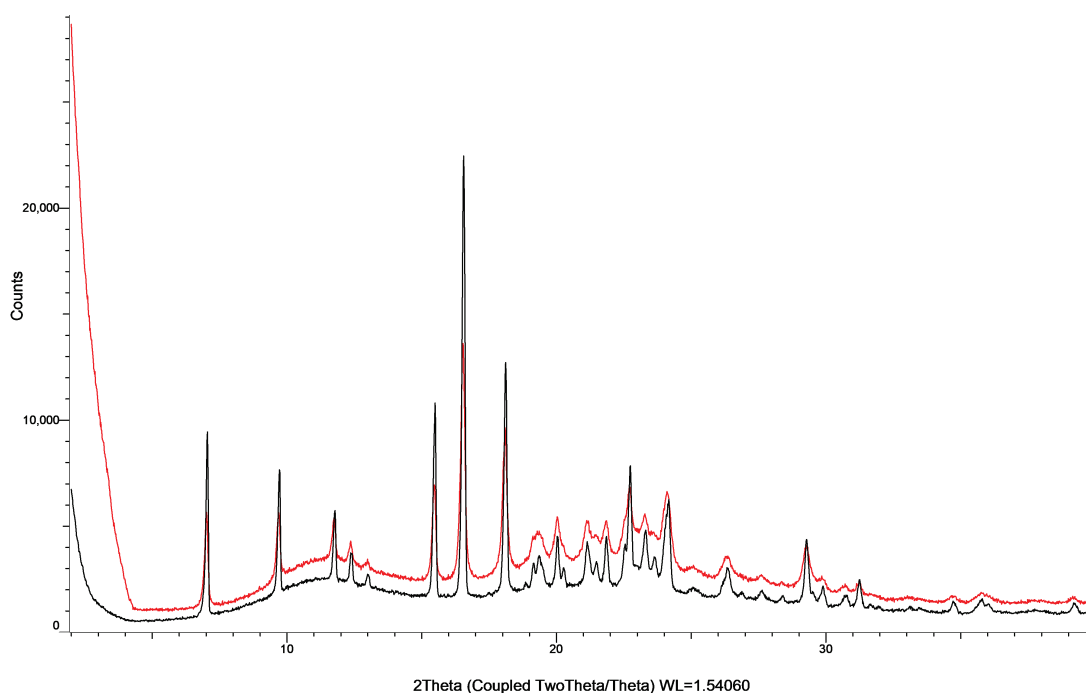
Figure S19: XRPD patterns of etoricoxib with PVP K25 in co-milled mixtures (black) and physical mixtures (red).
