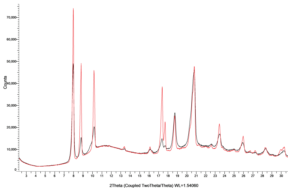
Figure S17: XRPD patterns of dipyridamole with PVP K25 in co-milled mixtures (black) and physical mixtures (red).
