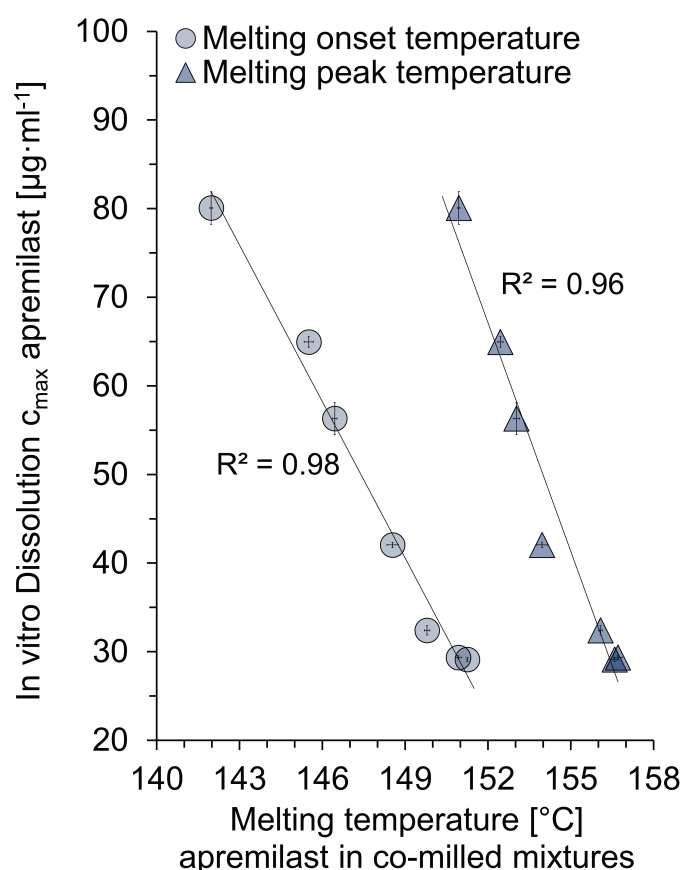
Figure 3-7: The melting point depression of the high- T_g glass former apremilast as a function of the highest measured apremilast concentration ( c_{\max} ) during the in vitro dissolution process. Apremilast was co-milled with croscarmellose sodium at different milling times from 1 to 60 min ( n = 3 ).
