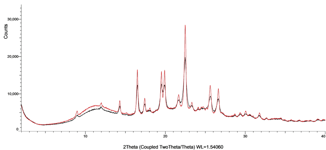
Figure S30: XRPD patterns of rivaroxaban with PVP K25 in co-milled mixtures (black) and physical mixtures (red).
