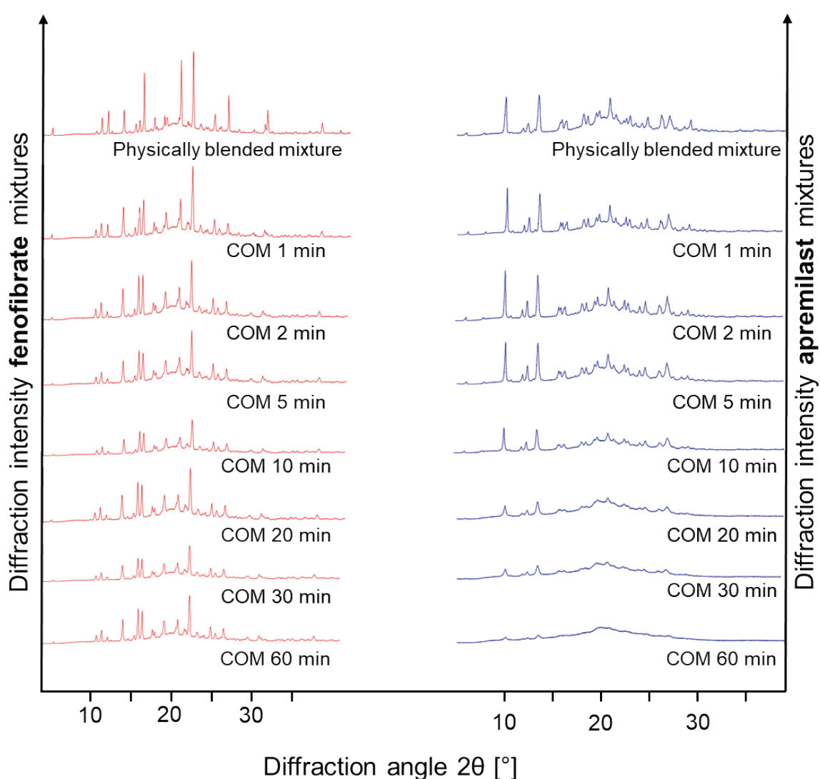
Figure 3-2: X-ray powder diffractograms of fenofibrate (red) and apremilast (blue) in physically blended mixtures and co-milled mixtures (COM) at different milling times.
