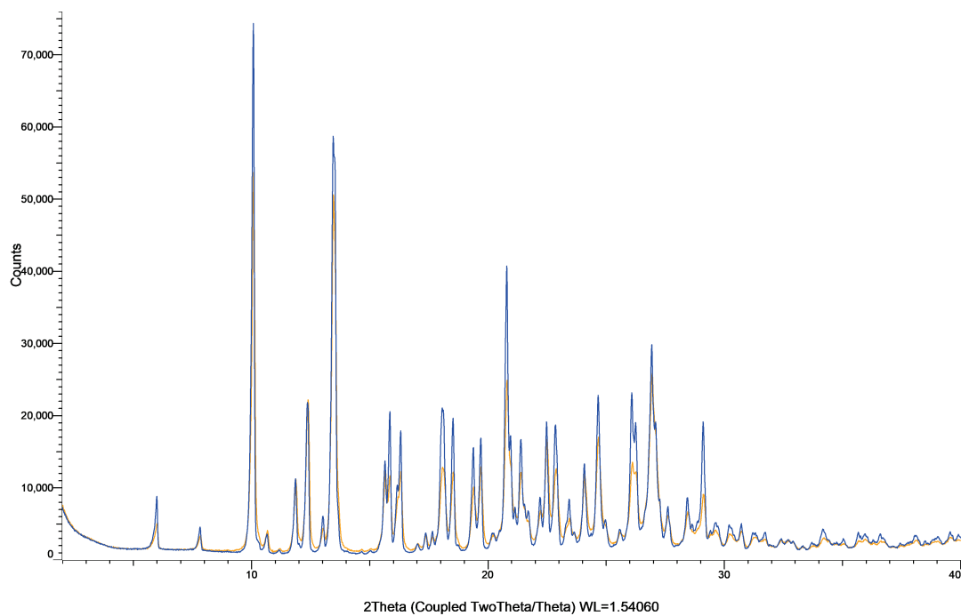
Figure S37: XRPD patterns of apremilast powder (blue) and milled apremilast powder (orange).
