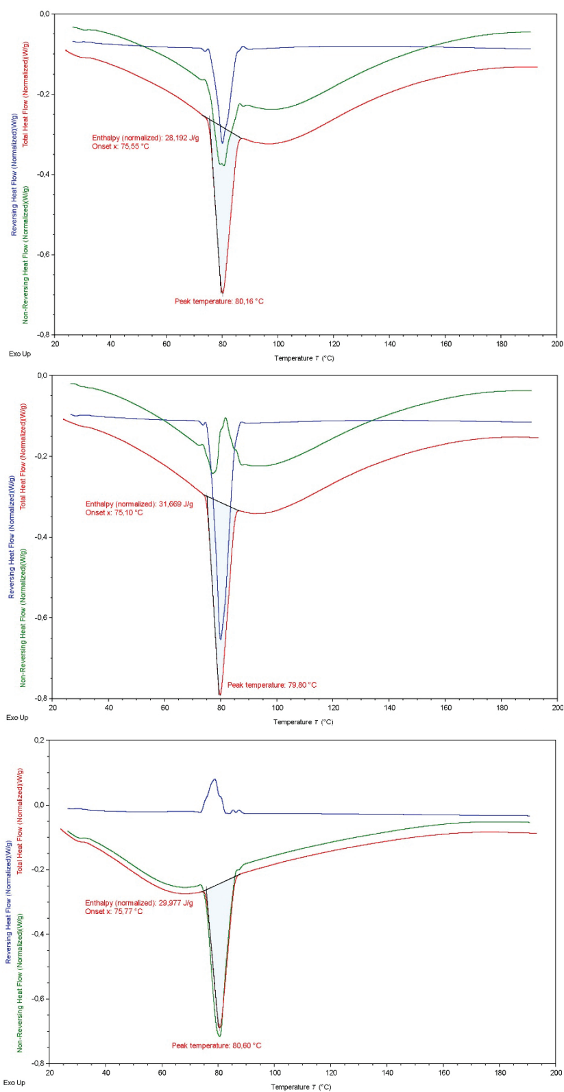
Figure S78: Thermograms illustrating the thermal behavior of fenofibrate blended (not milled) with croscarmellose sodium at a 1:2 (w/w), measured freshly after blending.
