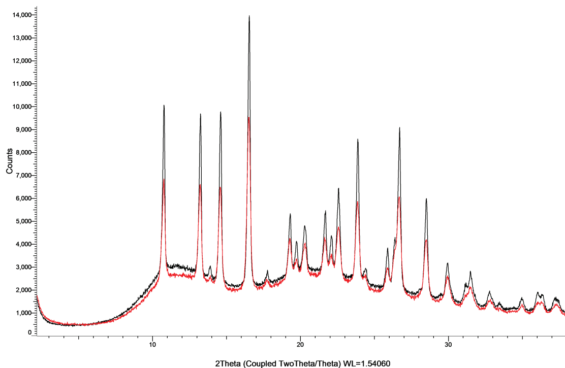
Figure S24: XRPD patterns of griseofulvin with PVP K25 in co-milled mixtures (black) and physical mixtures (red).
