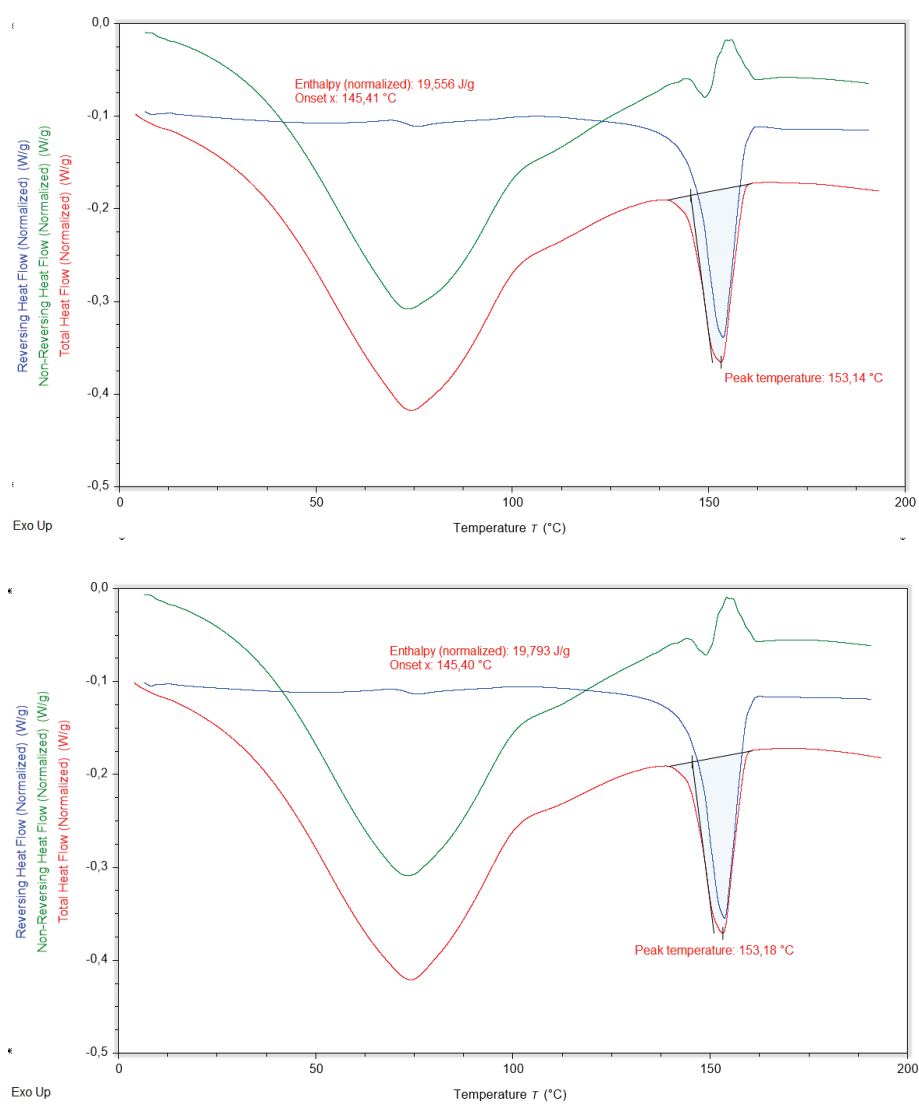
Figure S76: Thermograms illustrating the thermal behavior of apremilast co-milled with croscarmellose sodium at a 1:2 (w/w) ratio after 30 min of co-milling, measured after 3 months of storage.
