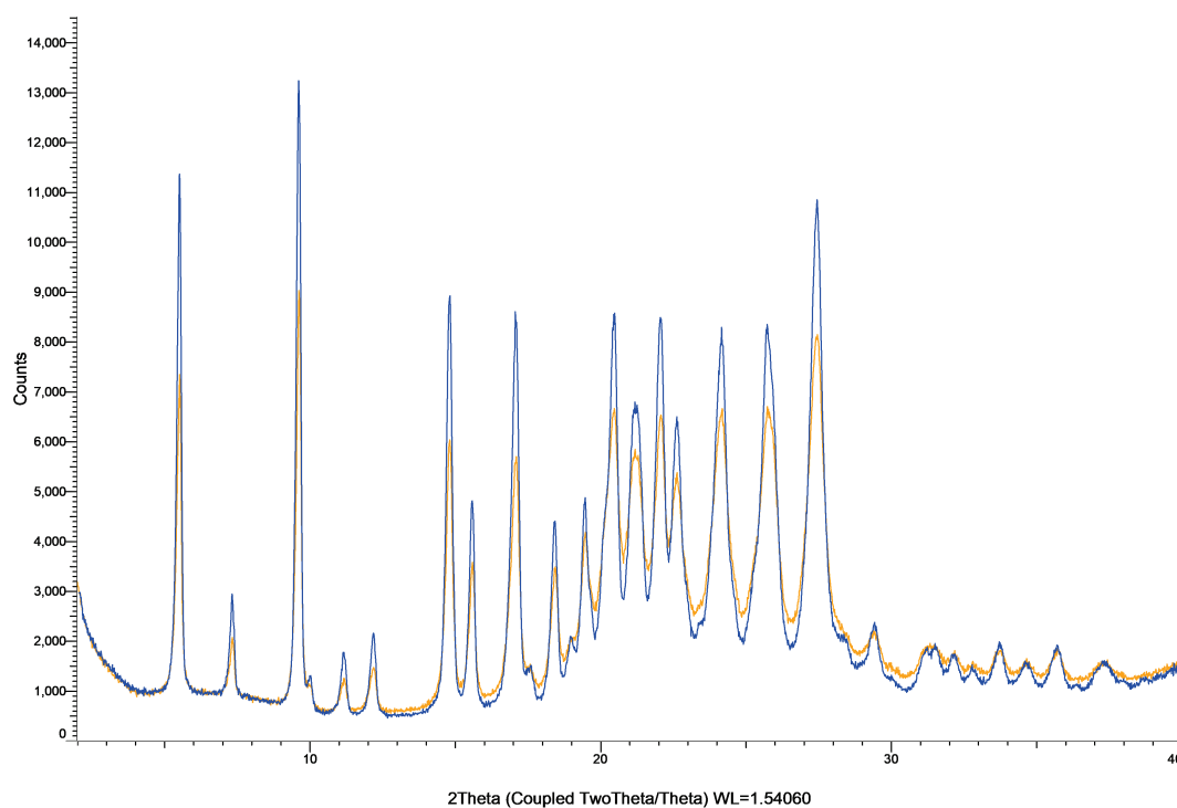
Figure S55: XRPD patterns of nilotinib powder (blue) and milled nilotinib powder (orange).
