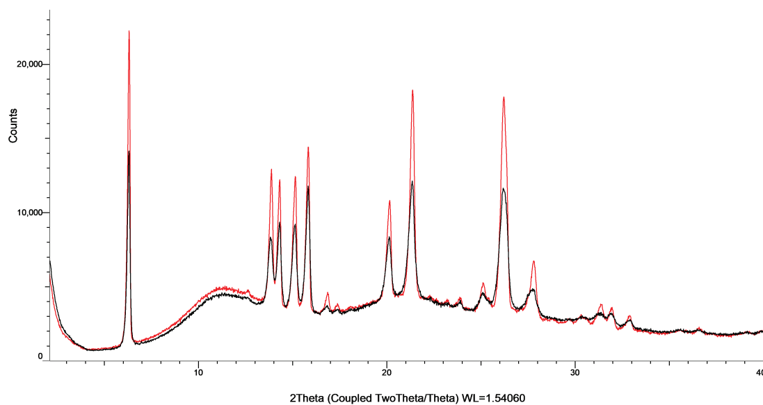
Figure S26: XRPD patterns of mefenamic acid with PVP K25 in co-milled mixtures (black) and physical mixtures (red).
