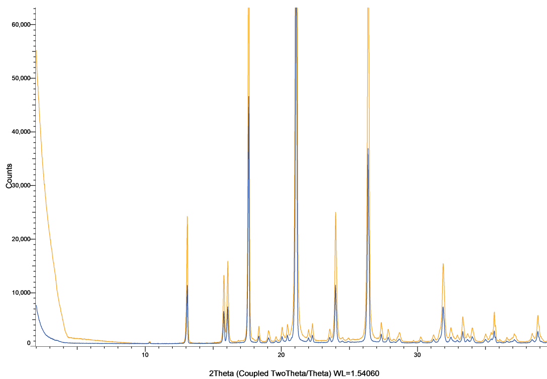
Figure S62: XRPD patterns of thiabendazole powder (blue) and milled thiabendazole powder (orange).
