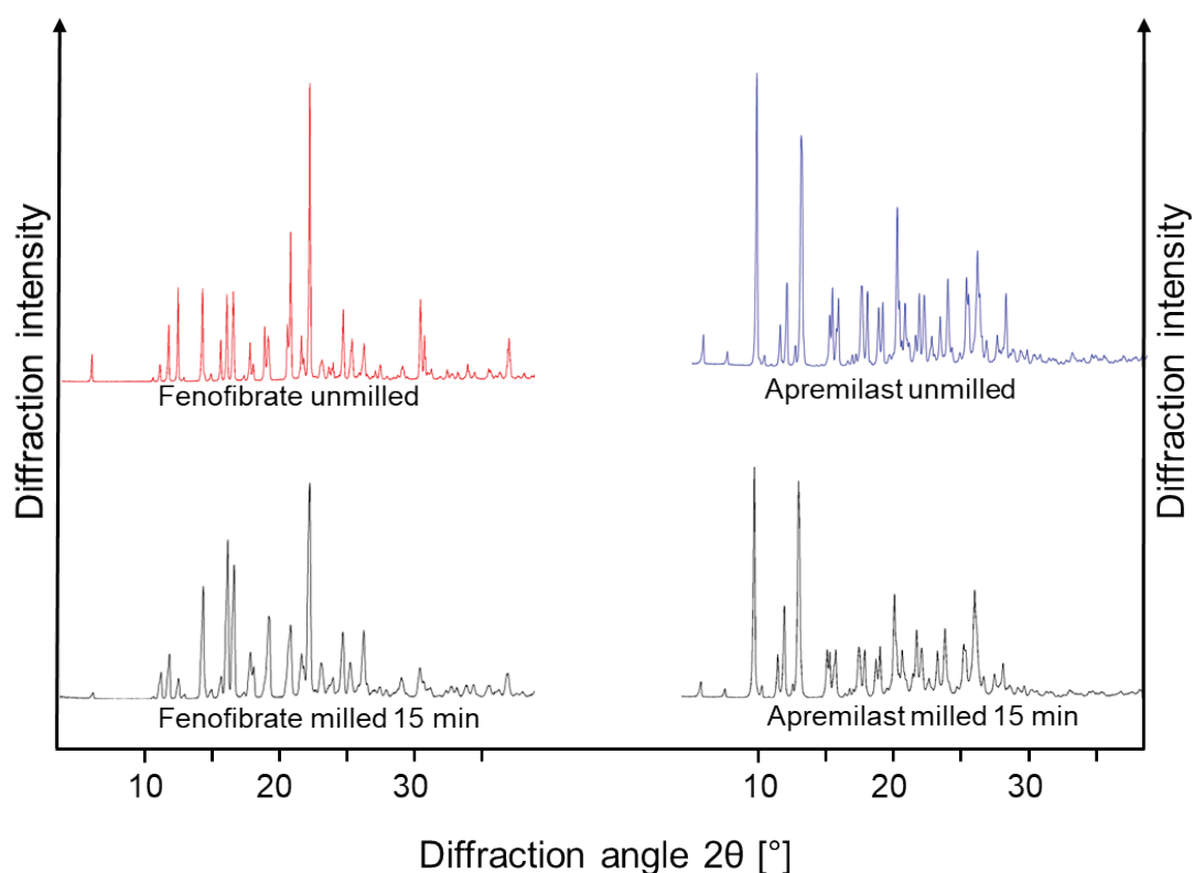
Figure 3-1: X-ray powder diffractograms of fenofibrate (left, red) and apremilast (right, blue) as unground drug powder and both drugs after 15 min ball milling (black).
