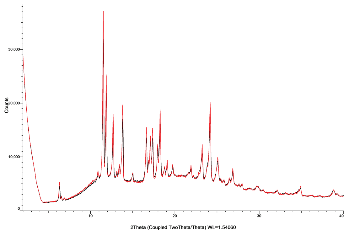
Figure S22: XRPD patterns of gemfibrozil with PVP K25 in co-milled mixtures (black) and physical mixtures (red).
