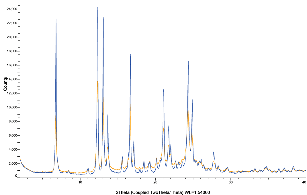
Figure S44: XRPD patterns of deferasirox powder (blue) and milled deferasirox powder (orange).
