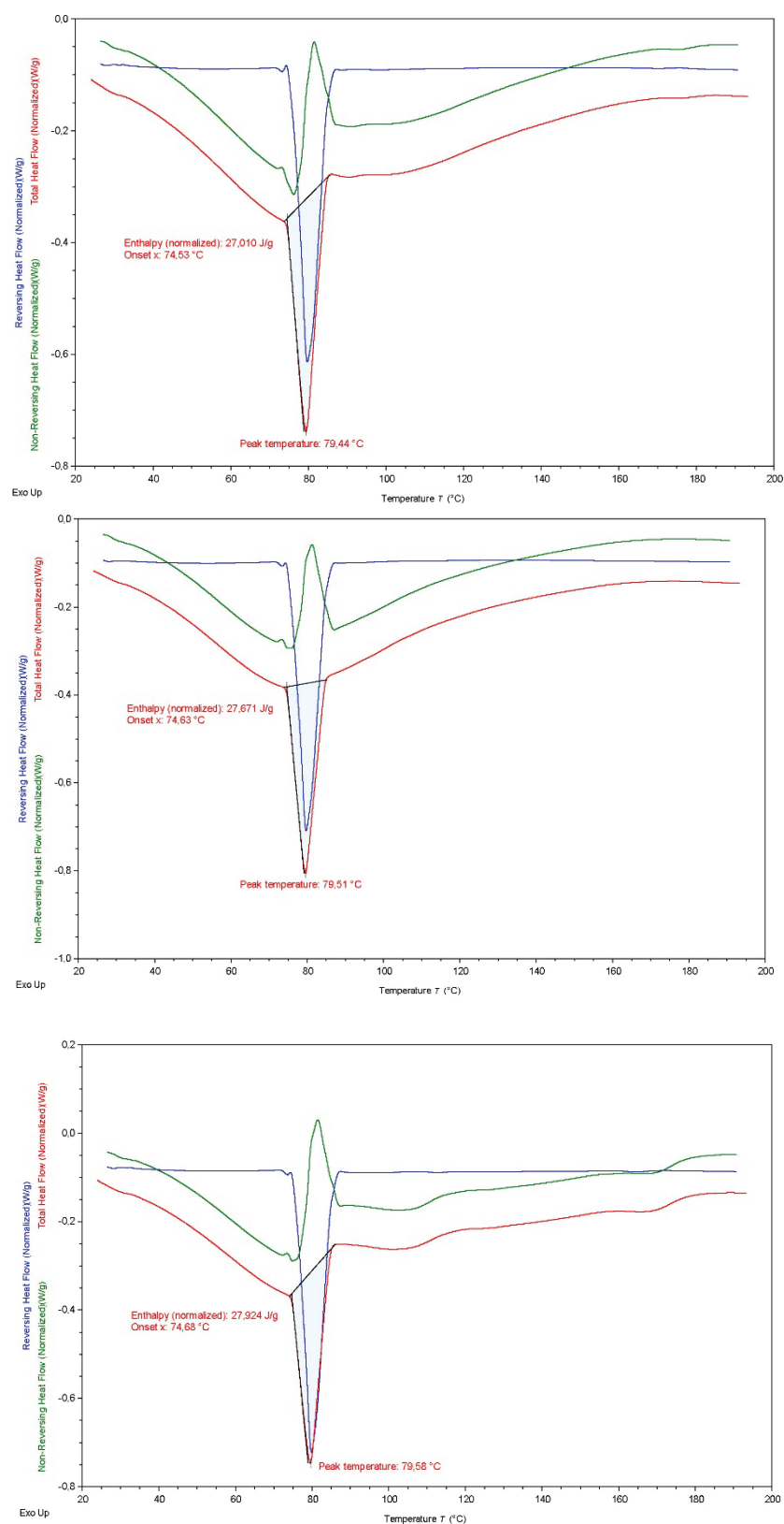
Figure S84: Thermograms illustrating the thermal behavior of fenofibrate co-milled with croscarmellose sodium at a 1:2 (w/w) ratio after 2 min of co-milling, measured freshly after preparation.
