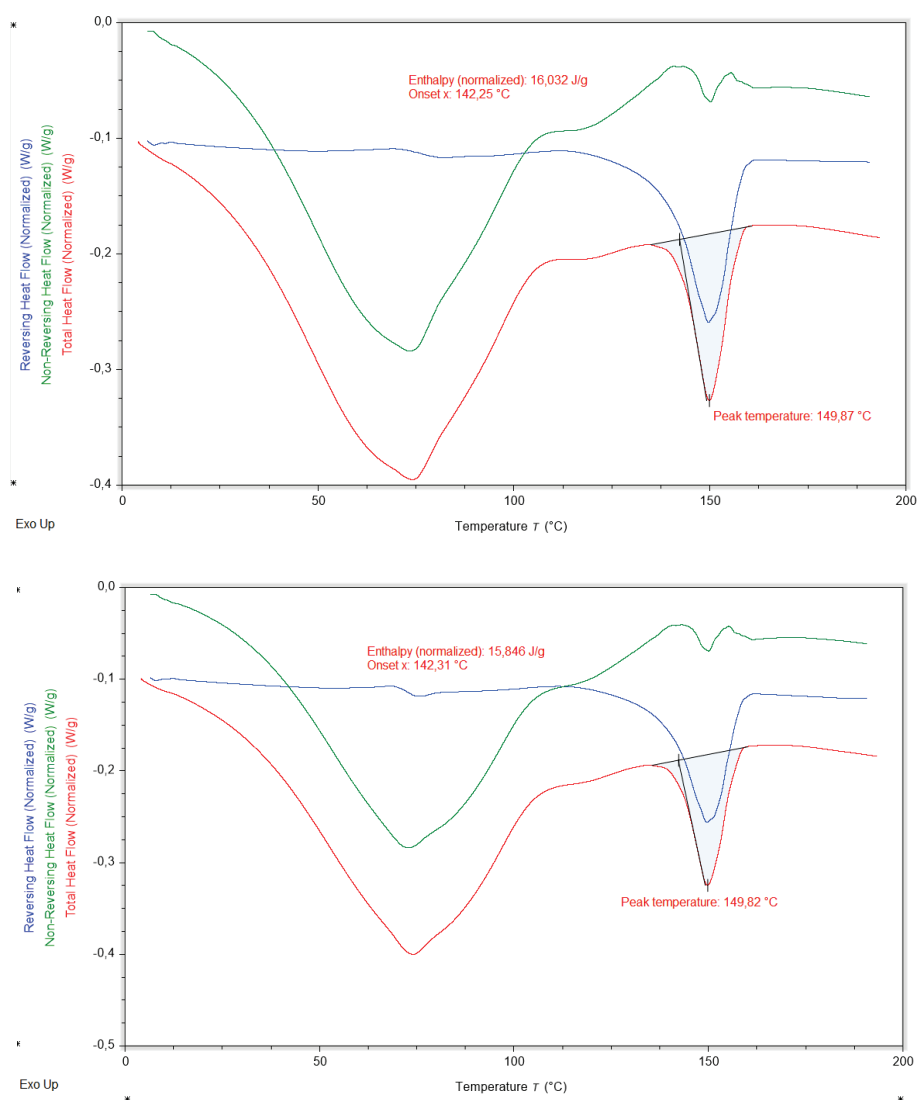
Figure S77: Thermograms illustrating the thermal behavior of apremilast co-milled with croscarmellose sodium at a 1:2 (w/w) ratio after 60 min of co-milling, measured after 3 months of storage.
