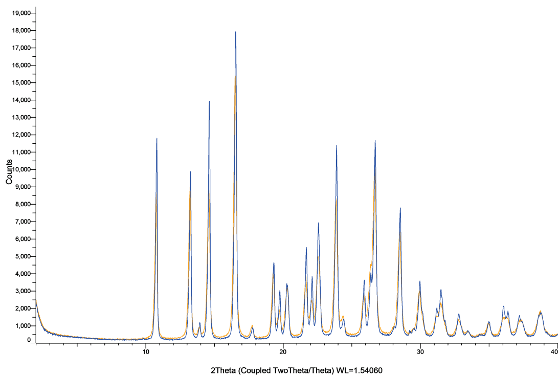
Figure S52: XRPD patterns of griseofulvin powder (blue) and milled griseofulvin powder (orange).
