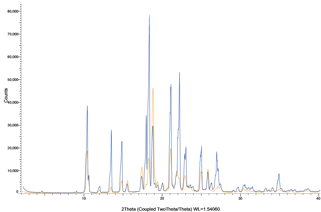
Figure S43: XRPD patterns of cinnarizine powder (blue) and milled cinnarizine powder (orange).
