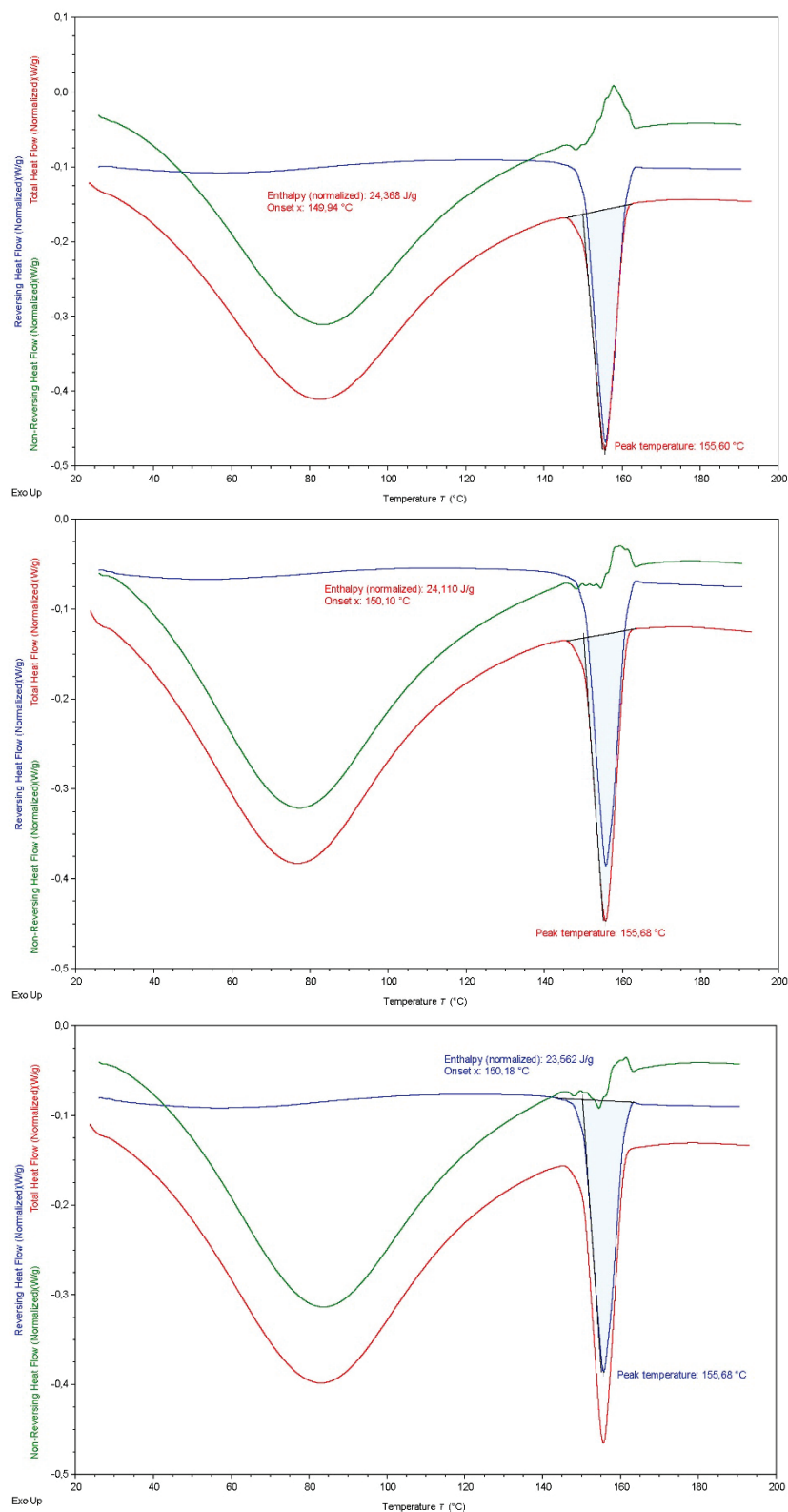
Figure S65: Thermograms illustrating the thermal behavior of apremilast co-milled with croscarmellose sodium at a 1:2 (w/w) ratio after 5 min of co-milling, measured freshly after preparation.
