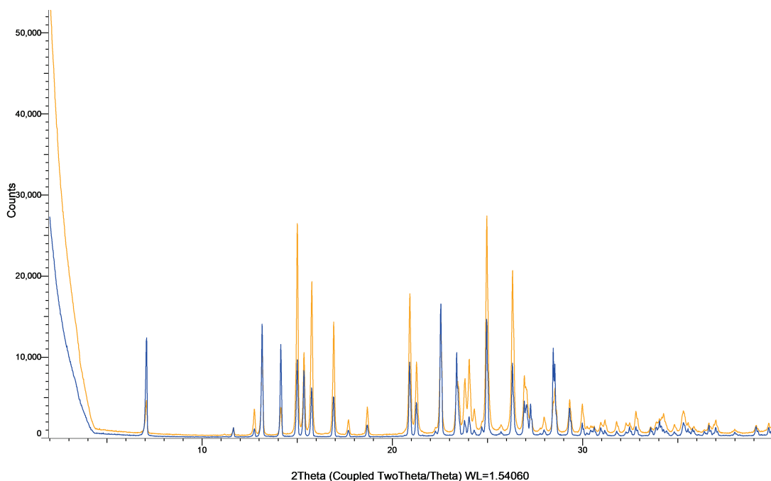
Figure S59: XRPD patterns of sertraline powder (blue) and milled sertraline powder (orange).
