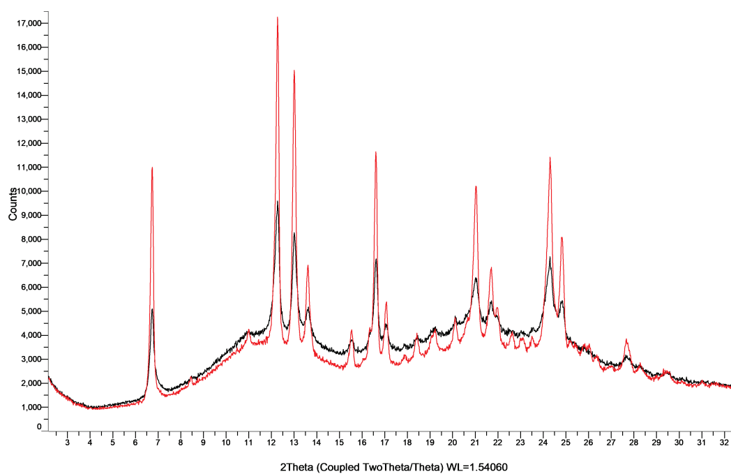
Figure S15: XRPD patterns of dasatinib with PVP K25 in co-milled mixtures (black) and physical mixtures (red).
