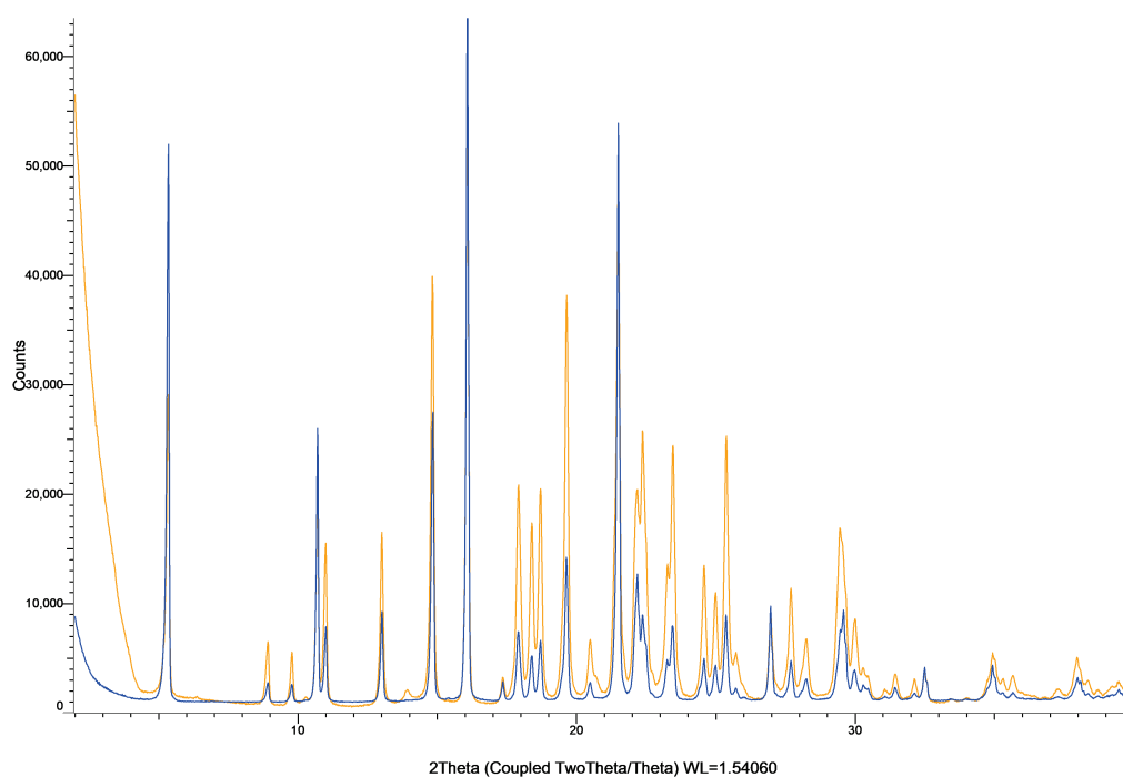
Figure S41: XRPD patterns of celecoxib powder (blue) and milled celecoxib powder (orange).
