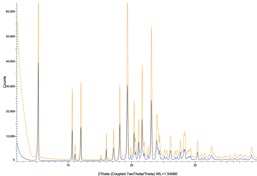
Figure S56: XRPD patterns of nimesulide powder (blue) and milled nimesulide powder (orange).
