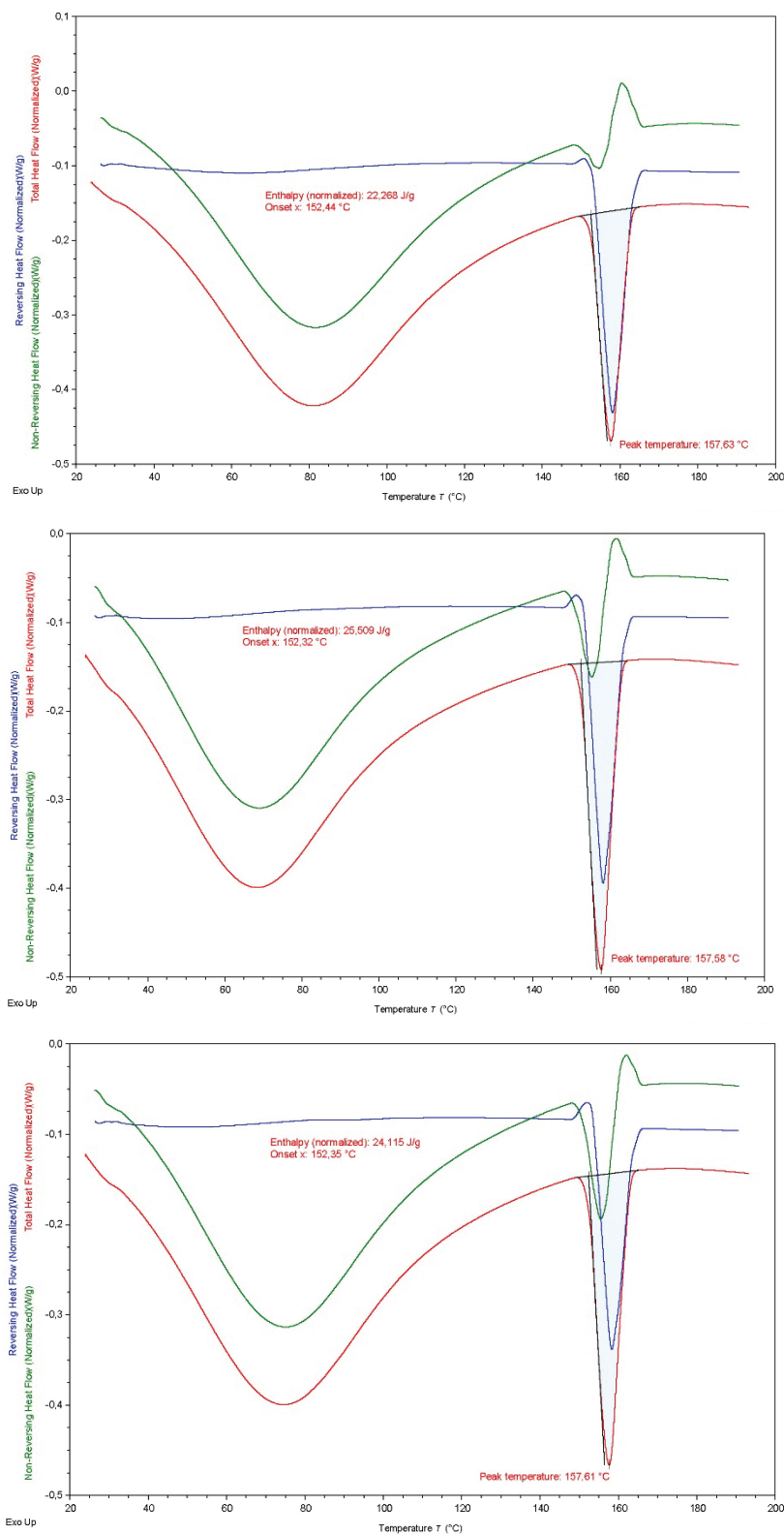
Figure S62: Thermograms illustrating the thermal behavior of apremilast blended (not milled) with croscarmellose sodium at a 1:2 (w/w), measured freshly after blending.
