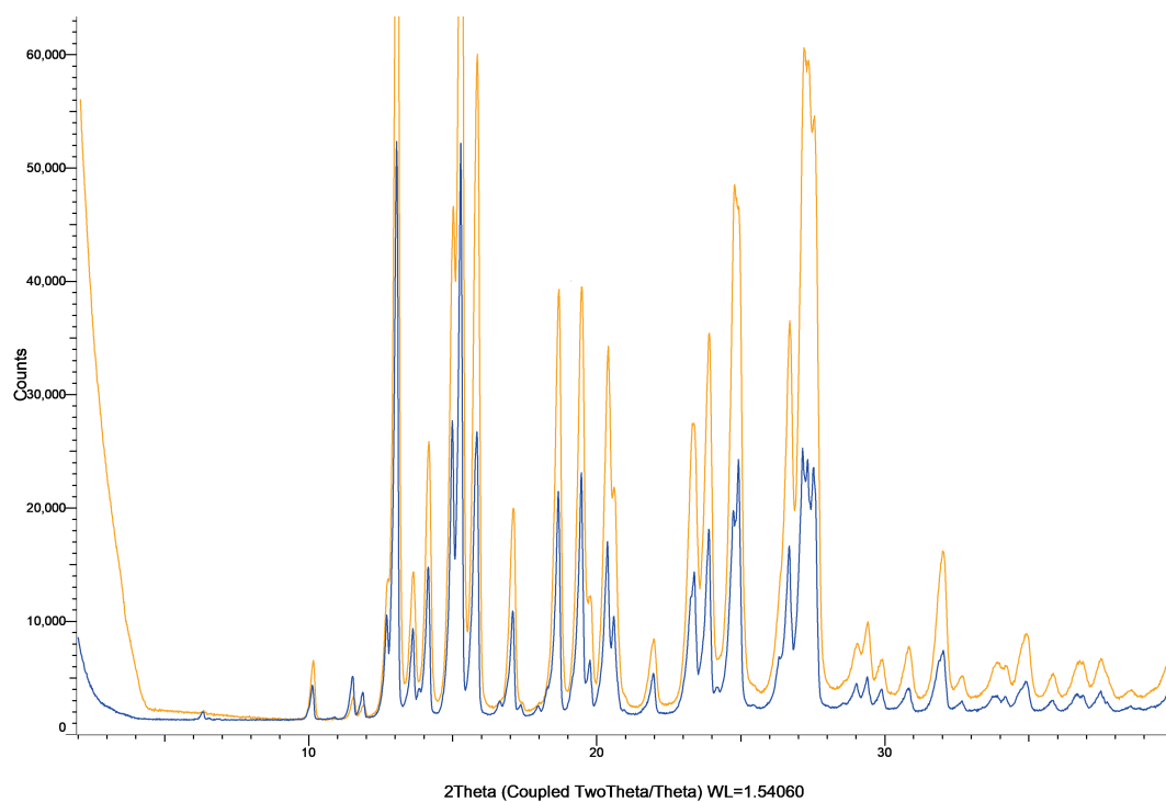
Figure S40: XRPD patterns of carbamazepine powder (blue) and milled carbamazepine powder (orange).
