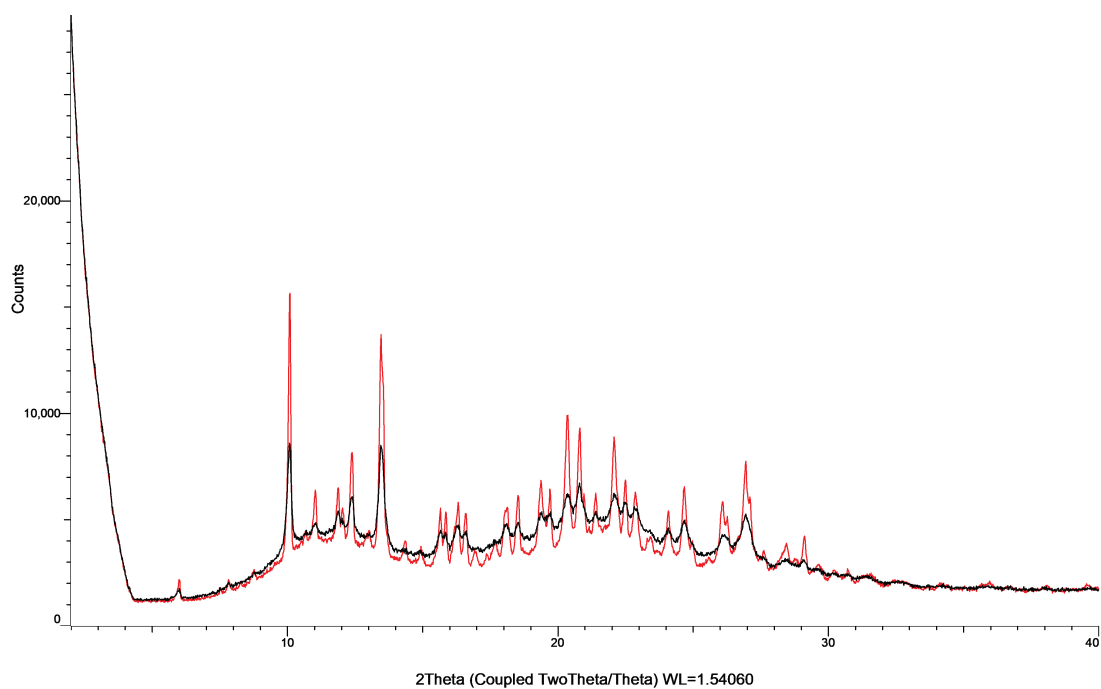
Figure S9: XRPD patterns of aripiprazole with PVP K25 in co-milled mixtures (black) and physical mixtures (red).
