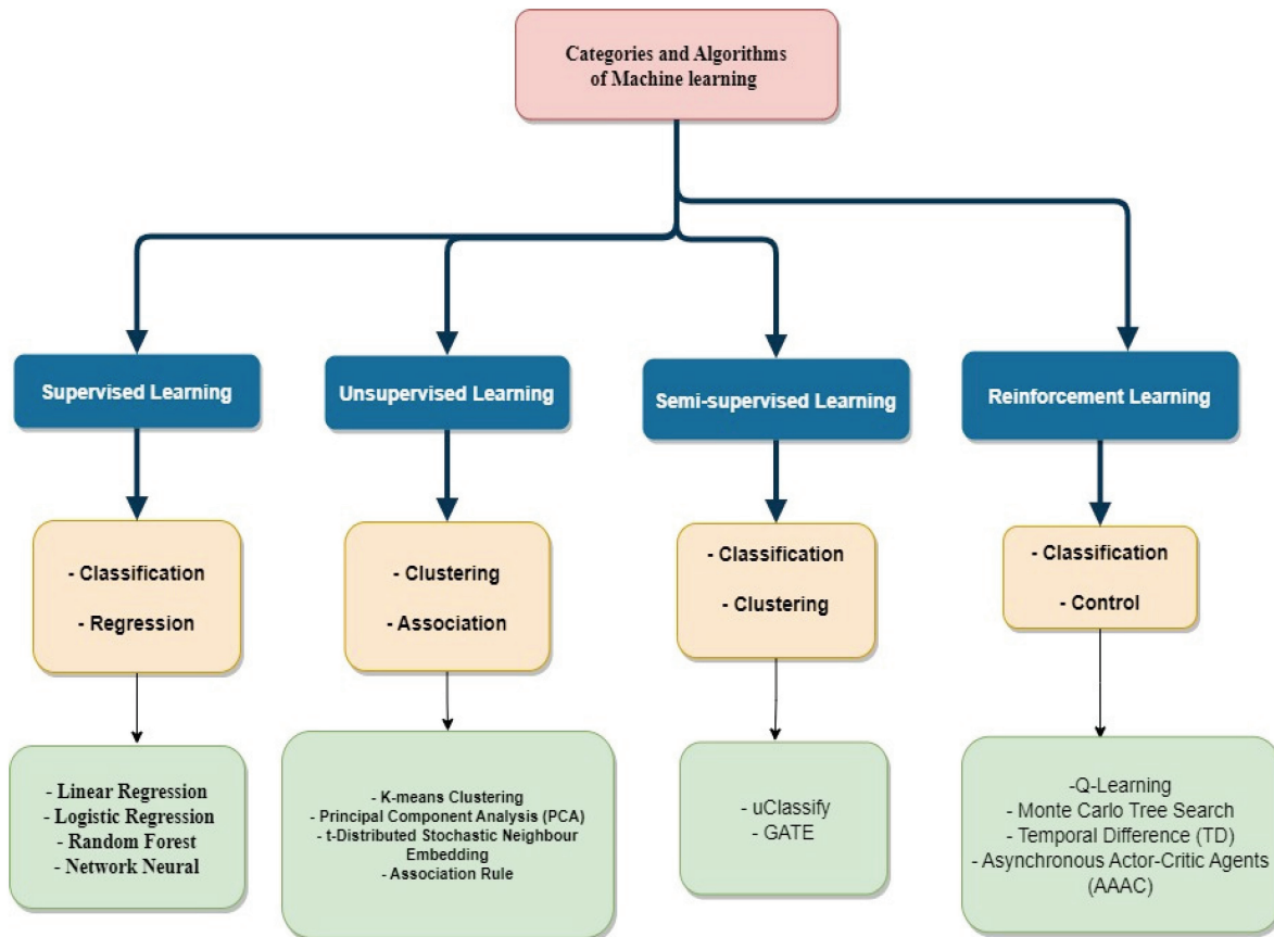
Figure 1-9: Overview of the main categories and representative algorithms of machine learning, extracted from (Taye, 2023). The diagram distinguishes four major learning paradigms: Supervised learning, unsupervised learning, semi-supervised learning, and reinforcement learning. Each category is associated with specific tasks such as classification, regression or clustering and employs characteristic algorithms tailored to its objectives.
