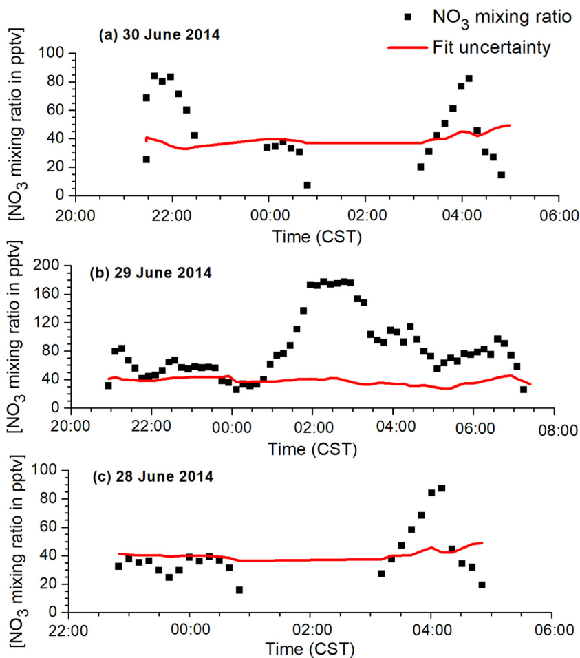
Fig. 7. Black trace (solid square) shows the real time NO_3 mixing ratio for all three days. The red trace (solid line) shows the estimated fit uncertainty of the measurements. The maximum mixing ratio ( \sim 175 pptv) for NO_3 was recorded on 29 June 2014.
