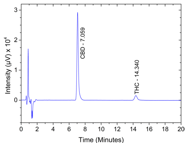
Figure 2. System suitability chromatogram of CBD and THC standard mixture (10 \mu\text{g/mL} CBD and 1 \mu\text{g/mL} THC) for assay.
