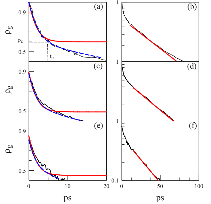
FIG. 2. (Color online) Experimental GS carrier relaxations (black), fitting with Eqs. (1) and (2) (blue), and fitting (red) with: [(a), (c), and (e)] Eq. (5) for the fast recovery stage; [(b), (d), and (f)] Eq. (8) for the slow recovery stage. The fitting parameters were: [(a) and (b)] \tau_w=18 ps; [(c) and (d)] \tau_w=12 ps; and [(e) and (f)] \tau_w=8 ps. The other parameters are the same as in Fig. 1.
