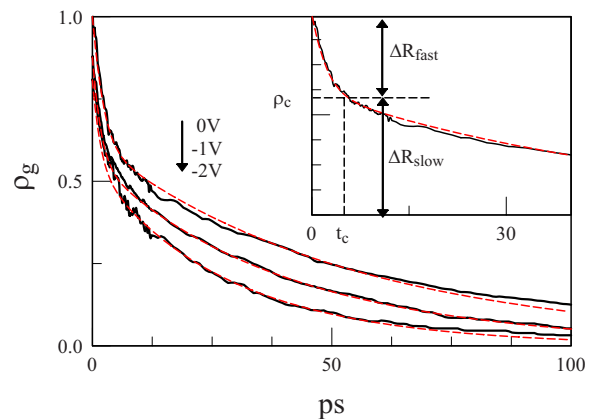
FIG. 1. (Color online) Experimental GS carrier relaxation for different reverse biased voltages (black) and fitting (red) with Eqs. (1) and (2): (a) 0 V, \tau_w = 18 \text{ ps} ; (b) 1 V, \tau_w = 12 \text{ ps} ; and (c) 2 V, \tau_w = 8 \text{ ps} . The other fitting parameters are: \tau_{\text{cap}} = 2 \text{ ps} and \tau_{\text{esc}} = 10 \text{ ps} . The inset illustrates t_c , \rho_c , \Delta R_{\text{slow}} , and \Delta R_{\text{fast}} which are introduced in the text.
