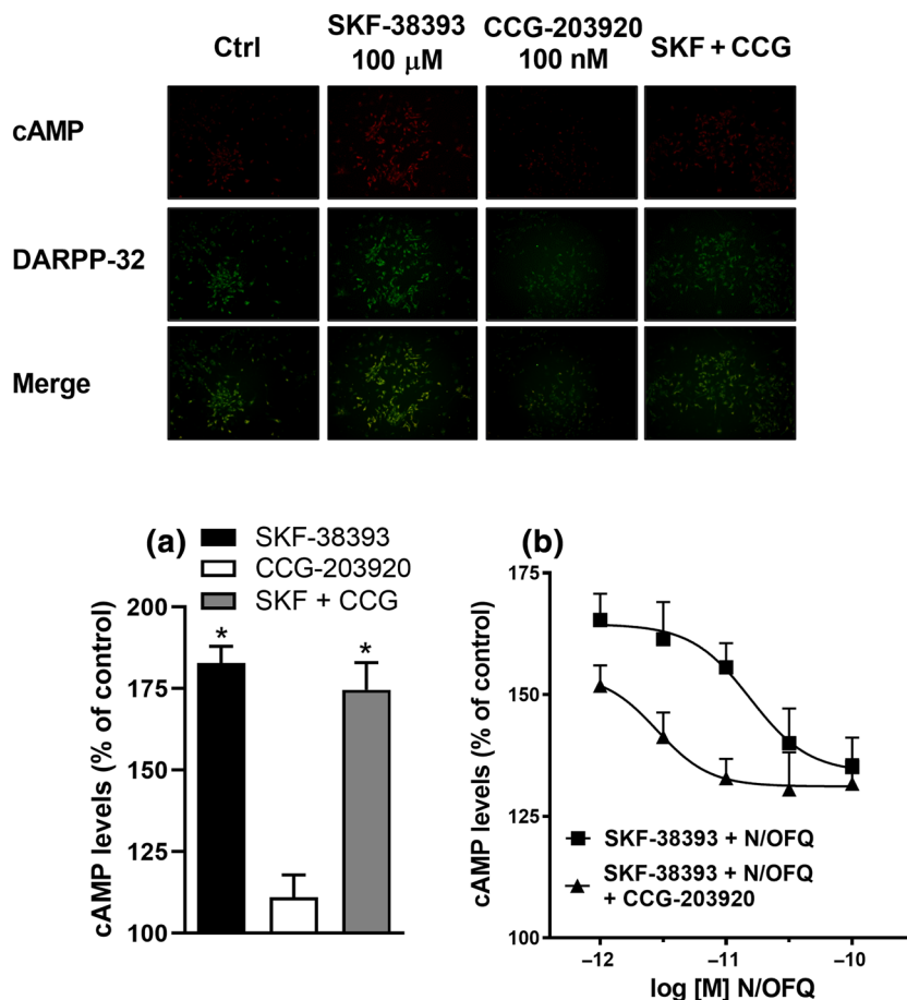
FIGURE 2 RGS4 reduced the NOP receptor agonist ability to attenuate the accumulation of cAMP triggered by D1 receptor agonist in DARPP-32+ striatal primary neurons. DARPP-32 is a marker of MSNs. Neurons were treated with the D1 receptor agonist SKF-38393 (100 \mu M) and the NOP receptor agonist N/OFQ (0.01–1 nM), in the presence or the absence of the experimental RGS4 chemical probe CCG-203920 (100 nM). (a) Primary effects of SKF-38393, CCG-203920 and their combination, with representative images (upper panels). (b) Concentration–response curves of N/OFQ in the presence or the absence of CCG-203920. Data are mean \pm SEM of n = 8 –10 experiments per group, namely, N/OFQ 0.001 nM n = 9 , N/OFQ 0.003 nM n = 8 , N/OFQ 0.01 nM n = 10 , N/OFQ 0.03 nM n = 10 (without CCG-203920) and n = 8 (with CCG-203920), N/OFQ 0.1 nM ( n = 9 ). * P < 0.05 , different from CCG-203920 (one-way ANOVA followed by the Bonferroni post hoc test)
