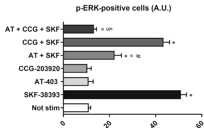
FIGURE 3 CCG-203920 potentiated the AT-403-driven inhibition of D1 receptor-stimulated ERK signalling in striatum. Number of ERK-positive cells in striatal slices of naïve mice following application of the D1 receptor agonist SKF-38393 (100 \mu M), the NOP receptor agonist AT-403 (30 nM) and the experimental RGS4 chemical probe CCG-203920 (50 nM) alone and in combination. Data are mean \pm SEM of n = 7 mice per group. * P < 0.05 , different from unstimulated vehicle; o P < 0.05 , different from SKF-38393 alone; # P < 0.05 different from AT-403 alone. § P < 0.05 , different from AT-403 + SKF-38393. Three-way ANOVA followed by the Bonferroni post hoc test
