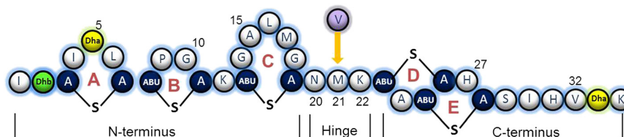
Figure 1 The structure of nisin A showing the location of the N-terminal domain, containing one lanthionine and two (β-methyl) lanthionine rings (A, B, and C) linked to the C-terminal intertwined rings (D and E) by a flexible hinge region. Post-translational modifications are highlighted as follows: dehydroalanine (Dha); dehydrobutyrate (Dhb); lanthionine (A-S-A) and (β-methyl) lanthionine (Abu-S-A). Standard residues are represented in the single letter code. Arrow indicates location of the methionine to valine substitution (M21V) in nisin V.
