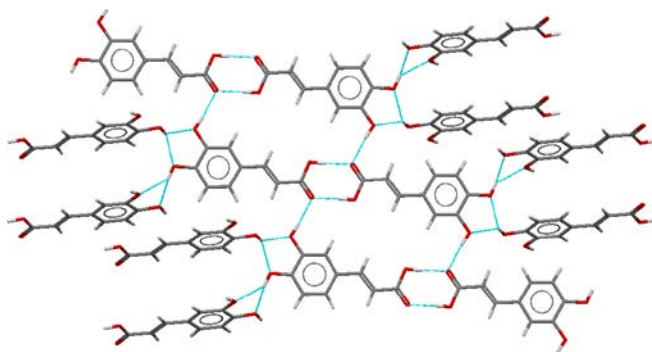
Figure 15. The structure of caffeic acid (FESNOG01). 65
