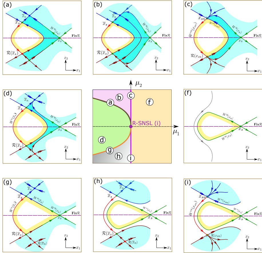
Fig. 2. Unfolding of the R-SNSL (i) bifurcation. The bifurcation diagram in the middle shows four different regions separated by codimension-one bifurcations. The corresponding schematic phase portraits are given in panels (a)–(i). Magenta line – saddle node bifurcation; brown curve – heteroclinic orbit flip; orange curve – heteroclinic saddle-saddle connection. Yellow shading – conservative region; blue shading – dissipative region; darker shading – emerging dissipative region with reversible heteroclinics.
