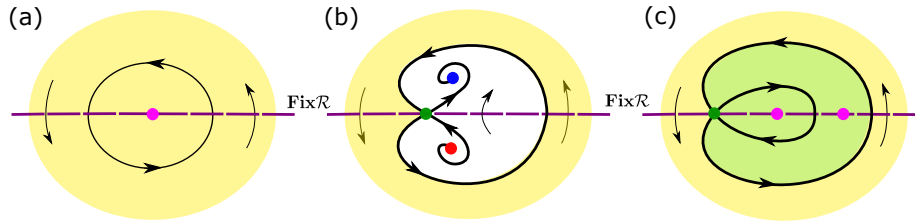
Fig. 7. Examples of schematic phase portraits of possible dynamics inside a conservative region. (a) A single conservative region with a single elliptic equilibrium. (b) A saddle equilibrium with a reversible homoclinic constitutes the boundary to a further dissipative region. (c) A saddle equilibrium with two reversible homoclinics constitutes the boundary to two further conservative regions. Stable, unstable and elliptic equilibria are indicated by blue, red and magenta colors.
