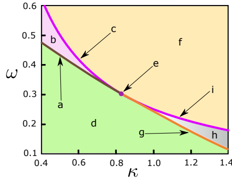
Fig. 5. Bifurcation diagram for system (9)–(10) in parameter plane (\kappa, \omega) in the neighborhood of the R-SNSL point (e). Bifurcation curves: magenta (c), (i) – saddle-node, orange (g) – saddle-saddle connection, brown (a) – homoclinic orbit flip.
