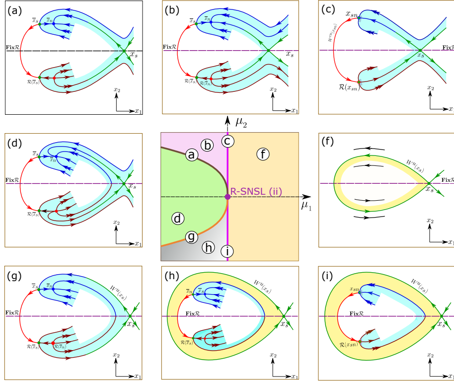
Fig. 3. Unfolding of the R-SNSL (ii) bifurcation. The bifurcation diagram in the middle shows four different regions separated by codimension-one bifurcations. The corresponding schematic phase portraits are given in panels (a)–(i). Magenta line – saddle node bifurcation; brown curve – heteroclinic orbit flip; orange curve – heteroclinic saddle-saddle connection. Yellow shading – conservative region; blue shading – dissipative region.
