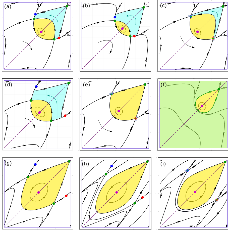
Fig. 6. Different types of phase portraits for the system (9)–(10) in phase space (\phi_1, \phi_2) \in [0, 2\pi] \times [0, 2\pi] . Parameters from the correspondingly marked bifurcation curves and regions in Fig. 5. Structurally stable phase portraits – (b), (d), (f), (h). Codimension-one situations – (a), (c), (g), (i). Codimension-two R-SNSL point of type (i) – (e). Colored regions: yellow – librations, green – rotations (conservative); white and blue – dissipative regions. Equilibrium points: red — source, blue — sink, green — saddle, magenta — center. Degenerate equilibria are marked with two-colored circles. The dashed purple line – \mathbf{Fix} \mathcal{R} .
