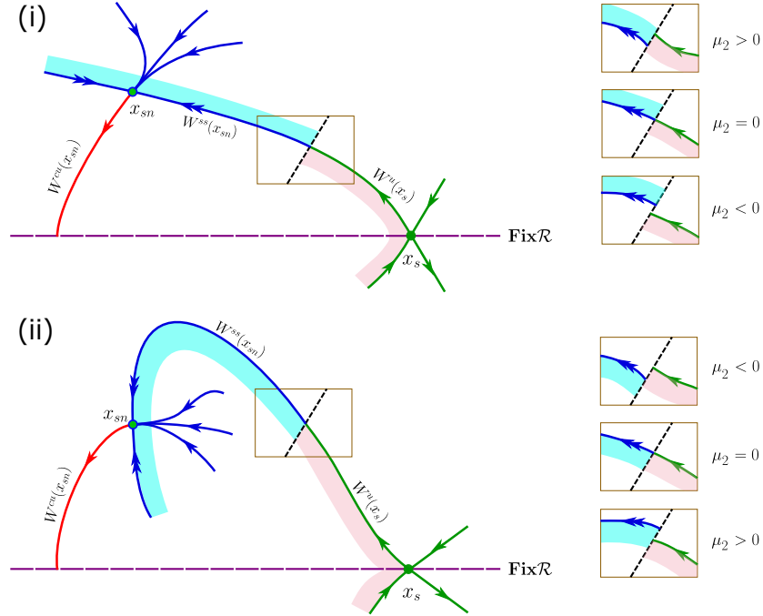
Fig. 1. Illustration of assumptions (H1)-(H4) for R-SNSL bifurcations. Fixed subspace \mathbf{Fix} \mathcal{R} according to (H1) (purple). Saddle-node equilibrium according to (H2) with center-stable manifolds (blue). Generic intersection of its center-unstable manifold (red) with \mathbf{Fix} \mathcal{R} according to (H3). Reversible saddle equilibrium with stable and unstable manifold (green). The non-generic heteroclinic connection (7) and its unfolding by \mu_2 at a Poincaré section (dashed) according to (H4) is given in the boxes in the right row. The two different cases are distinguished by the fact that for \mu = (0, 0) the reversible trajectories close to W^u(x_s) (purple shaded region) can be outside (i) or inside (ii) of W^{cs}(x_{\text{sn}}) (blue shaded region).
