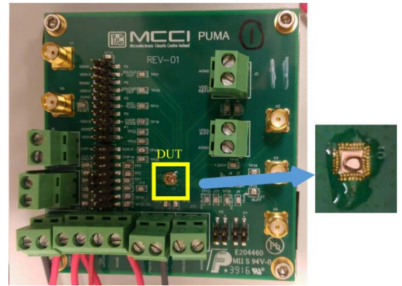
Fig. 16. Photograph of test-PCB.
