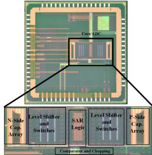
Fig. 15. Chip micrograph and core ADC.
