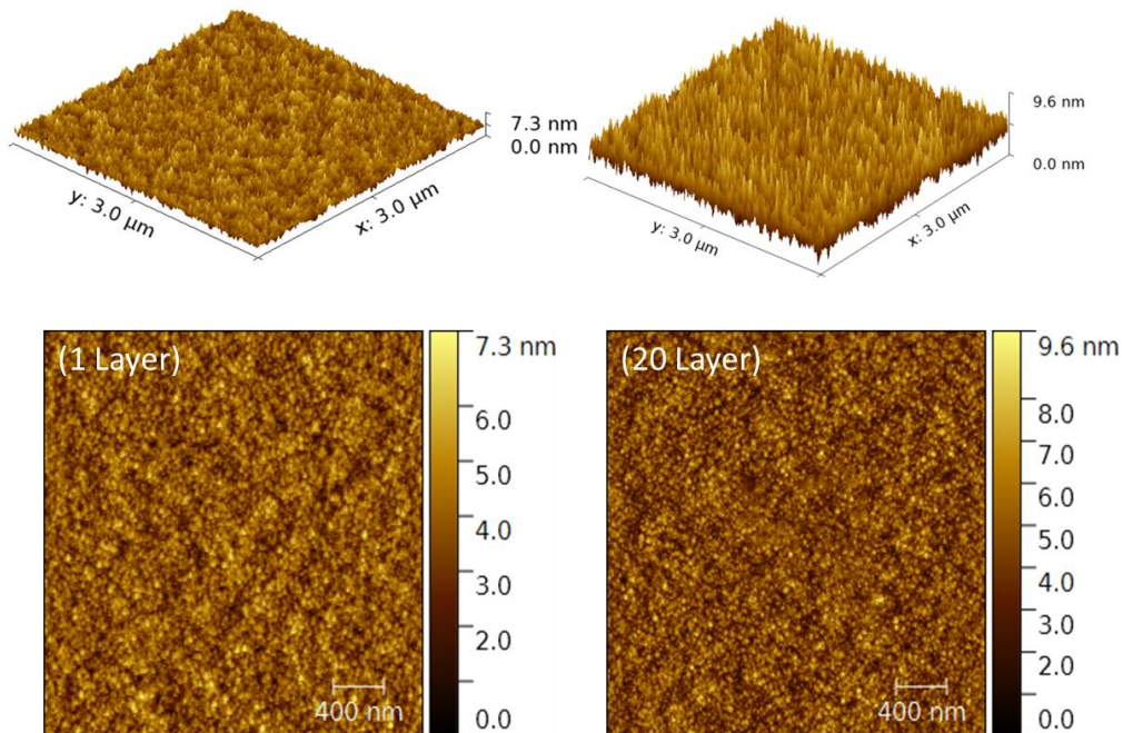
Figure 5. (Top) 3D AFM images showing the comparative roughness of 1 and 20 layer samples. (Bottom) AFM surface images for 1 and 20 layer ZnO thin films.
