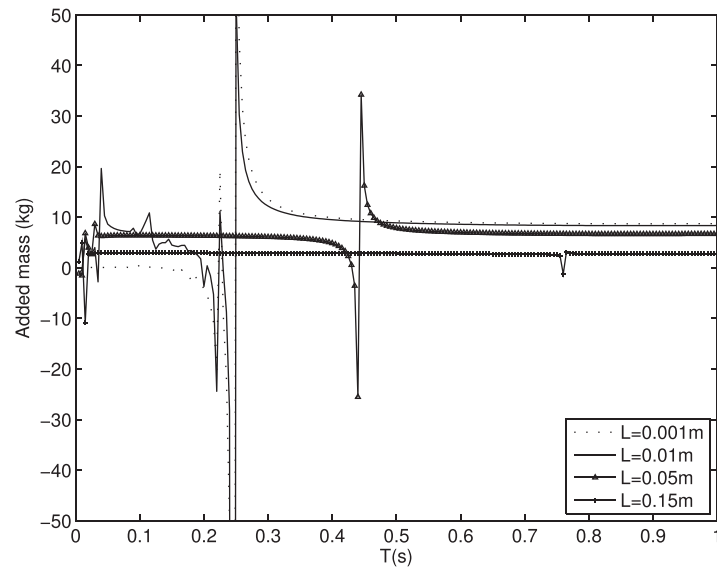
FIG. 9. Added mass predictions for the pistons with different lengths.
