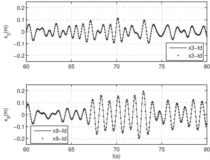
FIG. 25. Heave motions of the floating structure and the piston (piston length L = 0.10 m).
