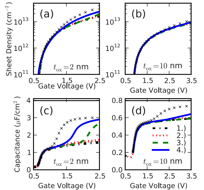
FIG. 3. (Color online) Electron sheet density vs gate voltage for t_{\text{ox}}=2 nm (a) and t_{\text{ox}}=10 nm (b). Total capacitance ( D_{\text{it}}=0 ) for t_{\text{ox}}=2 nm (c) and t_{\text{ox}}=10 nm (d). The four cases are: (1) parabolic \Gamma valley only, (2) \Gamma valley with nonparabolic corrections, (3) all valleys assuming parabolic bands, and (4) all valleys with nonparabolic corrections. Note that E_L=1.49 eV and E_X=1.98 eV except for the symbols which are case (4) with E_L=1.2 eV and E_X=1.33 eV. The horizontal lines in (c) and (d) are C_{\text{ox}} .
