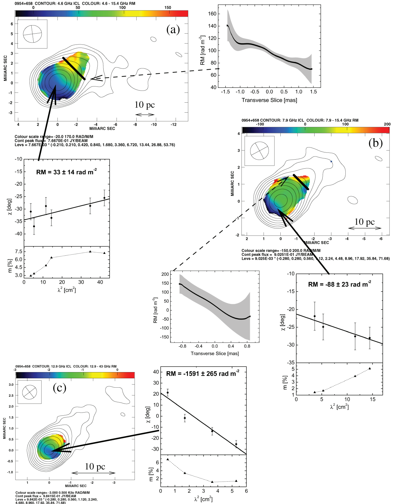
Figure 5. Source: 0954+658. (a) 4.6–15.4 GHz RM map (colour scale RM range: -20 to 170 rad m ^{-2} ) with 4.6 GHz total intensity contours ( I peak 0.77 Jy beam ^{-1} ; lowest contour 1.61 mJy beam ^{-1} ). The solid arrow points to the core region where the \chi versus \lambda^2 fits shown in the inset were found; the degree of polarization is plotted underneath for each corresponding polarization angle. The dashed arrow points to the indicated slice taken across the RM map; the plotted black line shows the RM fit at every pixel across the slice with the grey area indicating the error in the fit for each point. (b) 7.9–15.4 GHz RM map (colour scale RM range: -150 to 200 rad m ^{-2} ) with 7.9 GHz total intensity contours ( I peak 0.90 Jy beam ^{-1} ; bottom contour 2.53 mJy beam ^{-1} ). (c) 12.9–43 GHz RM map (colour scale RM range: -3 to 0.5 \times 10^3 rad m ^{-2} ) with 12.9 GHz total intensity contours ( I peak 0.98 Jy beam ^{-1} ; lowest contour 2.76 mJy beam ^{-1} ). All I contours increase by factors of 2.
