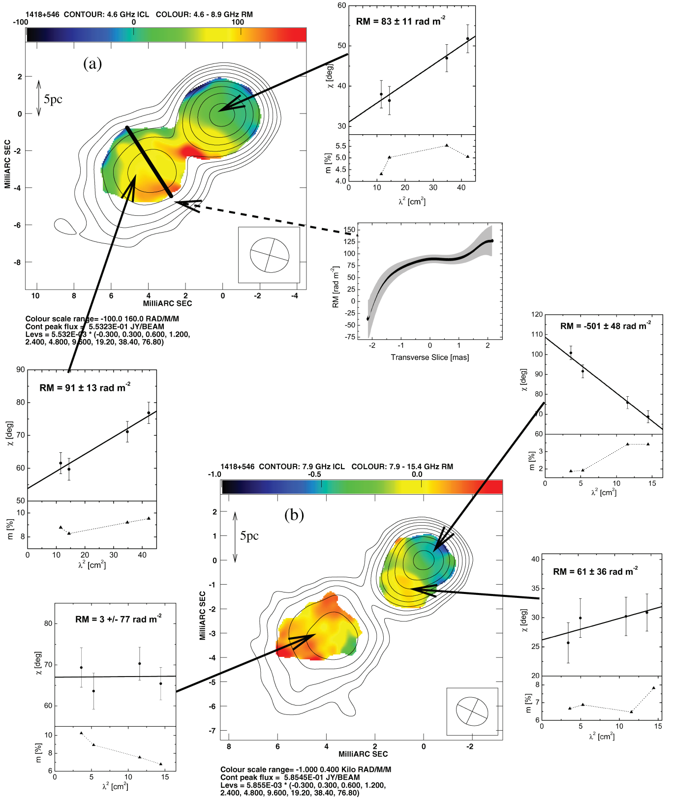
Figure 11. Source: 1418+546. (a) 4.6–8.9 GHz RM map (colour scale RM range: -100 to 160 rad m ^{-2} ) with 4.6 GHz total intensity contours ( I peak 0.55 Jy beam ^{-1} ; lowest contour 1.66 mJy beam ^{-1} ). The solid arrow points to the core region where the \chi versus \lambda^2 fits shown in the inset were found; the degree of polarization is plotted underneath for each corresponding polarization angle. The dashed arrow points to the indicated slice taken across the RM map; the plotted black line shows the RM fit at every pixel across the slice with the grey area indicating the error in the fit for each point. (b) 7.9–15.4 GHz RM map (colour scale RM range: -1 to 0.4 \times 10^3 rad m ^{-2} ) with 7.9 GHz total intensity contours ( I peak 0.59 Jy beam ^{-1} ; lowest contour 1.76 mJy beam ^{-1} ). All I contours increase by factors of 2.
