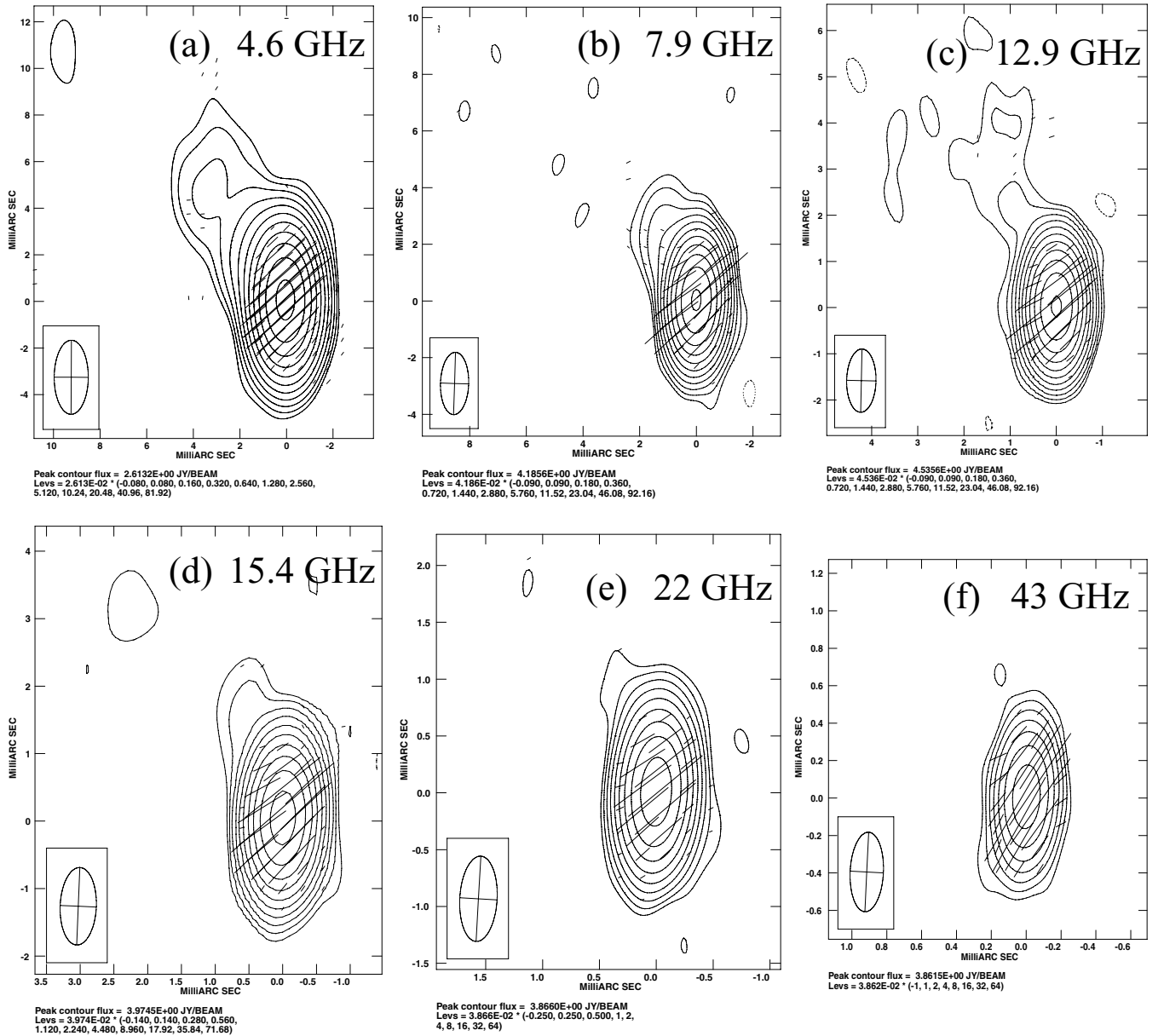
Figure 14. Total intensity ( I ) and polarization ( p ) maps for 1749+096: (a) 4.6 GHz, I peak 2.61 \text{ Jy beam}^{-1} , lowest contour 2.09 \text{ mJy beam}^{-1} , p vectors clipped at 2.5 \text{ mJy beam}^{-1} ; (b) 7.9 GHz, I peak 4.19 \text{ Jy beam}^{-1} , lowest contour 3.77 \text{ mJy beam}^{-1} , p vectors clipped at 2.5 \text{ mJy beam}^{-1} ; (c) 12.9 GHz, I peak 4.54 \text{ Jy beam}^{-1} , lowest contour 4.08 \text{ mJy beam}^{-1} , p vectors clipped at 3.0 \text{ mJy beam}^{-1} ; (d) 15.4 GHz, I peak 3.97 \text{ Jy beam}^{-1} , lowest contour 5.56 \text{ mJy beam}^{-1} , p vectors clipped at 3.0 \text{ mJy beam}^{-1} ; (e) 22 GHz, I peak 3.87 \text{ Jy beam}^{-1} , bottom contour 9.67 \text{ mJy beam}^{-1} , p vectors clipped at 4.5 \text{ mJy beam}^{-1} ; (f) 43 GHz, I peak 3.86 \text{ Jy beam}^{-1} , lowest contour 38.62 \text{ mJy beam}^{-1} , p vectors clipped at 5.0 \text{ mJy beam}^{-1} . The I contours increase by factors of 2 in all maps. Length of p vectors represents relative polarized intensity.
