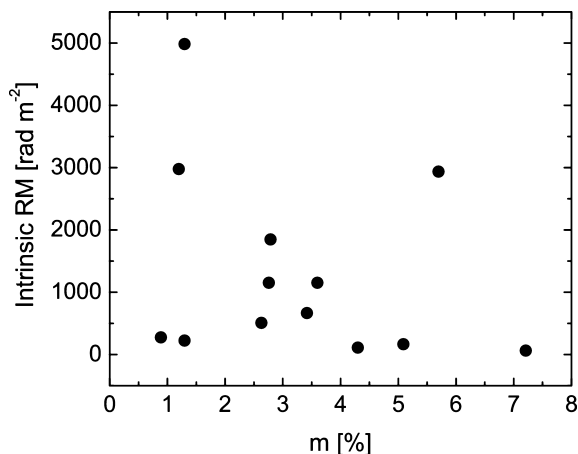
Figure 24. Plot of intrinsic core RM [ \text{RM}_{\text{intrinsic}} = \text{RM}_{\text{observed}}(1 + z)^2 ] for all sources versus the corresponding core degree of polarization ( m ) listed in Table 5. There is clearly a lack of highly polarized cores with high core RMs.
