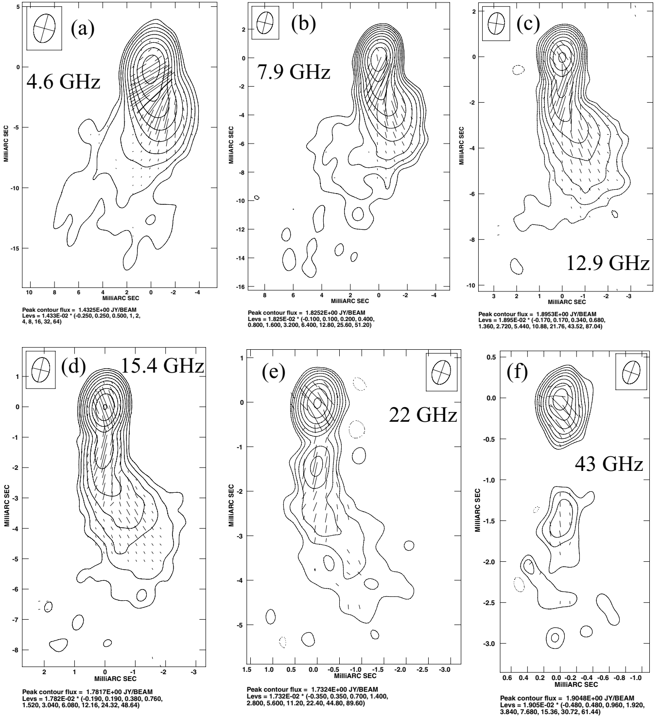
Figure 19. Total intensity ( I ) and polarization ( p ) maps for 2200+420: (a) 4.6 GHz, I peak 1.43\text{ Jy beam}^{-1} , lowest contour 3.58\text{ mJy beam}^{-1} , p vectors clipped at 1.5\text{ mJy beam}^{-1} ; (b) 7.9 GHz, I peak 1.83\text{ Jy beam}^{-1} , lowest contour 1.83\text{ mJy beam}^{-1} , p vectors clipped at 1.5\text{ mJy beam}^{-1} ; (c) 12.9 GHz, I peak 1.90\text{ Jy beam}^{-1} , lowest contour 3.22\text{ mJy beam}^{-1} , p vectors clipped at 1.8\text{ mJy beam}^{-1} ; (d) 15.4 GHz, I peak 1.78\text{ Jy beam}^{-1} , lowest contour 3.39\text{ mJy beam}^{-1} , p vectors clipped at 2.0\text{ mJy beam}^{-1} ; (e) 22 GHz, I peak 1.73\text{ Jy beam}^{-1} , bottom contour 6.06\text{ mJy beam}^{-1} , p vectors clipped at 4.0\text{ mJy beam}^{-1} ; (f) 43 GHz, I peak 1.90\text{ Jy beam}^{-1} , lowest contour 9.14\text{ mJy beam}^{-1} , p vectors clipped at 5.5\text{ mJy beam}^{-1} . The I contours increase by factors of 2 in all maps. Length of p vectors represents relative polarized intensity.
