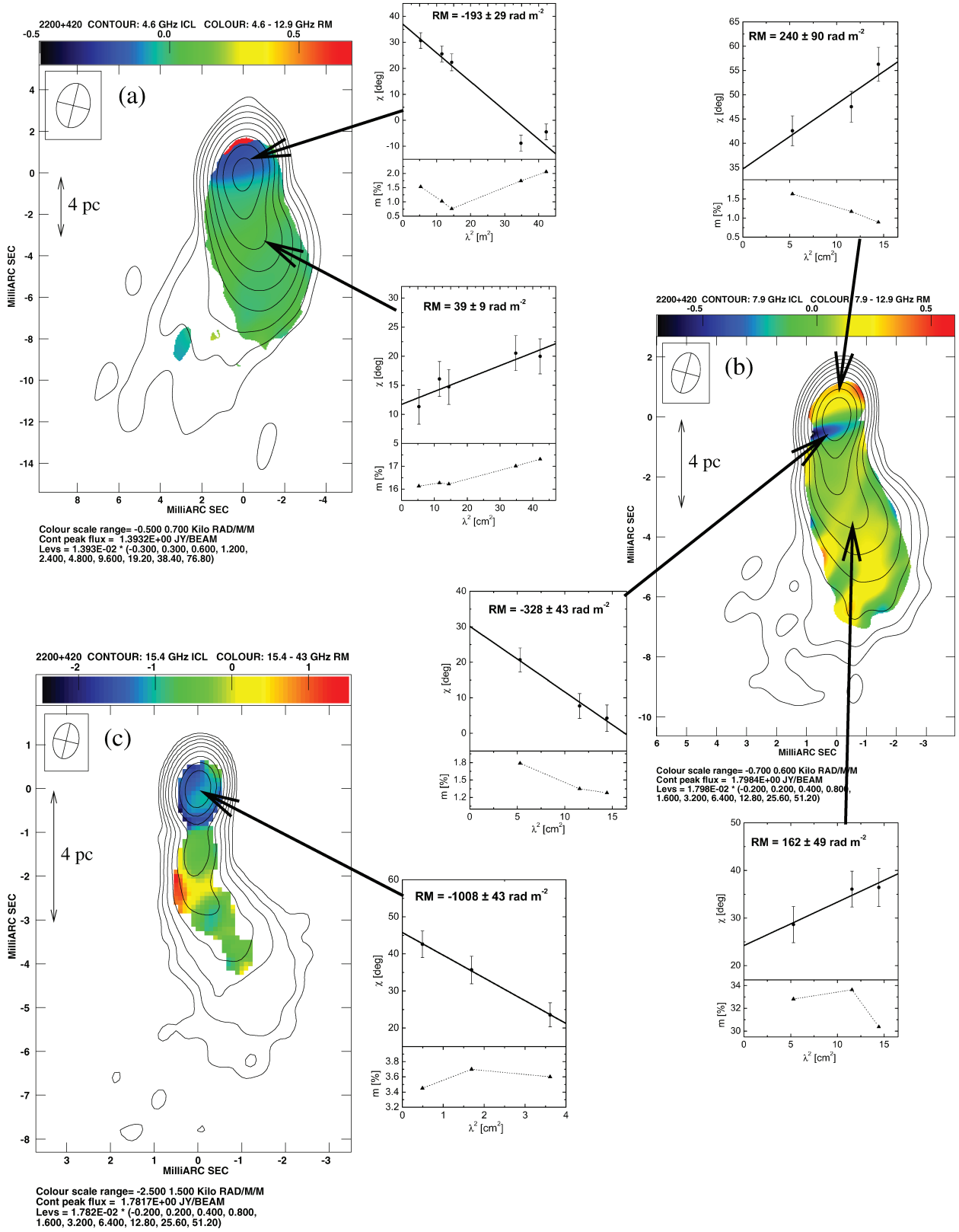
Figure 20. Source: 2200+420. (a) 4.6–12.9 GHz RM map (colour scale RM range: -0.5 to 0.7 \times 10^3 rad \text{m}^{-2} ) with 4.6 GHz total intensity contours ( I peak 1.39 Jy beam ^{-1} ; lowest contour 4.18 mJy beam ^{-1} ). The solid arrow points to the core region where the \chi versus \lambda^2 fits shown in the inset were found; the degree of polarization is plotted underneath for each corresponding polarization angle. The dashed arrow points to the indicated slice taken across the RM map; the plotted black line shows the RM fit at every pixel across the slice with the grey area indicating the error in the fit for each point. (b) 7.9–12.9 GHz RM map (colour scale RM range: -0.7 to 0.6 \times 10^3 rad \text{m}^{-2} ) with 7.9 GHz total intensity contours ( I peak 1.80 Jy beam ^{-1} ; lowest contour 3.60 mJy beam ^{-1} ). (c) 15.4–43 GHz RM map (colour scale RM range: -2.5 to 1.5 \times 10^3 rad \text{m}^{-2} ) with 15.4 GHz total intensity contours ( I peak 1.78 Jy beam ^{-1} ; lowest contour 3.56 mJy beam ^{-1} ). All I contours increase by factors of 2.
