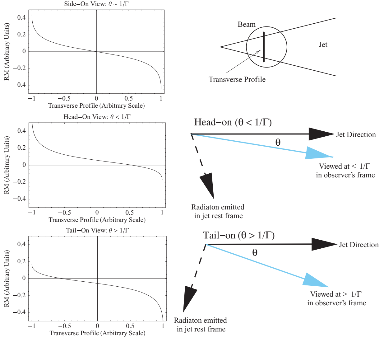
Figure 26. Top right: cartoon of a conical jet with the heavy line indicating a transverse profile of the jet. The circle is an example of the finite resolution of our VLBI observations. Middle right: because of the relativistic motion of the jet towards us, radiation emitted at <90^\circ in the jet rest frame is observed at <1/\Gamma , where \Gamma is the bulk Lorentz factor of the jet. Bottom right: radiation emitted at >90^\circ in the jet rest frame is observed at >1/\Gamma . Top left: transverse RM profile of a jet surrounded by a sheath of Faraday rotating material and viewed at 90^\circ in the jet rest frame. Because of the finite resolution of our observations a zero net RM would be observed. Middle left: transverse RM profile for a jet viewed ‘head-on’ ( <90^\circ in the jet rest frame). If we cannot resolve the transverse jet structure a net positive RM will be observed. Bottom left: transverse RM profile for a jet viewed ‘tail-on’ ( >90^\circ in the jet rest frame). In this case, a net negative RM will be observed if the transverse structure is resolved out.
