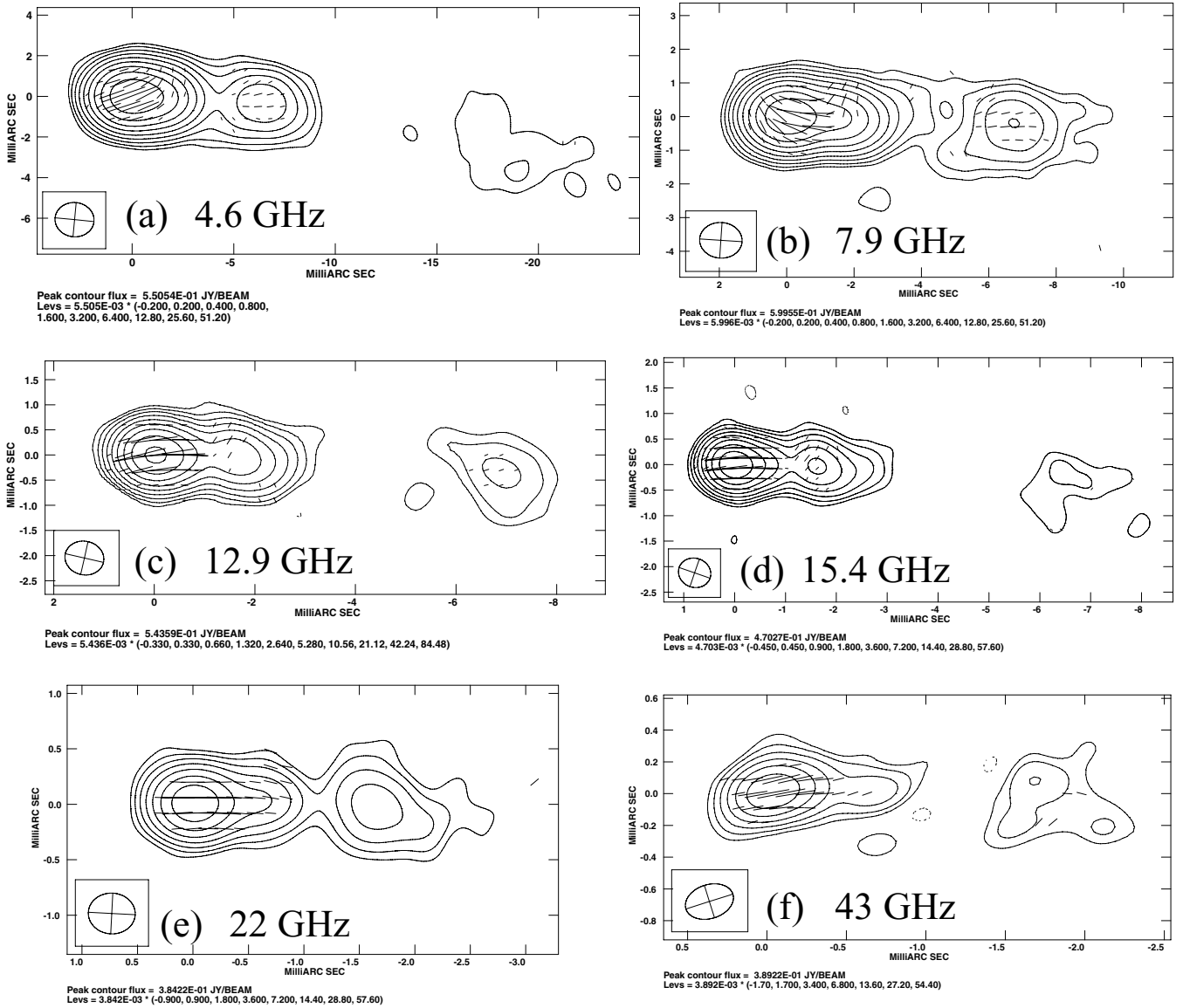
Figure 16. Total intensity ( I ) and polarization ( p ) maps for 2007+777: (a) 4.6 GHz, I peak 0.55 \text{ Jy beam}^{-1} , lowest contour 1.10 \text{ mJy beam}^{-1} , p vectors clipped at 1.0 \text{ mJy beam}^{-1} ; (b) 7.9 GHz, I peak 0.60 \text{ Jy beam}^{-1} , lowest contour 1.20 \text{ mJy beam}^{-1} , p vectors clipped at 1.0 \text{ mJy beam}^{-1} ; (c) 12.9 GHz, I peak 0.54 \text{ Jy beam}^{-1} , lowest contour 1.79 \text{ mJy beam}^{-1} , p vectors clipped at 1.5 \text{ mJy beam}^{-1} ; (d) 15.4 GHz, I peak 0.47 \text{ Jy beam}^{-1} , lowest contour 2.12 \text{ mJy beam}^{-1} , p vectors clipped at 1.5 \text{ mJy beam}^{-1} ; (e) 22 GHz, I peak 0.38 \text{ Jy beam}^{-1} , bottom contour 3.46 \text{ mJy beam}^{-1} , p vectors clipped at 5.5 \text{ mJy beam}^{-1} ; (f) 43 GHz, I peak 0.39 \text{ Jy beam}^{-1} , lowest contour 6.62 \text{ mJy beam}^{-1} , p vectors clipped at 7.5 \text{ mJy beam}^{-1} . The I contours increase by factors of 2 in all maps. Length of p vectors represents relative polarized intensity.
