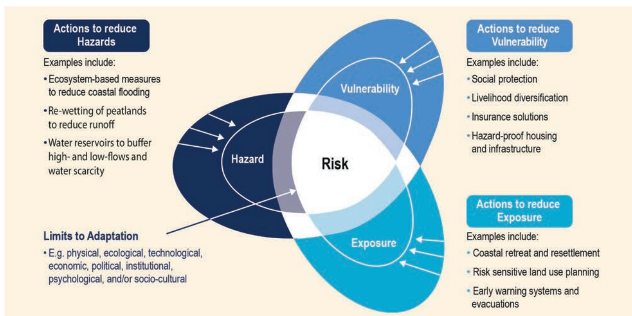
Figure SYR.3. Adaptation can reduce risk by addressing one or more of the three risk factors: vulnerability, exposure and/or hazard. A reduction in vulnerability, exposure and/or hazard potential can be achieved through different policy and action choices over time until limits to adaptation may be reached. Source: IPCC (2019, figure TS.4 (modified with permission)). 2
