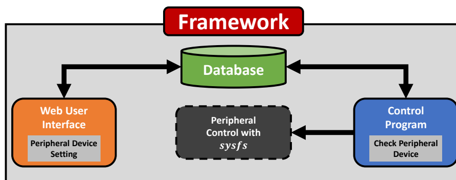
Figure 1. SoEasy framework.
