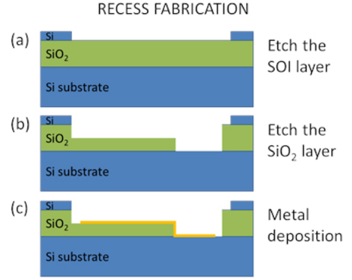
Fig. 4. (a) The recesses were fabricated by dry-etching the SOI layer, (b) the oxide (without reaching the Si substrate) and a recess to the Si substrate; (c) then a metal layer is evaporated to adjust the recess depth and sinks the heat to the substrate.
