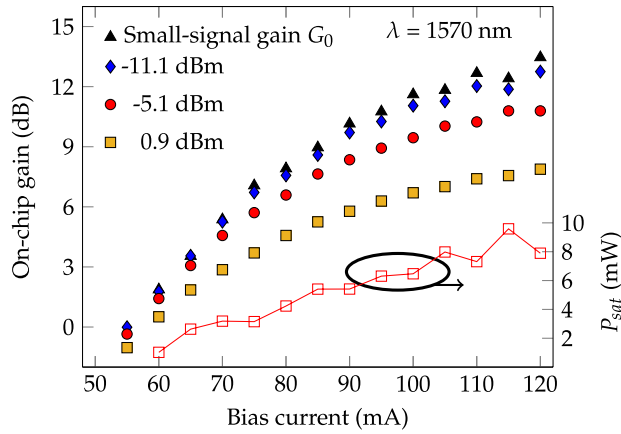
Fig. 5. On-chip gain of the III-V-on-Si 3 N 4 amplifier at 1570 nm as a function of bias current for three on-chip optical input levels. The fitting parameters G_0 and P_{\text{sat}} —extracted from the fits in Fig. 4—are shown.
