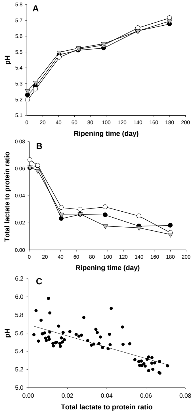
Figure 2.3. The effect of milk pre-treatments on (A) pH and (B) lactate to protein ratio of Maasdam cheese during maturation. Milk pre-treatments: control (●); centrifugation (▼); and centrifuged milk containing high heat-treated centrifugate (○). Data presented are means of data from three replicate trials. (C) Relationship between pH and lactate to protein ratio; data were obtained from all experimental cheeses produced in three replicate trials and analyzed over a 180 d of ripening.
