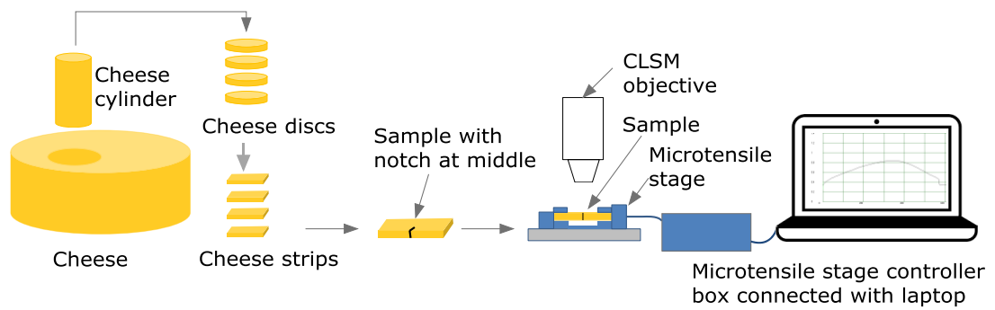
Figure 5.1. Schematic of experimental set-up for microtensile testing, showing sample preparation and accessories related to microtensile testing.
