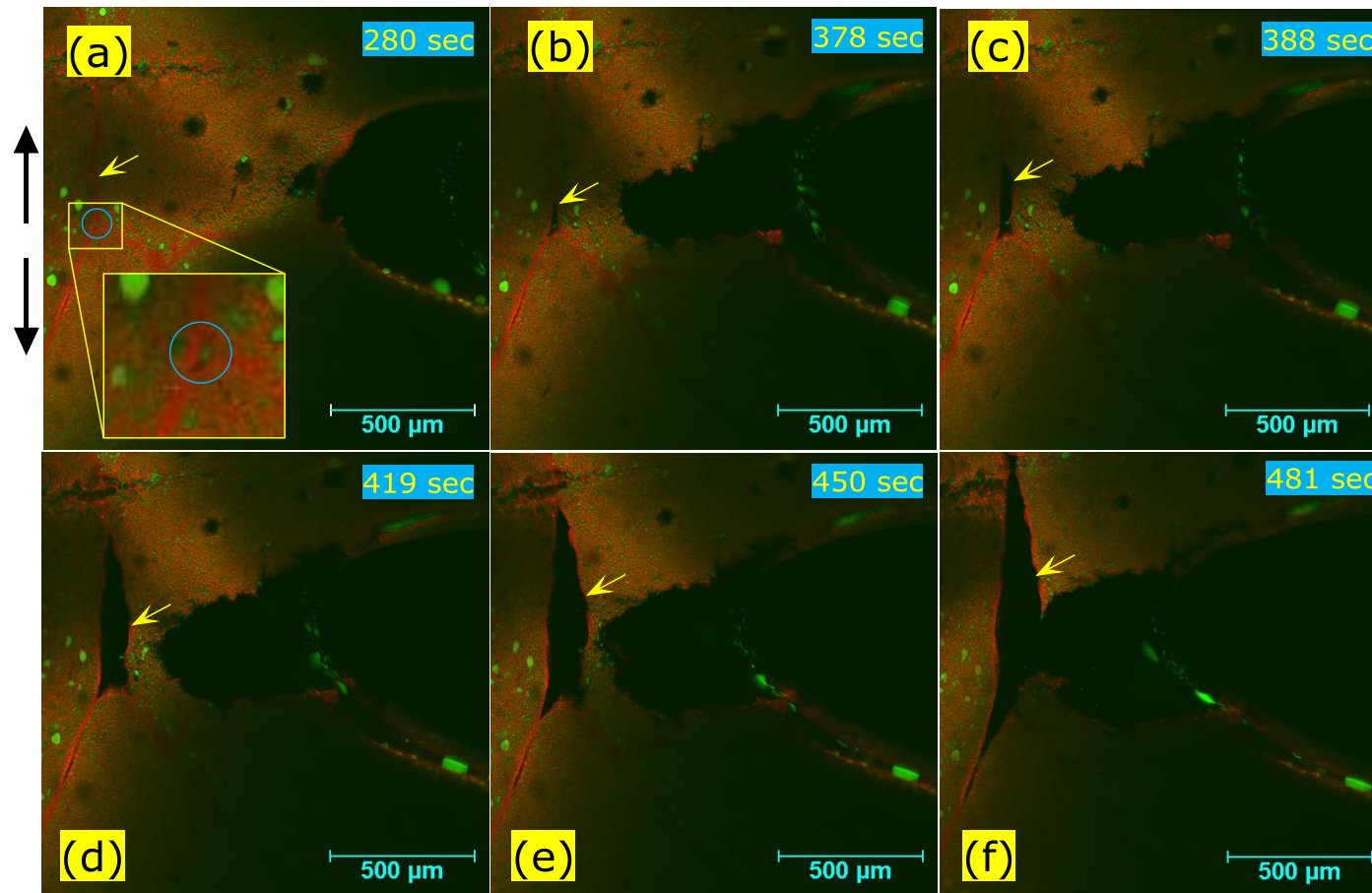
Figure 5.7. Sequence of confocal scanning laser microscopy (CSLM) images of cheese taken during tensile deformation of a notched cheese sample after 90 d of ripening, illustrating the fracture behaviour in the presence of an inherent defect at a curd granule junction. The circle, in the micrograph and in the inset (a), shows the inherent defect ( \sim 32 \mu\text{m} ) at a curd granule junction and the arrow shows the curd granule junction. Both the inherent defect and the notch (b-e) grew gradually and (f) merged during tensile deformation. The protein phase appears red while the fat phase appears green. Arrows beside the micrographs indicate the direction of tensile deformation.
