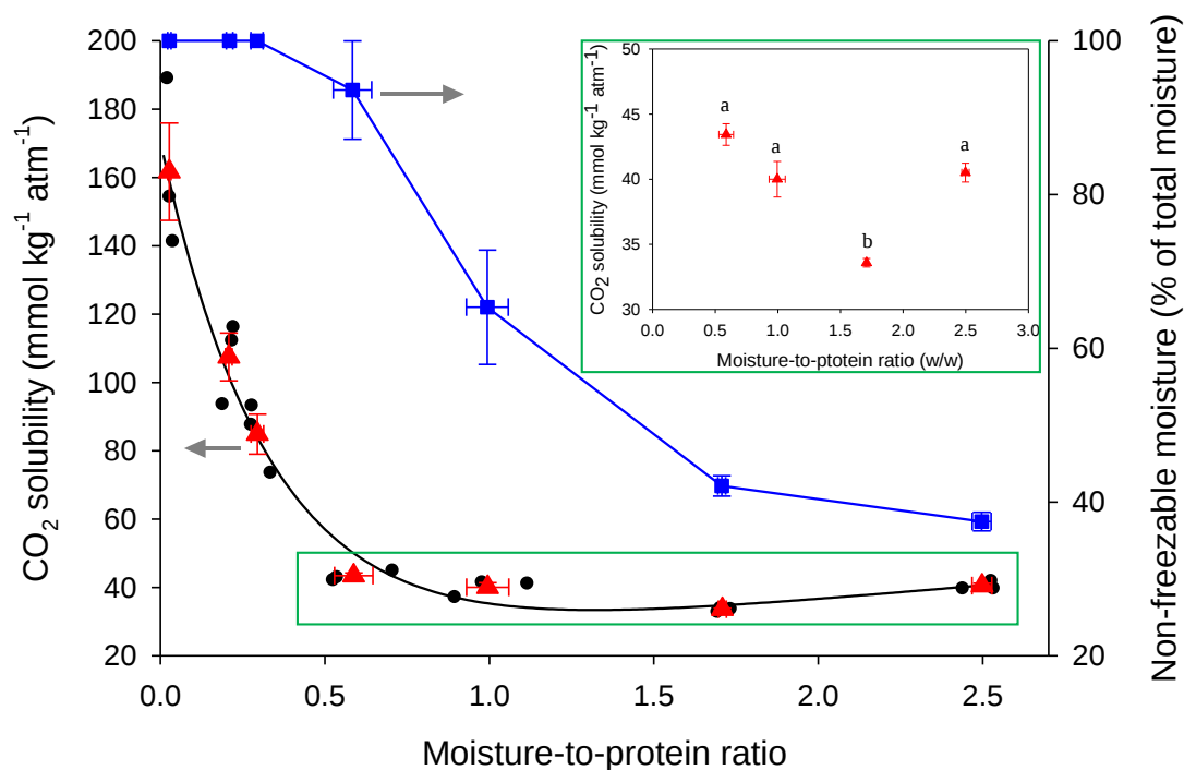
Figure 6.4. Relationships between moisture-to-protein ratio and (▲) CO 2 solubility or (■) non-freezable moisture (% of the total moisture) in renneted-casein matrices; (●) individual data points. Inset: magnification of CO 2 solubility data for casein matrices of moisture-to-protein ratio between 0.5 and 2.5; means with different letters differ ( P < 0.05 ). Error bars represent standard deviations of means ( n = 3 ).
