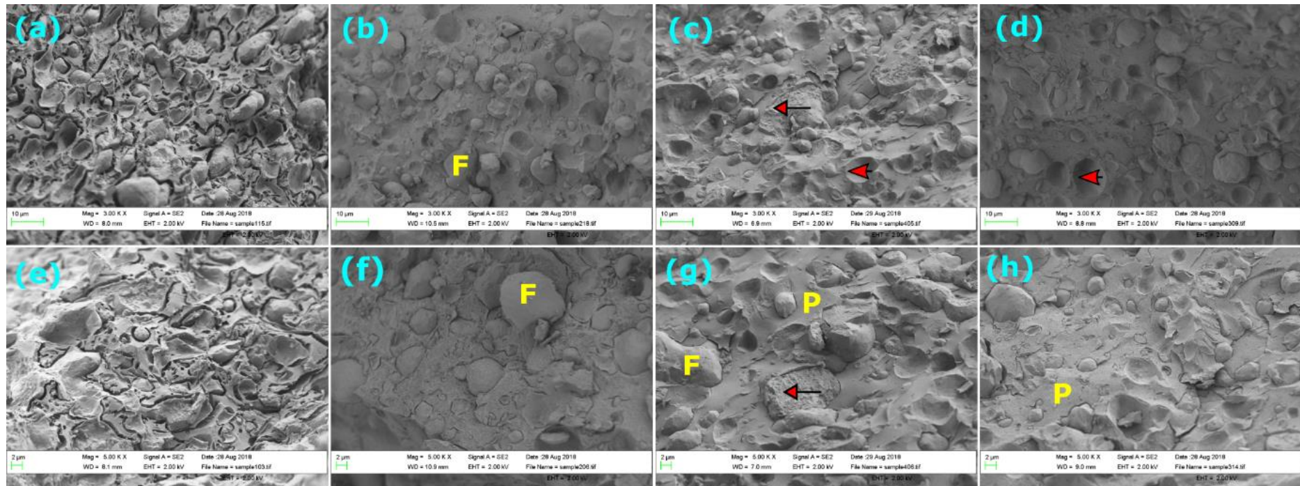
Figure 4.5. Selected cryo-SEM micrographs of (a, e) Control, (b, f) noWR, (c, g) CC, and (d, h) PepA cheeses after 90 d of ripening. Experimental cheese variants were Control (control cheeses), noWR (cheeses without warm-room ripening), CC (cheeses made from fermentation-produced camel chymosin as a coagulant), and PepA (cheeses containing chymosin inhibitor, i.e., pepstatin A). P = protein matrix, F = fat globules, short arrows = spherical imprints in the protein matrix left by fat globules that were removed during sample preparation, and long arrows = remnant fat from globules partially removed during sample preparation.
