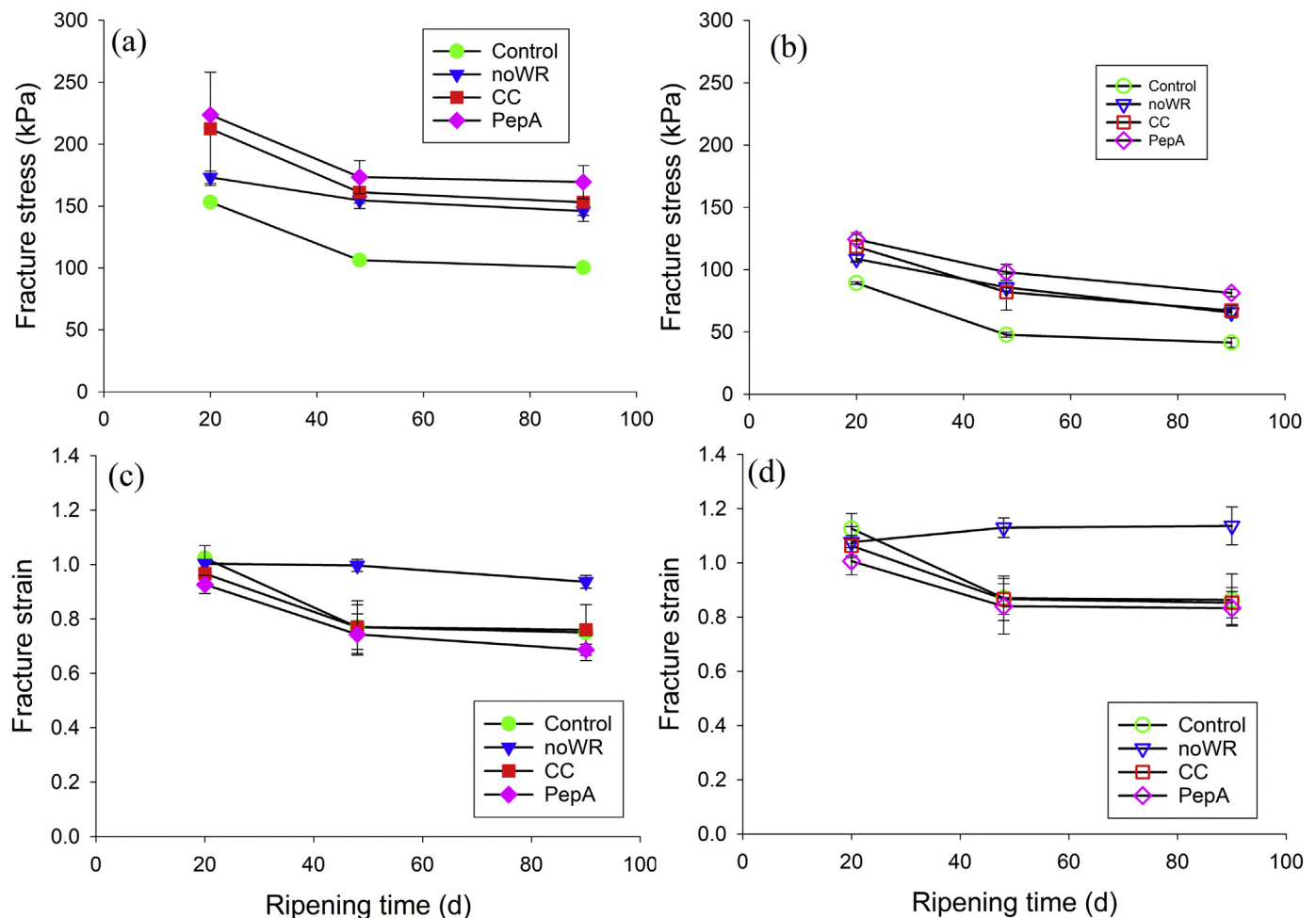
Fig. 4. Changes in (a–b) fracture stress ( \sigma_f , n = 2 ) and (c–d) fracture strain ( \epsilon_f , n = 3 ), measured at 4 °C (closed symbols) and 23 °C (open symbols), in semi-hard cheese during ripening. Error bars represent standard error of mean. Experimental cheese variants were Control (control cheeses), noWR (cheeses without warm-room ripening), CC (cheeses made from fermentation-produced camel chymosin as a coagulant), and PepA (cheeses containing chymosin inhibitor, i.e., pepstatin A).
