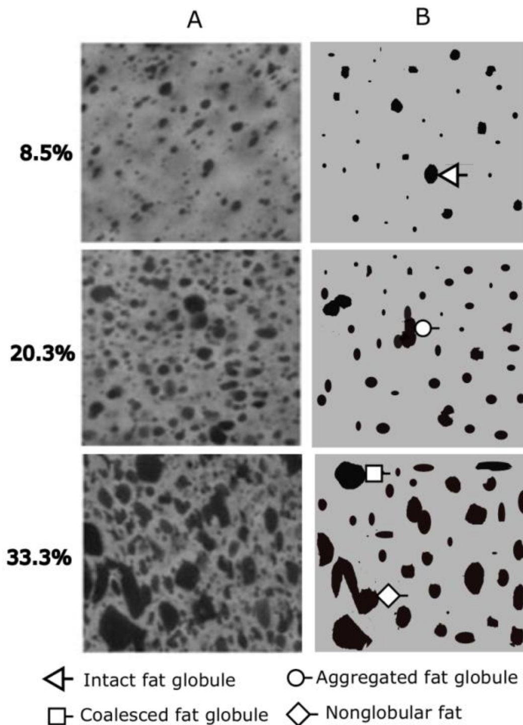
Figure 1.2. Column A shows confocal laser scanning microscopy images (100 \mu\text{m} \times 100 \mu\text{m} ) of Cheddar cheese (age: 12 wk) at 3 different fat levels (8.5%, 20.3% and 33.3%). Column B shows a schematic representation of Cheddar cheese microstructure, with intact fat globules, aggregated fat globules, coalesced fat globules, and nonglobular fats. The dark and gray areas represent fat globules and protein network within the cheese matrix, respectively. Adapted from Rogers et al. (2010) with permission.
