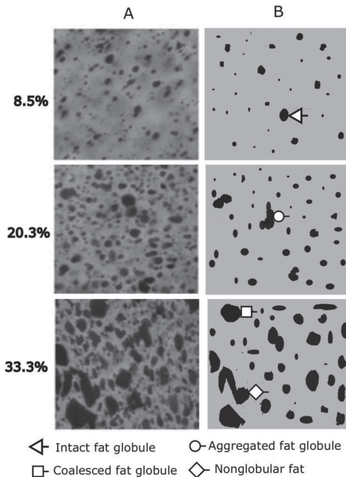
Figure 2. Column A shows the confocal laser scanning microscopy images ( 100 \mu\text{m} \times 100 \mu\text{m} ) of Cheddar cheese (age: 12 wk) at 3 different fat levels (8.5, 20.3, and 33.3%). Column B is the schematic representation of Cheddar cheese microstructure, with intact fat globules, aggregated fat globules, coalesced fat globules, and nonglobular fats. The dark and gray areas represent fat globules and protein network within the cheese matrix, respectively. Adapted from Rogers et al. (2010) with permission. Copyright (2010) American Dairy Science Association.
