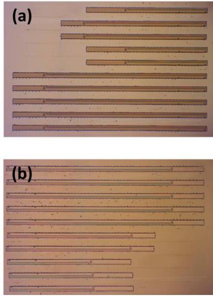
Fig. 6 Microscope images of QD laser coupons on (a) 5 nm BCB and (b) 35 nm BCB on Si substrate. Coupons are 1.5 mm, 1.8 mm and 2.4 mm long.
