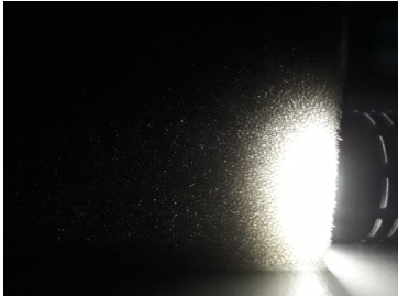
Figure 2.6: Light absorption in an absorbing medium.
