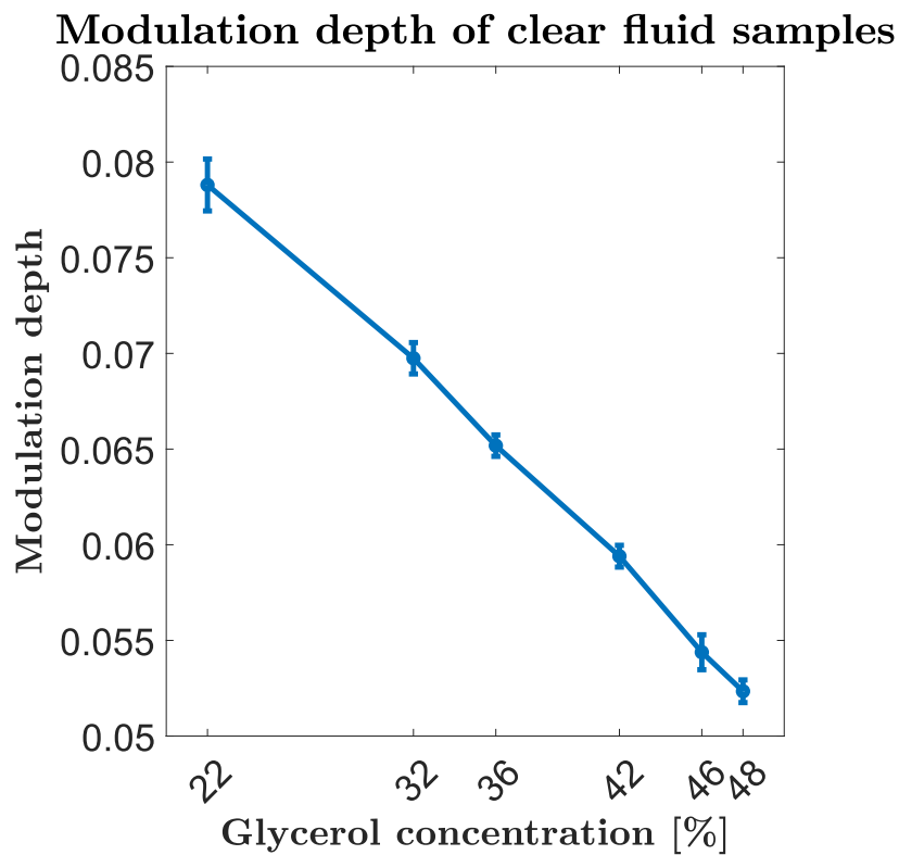
Figure 8.3: The modulation depth of non scattering aqueous glycerol of varying concentrations showing a negative dependence.
