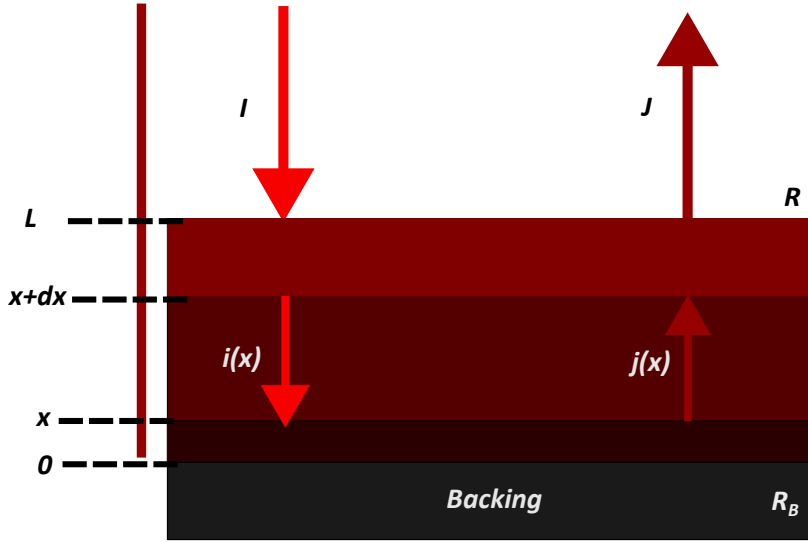
Figure 3.1: The Kubelka-Munk model of light-matter interaction.
