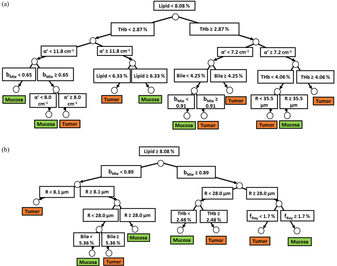
Figure 6. (a) Classification decision tree of the colorectal mucosa and tumor tissues based on parameter threshold values of probe 2 for f_{\text{lipid}} < 8.08\% . (b) Classification decision tree of the colorectal mucosa and tumor tissues based on parameter threshold values of probe 2 for f_{\text{lipid}} \geq 8.08\% .
