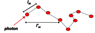
Figure 2.12: Illustration of scattering mean free path ( l_{sc} ) and transport mean free path ( l'_{sc} ).
