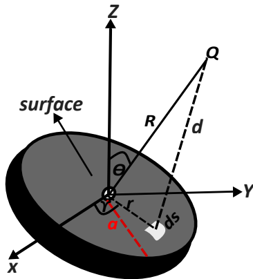
Figure 4.5: Ultrasound propagation by a cylindrical ultrasound transducer. Inspired from [44].
