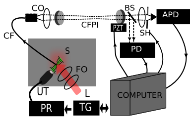
Figure 5.6: L=laser, TG= trigger generator, PR= pulser-receiver, UT= ultrasonic transducer, FO= focusing optics, CF= collecting fibre, S= sample, CO= coupling optics, PZT=piezoelectric transducer, BS=beam splitter, SH= shutter, PD= photo-detector. Inspired from [67].
