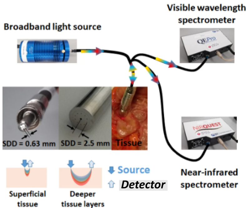
Figure 3.2: Diffuse reflectance system components. Inspired from [41].
