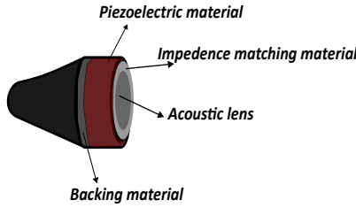
Figure 4.4: Parts of a cylindrical transducer.
