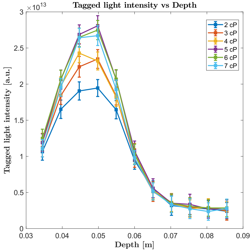
Figure 8.5: An axial acquisition of 11 data locations at an interval of 5.1 mm were collected. This corresponded to a scanning range from 3.45 cm to 8.55 cm from the ultrasound transducer. The plot shows the mean and the associated standard error.
