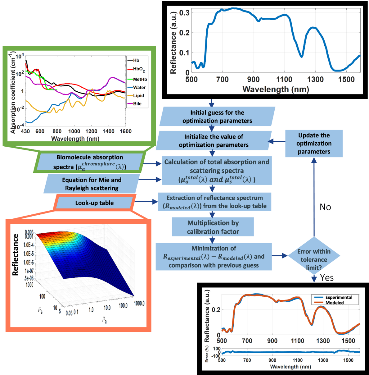
Figure 2. Flowchart of the steps of our spectral fitting algorithm.
