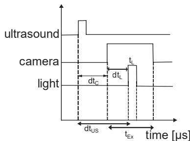
Figure 8.1: The delay ( dt_{US} ) of the ultrasound signal was used to scan in an around the embedded tube. The camera was opened at dt_L = 10 \mu\text{s} by adjusting dt_C before the acousto-optic interaction. The exposure time of the camera was t_{Ex} = 30 \mu\text{s} and the light stayed on for t_L = 4 \mu\text{s} .
