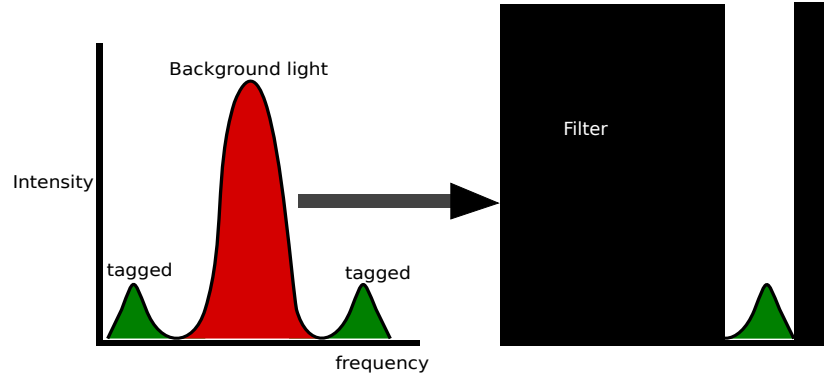
Figure 5.7: Spectral hole burning for filtering out tagged photon frequency. The wavelength shift between the background light and tagged light is 10^{-5} nm.
