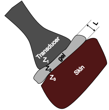
Figure 4.3: Impedance matching requirement for ultrasound imaging. The thickness of the gel is independent of the transmission coefficient of the wave that gets to the skin. For thick and thin layers ( L ), L = n\lambda/2 and L \ll \frac{\lambda}{4} respectively, where n is an integer [44].
