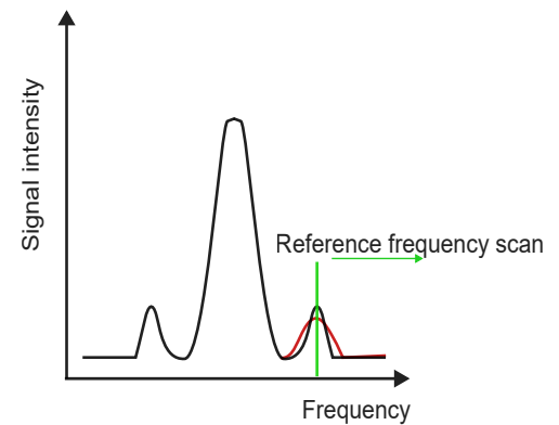
Figure 9.1: Frequency scanning for the flow rate and its effects on decorrelation. The frequency scan broadens the bandwidth of the frequency which is the red band.
