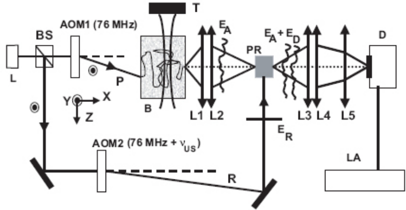
Figure 5.9: L:light source, BS:splits the laser beam into a probe(P) and a reference(R) beam, T: US piezo-transducer. AOM1,2: Acousto-optic modulators, E_A , E_D : fields associated to the speckle wavefronts. E_R : reference field. L1-L5 : wide aperture NA=1 aspherical lenses. B: chicken breast. PR: GaAs photorefractive crystal. LA: Lock-in amplifier. D: silicon photodetector ( S = 4.9 \text{ mm}^2 ). Copied from [88].
