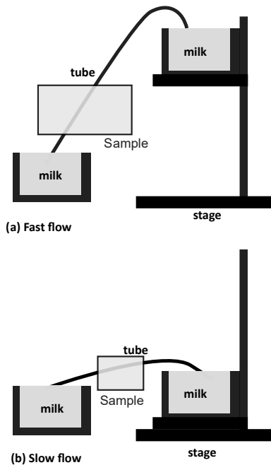
Figure 9.2: Using the siphoning principle to ensure different flow conditions: (a) fast flow condition ( 3 \text{ m s}^{-1} ), (b) slow flow condition ( 1.7 \text{ m s}^{-1} ).
