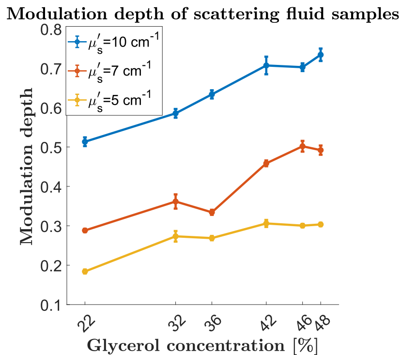
Figure 8.4: A study of the modulation depth dependence on optical scattering and glycerol concentration.
