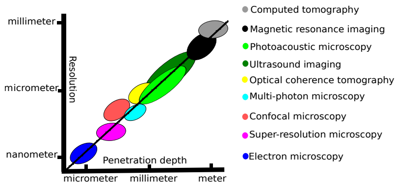
Figure 1.3: Resolution and penetration depth of various imaging modalities. This image was inspired from [11].
