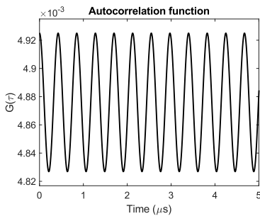
Figure 5.5: A time domain representation of the autocorrelation function [60].
