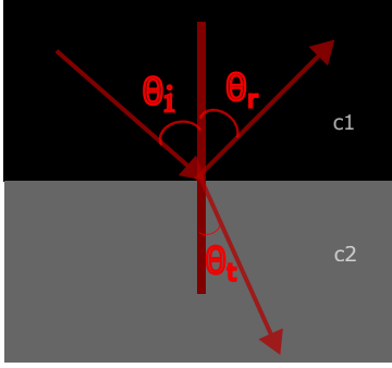
Figure 4.2: Snell's law depiction of ultrasound waves at the interface of two media.
