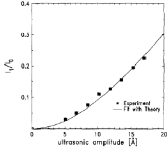
Figure 5.4: Modulation depth variation with respect to changes ultrasound amplitude [50].
