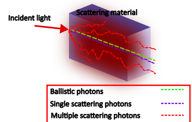
Figure 2.4: Photon scattering regimes.
