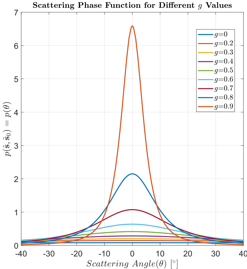
Figure 2.11: Relationship between scattering phase function and anisotropy. Typically for tissues, anisotropy that characterises scattering is 0.9. This shows the Henyey-Greenstein's phase function.
