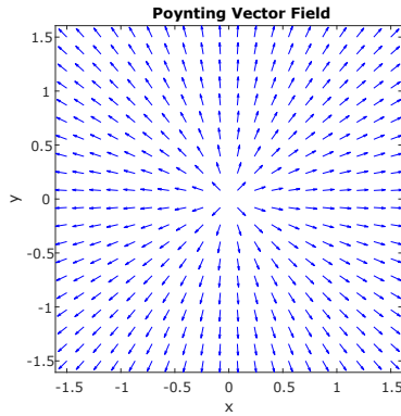
Figure 2.2: The Poynting vector field showing the flow of energy out of the page in the direction of \hat{\mathbf{s}} where the vector is the direction of the cross product between the magnetic and electric fields.
