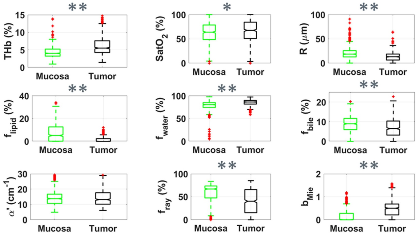
Figure 3. Boxplots of relevant parameters for differentiation between superficial tissue layers of mucosa (green, n = 728 ) and tumor (black, n = 635 ) by using probe 1. Red points represent outliers (points at more than 1.5 times the interquartile range away from the bottom or top of the box). Statistical difference for p < 0.05 is represented by * and that for p < 0.001 is represented by ** for the Wilcoxon rank sum test.
