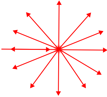
Figure 2.10: Isotropic scattering of the incident light. For isotropic scattering, g = 0 .
