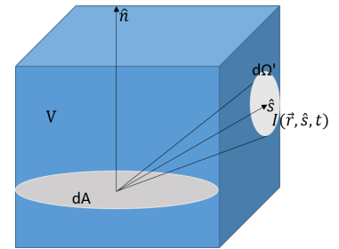
Figure 2.5: The spectral radiance from an area dA within a volume V . The spectral radiance is in the direction of the unit vector \hat{s} with a solid angle d\Omega' .
