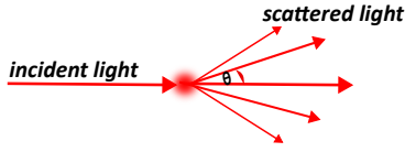
Figure 2.9: Anisotropic scattering of the incident light. For forward anisotropic scattering, g = 1 .
