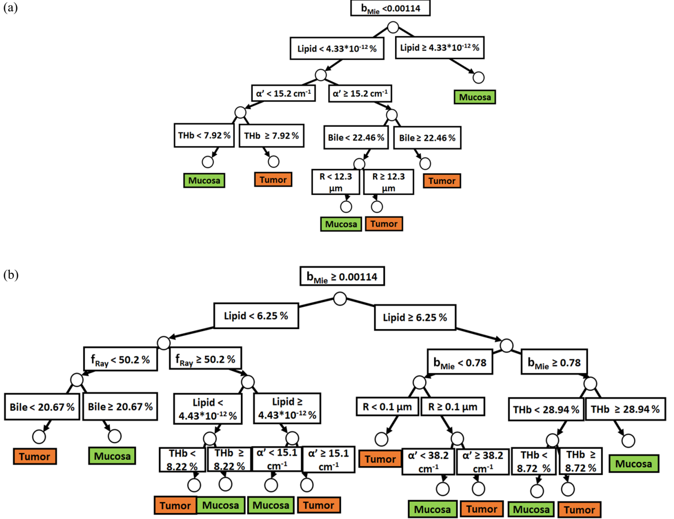
Figure 5. (a) Classification decision tree of the colorectal mucosa and tumor tissues based on parameter threshold values of probe 1 for b_{Mie} < 0.00114 . (b) Classification decision tree of the colorectal mucosa and tumor tissues based on parameter threshold values of probe 1 for b_{Mie} \geq 0.00114 .
