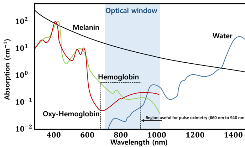
Figure 2.7: Wavelength dependence of optical absorption by chromophores in biological tissues. Inspired from [23].
