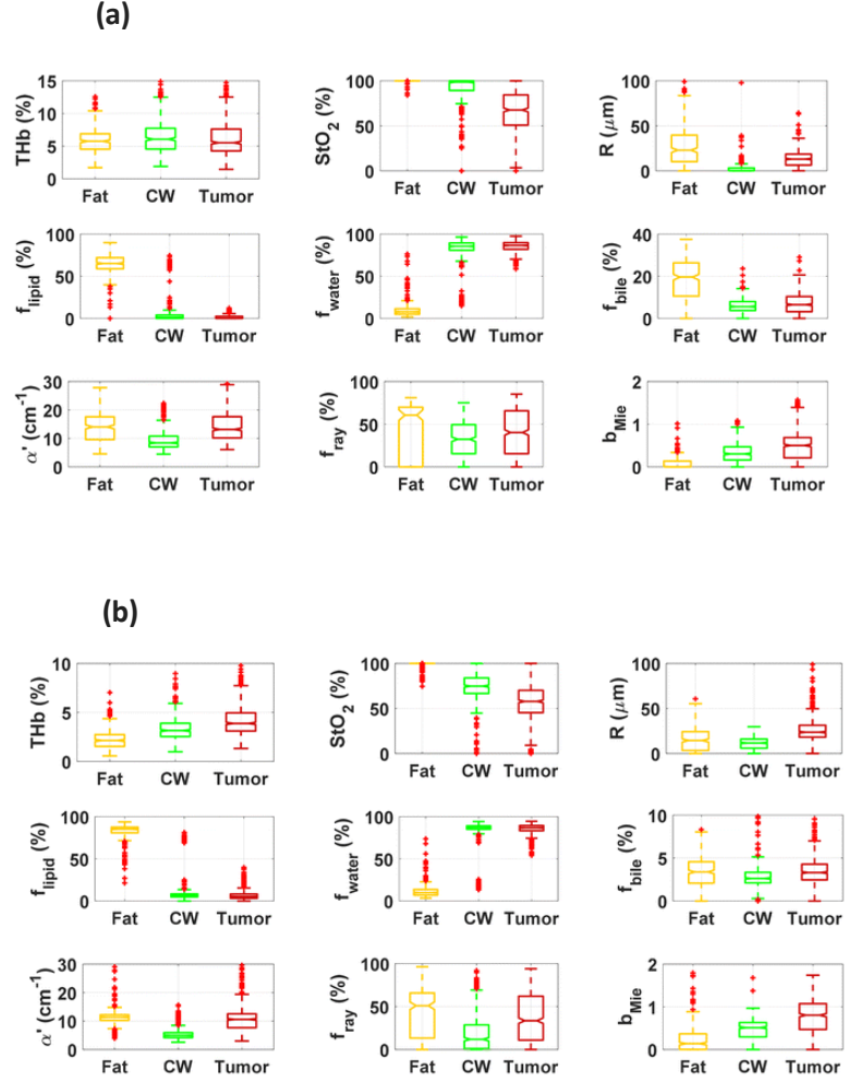
Figure 6.3: Boxplots showing tissue classification for small probe in (a) and large probe in (b). Copied from [41]. The outliers (red points) appear at more than (1.5 \times \text{the interquartile range}) in both (a) and (b). The changes in median are seen in biomarkers such as \alpha' , StO_2 , b_{Mie} and F_{Ray} .
