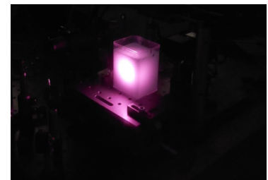
Figure 2.8: Light scattering in diffusive medium (agar block).
