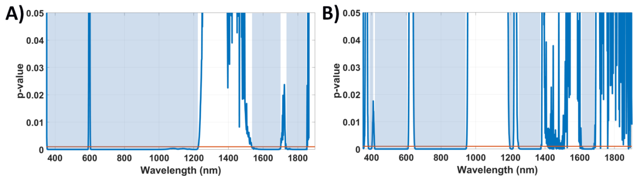
Figure 4. Selected spectral regions (blue) where statistically significant differences ( p < 0.001 ) are found for (A) short-SDD probe and (B) long-SDD probe. The red line indicates the 0.001 cutoff for the p -value.
