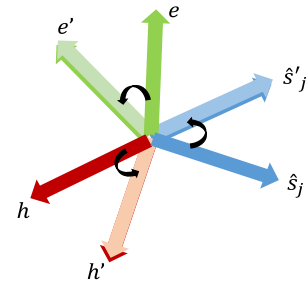
Figure 2.3: This shows the rotation of the direction of the Poynting vector, \hat{\mathbf{s}} unto an arbitrary direction \hat{\mathbf{s}}_j . This was inspired from [16].
