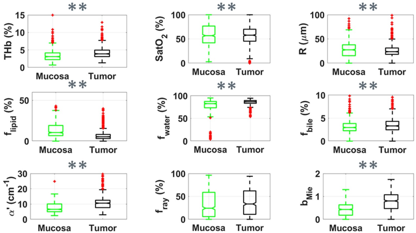
Figure 4. Boxplots of relevant parameters for differentiation between superficial tissue layers of mucosa (green, n = 804 ) and tumor (black, n = 722 ) by using probe 2. Red points represent outliers (points at more than 1.5 times the interquartile range away from the bottom or top of the box). Statistical difference for p < 0.05 is represented by * and that for p < 0.001 is represented by ** for the Wilcoxon rank sum test.
