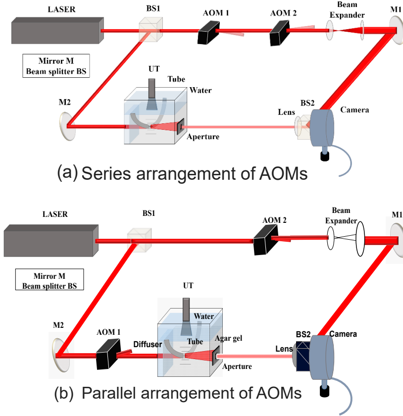
Figure 7.1: Digital heterodyne holography for the selection of ultrasound shifted light. A coherent laser source is split into an reference beam and a sample beam by a beam splitter (BS 1). From mirror (M2), the sample beam goes through a diffuser that is attached to a container holding the block of agar fitted with a tube containing blood mimicking fluid. The tube is placed in the focus of the Ultrasound transducer (UT). Water is used to couple the ultrasound wave propagation. An aperture is placed close to the sample holder the emerging light is focused on a lens (Bi-convex, focal length=75 mm) placed 5 cm away together with a beam splitter (BS2) and a camera. The sample beam is modulated by AOM 1 at 80 MHz at its -1 order was directed unto the sample. The reference beam was created with the -1 order of AOM 2 and modulated at 8 500 012 500 MHz before being expanded by a beam expander (Plano-concave lens, f = -30 mm). This was then reflected on mirror M1 unto the camera through beam splitter BS2.
