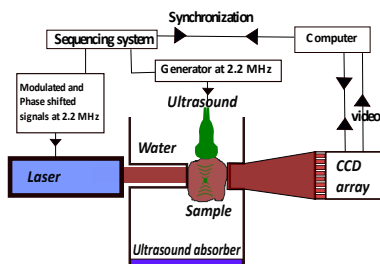
Figure 5.10: An ultrasound transducer modulates the speckles created by the laser beam within the sample. Instead of using a single optical detector, which combines the signals from many speckle grains, the CCD camera and parallel lock-in detection are used to record the full modulation of the speckle. Inspired from [101].
