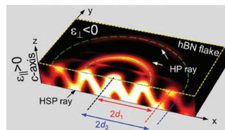
Figure 19: Two types of confined modes at an hBN flake with
