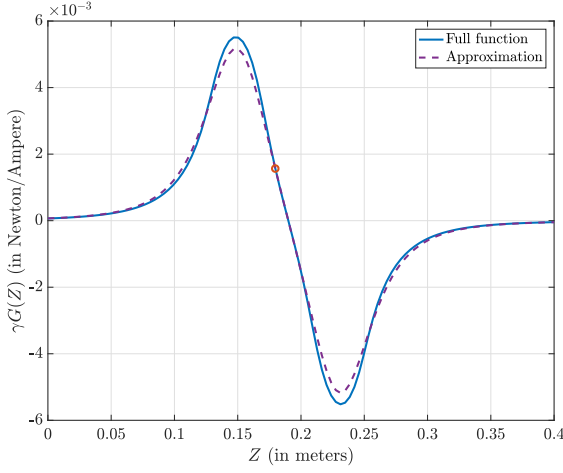
Fig. 3. Function G(Z) (defined in (5)) and its approximation G_{\text{approx}}(Z) in the far field of the magnet (defined in (6)). The circle denotes the value G(\bar{Z}) at the rest position \bar{Z} = 0.18 . The values used for the rest of the parameters are taken from the table found in the appendix of [2].
