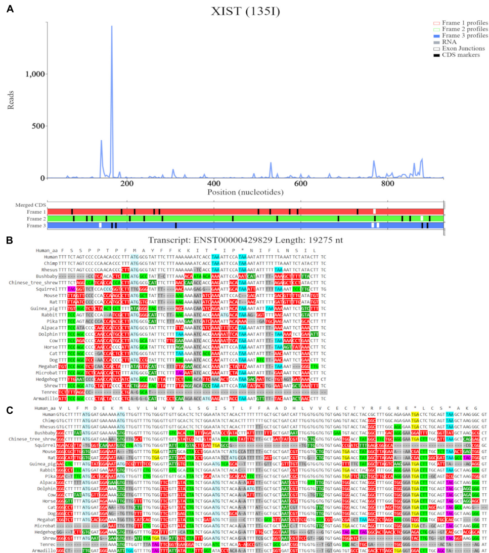
FIGURE 9 | Visualization of XIST in Trips-Viz and CodAlignView. (A) Visualization of transcript ENST00000429829 without RNA-seq data enabled and only reading frame 3 enabled. (B) CodAlignView for the ORF previously outlined in blue showing predominantly absolute codon conservation. (C) CodAlignView for the ORF previously outlined in orange showing mostly absolute codon conservation, there are also more radical non-synonymous codon substitutions than synonymous substitutions.
