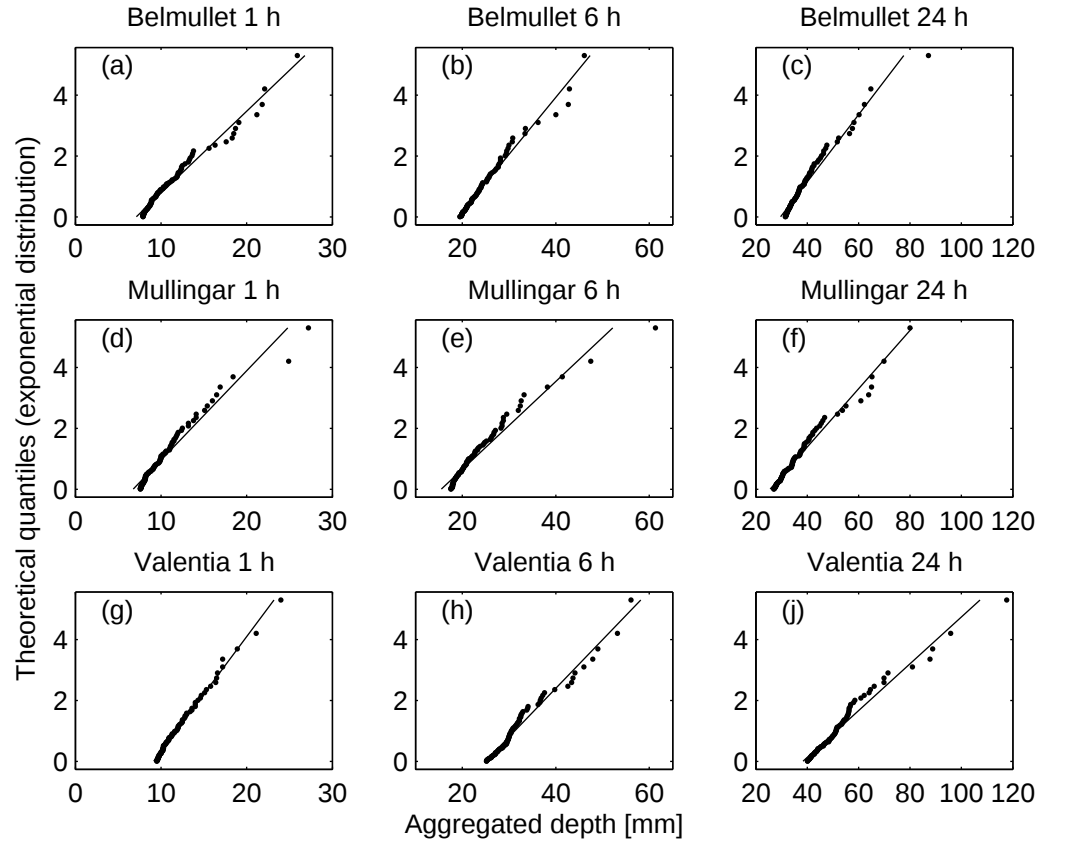
Figure 3: Q-Q plots of quantiles derived from an exponential distribution ( \xi = 0 ) against empirical extrema observed at Belmullet, Mullingar and Valentia over aggregation levels of 1, 6 and 24 hours.
