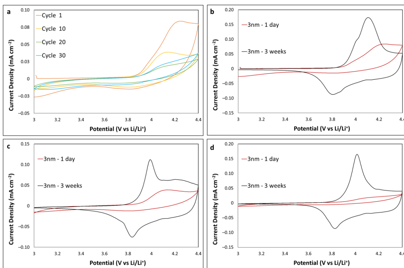
Figure 4. CV profiles of 3 nm \text{Al}_2\text{O}_3 -coated LCO at 0.2 \text{ mV s}^{-1} (a) 1-day air exposure (cycle 1 to 30), (b) 1-day vs. 3-week air exposure (cycle 1), (c) 1-day vs. 3-week air exposure (cycle 10) and (d) 1-day vs. 3-week air exposure (cycle 20).
