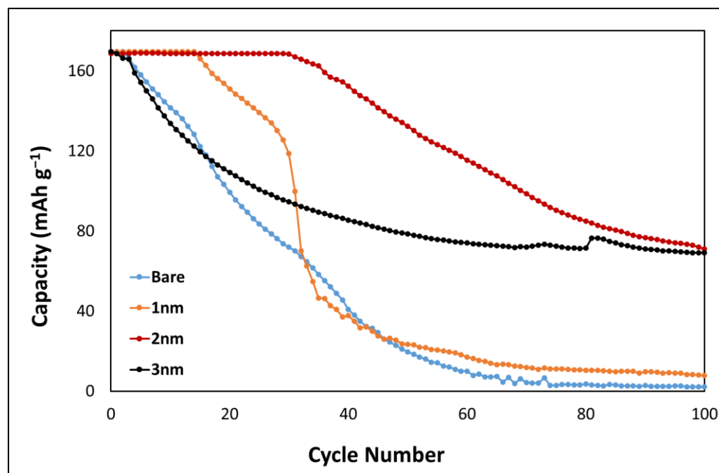
Figure 2. Discharge profiles of bare, 1, 2 and 3 nm coated \text{Al}_2\text{O}_3 at LCO at 63 \mu\text{A}/\text{cm}^2 .
