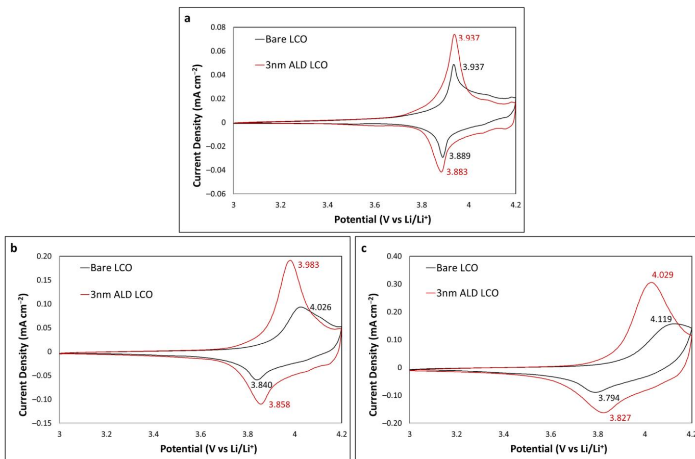
Figure 1. CV profiles of bare and 3 nm \text{Al}_2\text{O}_3 -coated LCO at (a) 0.05 \text{ mV s}^{-1} (cycle 10); (b) 0.2 \text{ mV s}^{-1} (cycle 40); and (c) 0.5 \text{ mV s}^{-1} (cycle 70).
