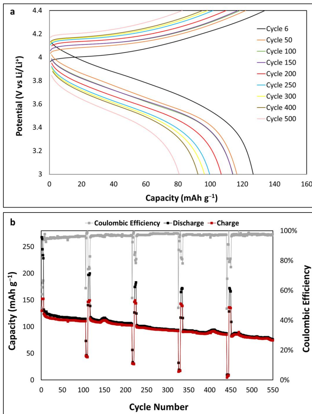
Figure 5. (a) Discharge profile of 3 nm \text{Al}_2\text{O}_3 -coated LCO and (b) the measured capacity and coulombic efficiency.
