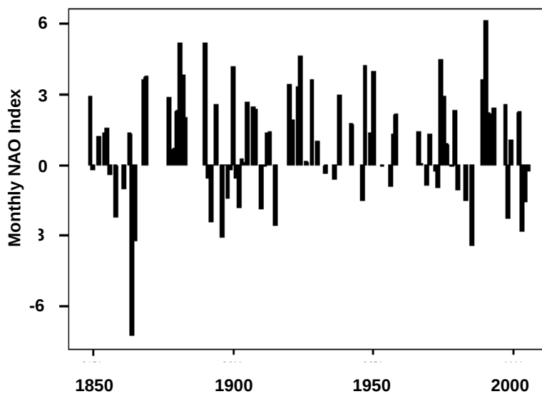
Figure 3. North Atlantic Oscillation (NAO) Values 1849-2008 corresponding to recorded flood events in the historical flood database
