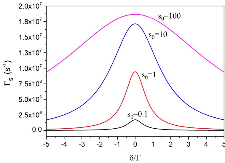
Figure 3.2: Scattering rate for the 5 S_{1/2} F=2 \rightarrow 5 P_{3/2} F'=3 transition of ^{87}\text{Rb} ( \Gamma/2\pi = 6 MHz) as a function of \delta/\Gamma .
