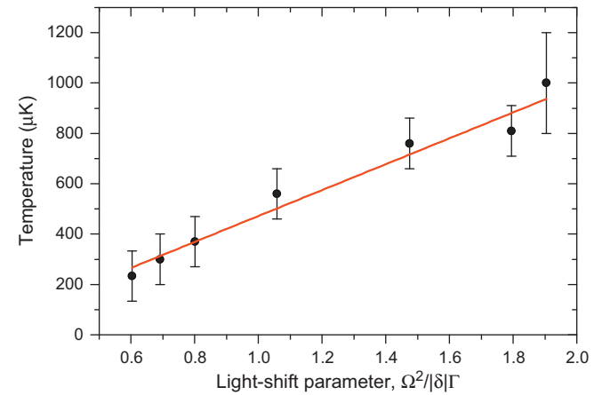
Fig. 5. Temperature of the cloud as measured with RR plotted against the dimensionless light-shift parameter \Omega^2/|\delta|\Gamma (black circles) and a linear fit (red solid line) to the data. (For interpretation of the references to color in this figure caption, the reader is referred to the web version of this article.)
