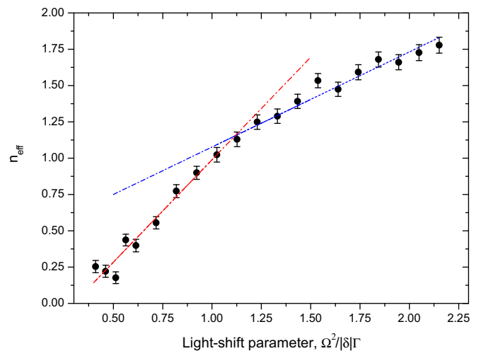
Fig. 7. Estimation of effective atom-number, n_{eff} , with increasing dimensionless light-shift parameter \Omega^2/|\delta|\Gamma (black circles) with two linear fits to indicate the change in slope around a light-shift parameter 1.2.
