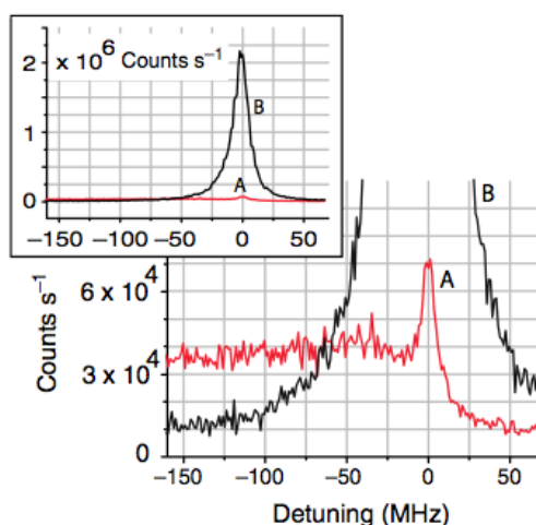
Figure 5. Laser induced fluorescence spectra from Cs measured through an optical nanofiber for the closed-cycle transition, 6S F = 4 \leftrightarrow 6P F = 5 . Traces A and B correspond to without and with the effect of violet laser irradiation, respectively. The violet irradiation was used to remove Cs that had adhered to the surface of the fiber. Reprinted with permission from [58]. Copyright 2008 Institute of Physics.
