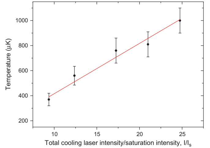
Fig. 4. Temperature as a function of cooling laser intensity normalised to the saturation intensity, I_s ( \delta = -2\Gamma ). The solid red line is a linear fit to the experimental data. (For interpretation of the references to color in this figure caption, the reader is referred to the web version of this article.)
