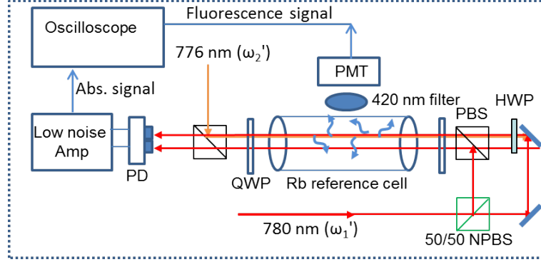
Figure 3. Vapor cell spectroscopy for two-photon excitation with \omega'_1 locked and \omega'_2 in scan mode. Counter-propagating \omega'_1 and \omega'_2 beams excite the atoms to 5D_{5/2} F'' states. This is detected either by monitoring the blue photons on the photomultiplier tube (PMT) or the absorption of \omega'_1 on a photodiode. QWP: quarter waveplate, NPBS: non-polarizing 50-50 beamsplitter, PD: photo detector, PMT: photo multiplier tube.
