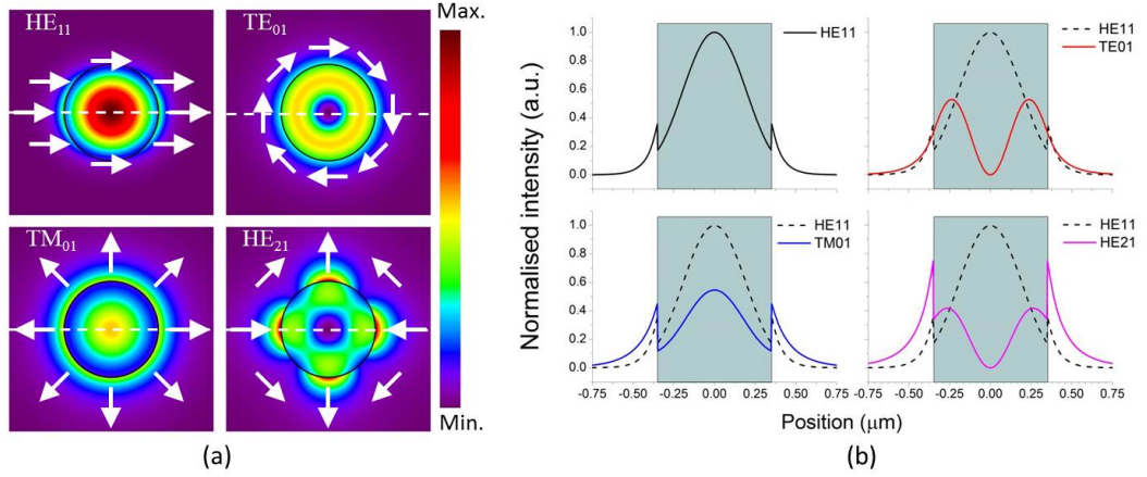
Figure 8.1: (a) Intensity distribution of the first four fibre modes ( HE_{11} , TE_{01} , TM_{01} , and HE_{21} ) of a nanofibre (radius 350 nm) for 780 nm light. Refractive indices of the nanofibre material and the surrounding medium are taken as 1.456 and 1 respectively. Black circles denote the nanofibre boundary. Arrows denote the polarisation of the light fields. The amount of power in each mode is identical and the four plots are normalised to the maximum intensity in the HE_{11} mode. (b) Intensity profile along the white dashed line in figure (a) with the zero position at the fibre axis. The shaded region denotes the fibre. The intensities are normalised to the maximum intensity in the HE_{11} mode. The profile of the HE_{11} mode is plotted along with the other modes for ease of comparison.
