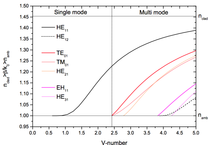
Figure 2. A plot of the effective index of refraction, n_{eff} = \beta/k_0 , against V-number for an optical fiber with cladding and core refractive indices as 1.4537 and 1.000, respectively. \beta represents the propagation constant. The vertical line indicates the boundary between single- and multimode guidance in the fiber ( V = 2.405 ).
