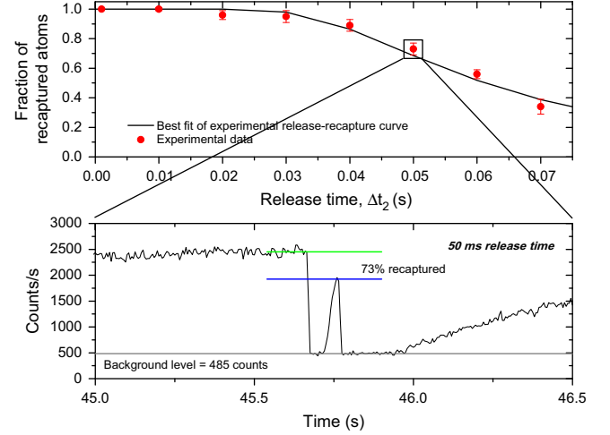
Figure 3. Fraction of recaptured atoms estimated from the fluorescence data obtained from an optical nanofibre placed near the cold cloud of atoms. For a release time, \Delta t_2 , of 50 ms, 73% of the expanded cloud was recaptured with \delta = -2.6\Gamma and cooling laser intensity of 2.9I_s ( 4.6 \text{ mW/cm}^2 ) per beam.
