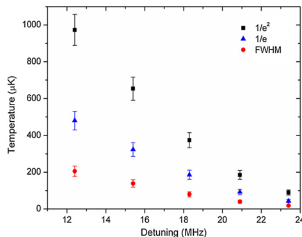
Figure 7. Atom cloud temperature as a function of detuning of the cooling laser beams for three standard definitions of cloud radius. The measurements were made using the forced oscillation technique and indicate that sub-Doppler temperatures <144\ \mu\text{K} can be achieved in the presence of an ONF. Reprinted with permission from [3]. Copyright 2012 Institute of Physics.
