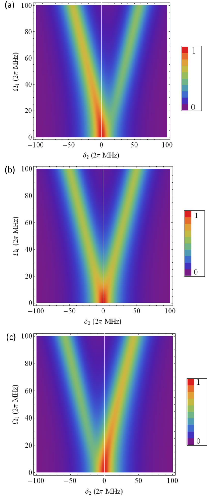
Figure 3.4: Calculated absorption spectra showing Autler-Townes splitting with \Omega_2 = 2\pi \times 200 kHz, \Gamma_2 = 2\pi \times 10 MHz and \Gamma_3 = 2\pi \times 20 MHz for the coupling beam ( \omega_1 ): (a) 14 MHz red-detuned from the resonance ( \delta_1 = -14 MHz), (b) at resonance ( \delta_1 = 0 ), and (c) the coupling beam 14 MHz blue-detuned from the resonance ( \delta_1 = +14 MHz).
