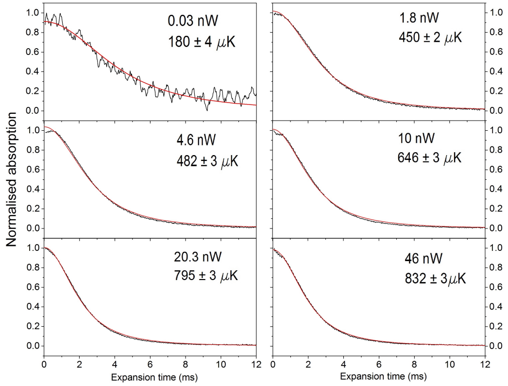
Figure 5.6: Transient absorption with theoretical fits for various probe powers. The corresponding temperature values found from the fits are shown with the standard error obtained from the fitting parameters.
