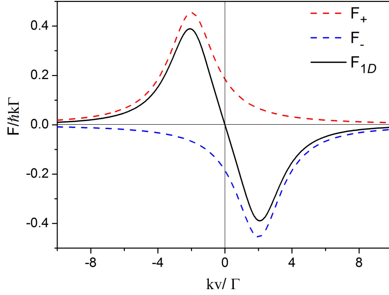
Figure 4.2: Velocity dependence of the damping force in one-dimension for \delta = -2\Gamma and s_0 = 10 . Near v = 0 m/s, the total force on the atom varies linearly with the velocity.
