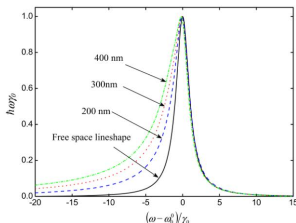
Figure 4. Frequency dependence of the fluorescence power from a Cs cloud coupled into an ONF, including contributions from the van der Waals and the Casimir-Polder effects. For this calculation a cloud radius of 400 nm has been used. The nanofiber radius is varied from 200 nm to 400 nm for the different plots. The solid line shows the expected free space line shape as a comparison. Note that all lines are normalized. Reprinted with permission from [35]. Copyright 2009 Institute of Physics.
