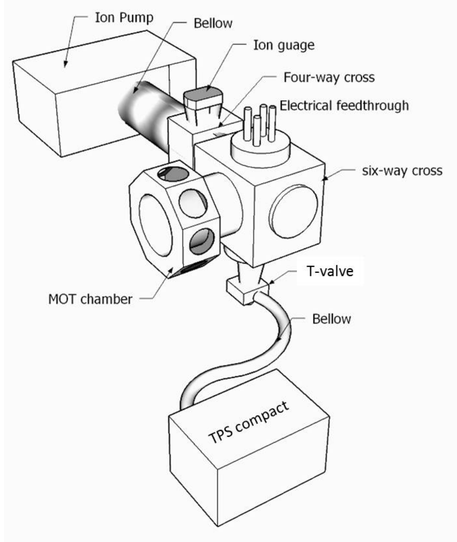
Figure 4.10: Illustration of vacuum components of the experimental setup.
