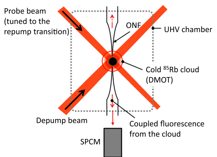
Figure 3. Schematic of the experimental setup. (a) Free-space spectroscopy on the DMOT incorporating a frequency-scanned probe beam, APD: avalanche photodiode, UHV: ultrahigh vacuum. (b) Probing the DMOT with an optical fibre, ONF: optical nanofibre, SPCM: single photon counting module.
