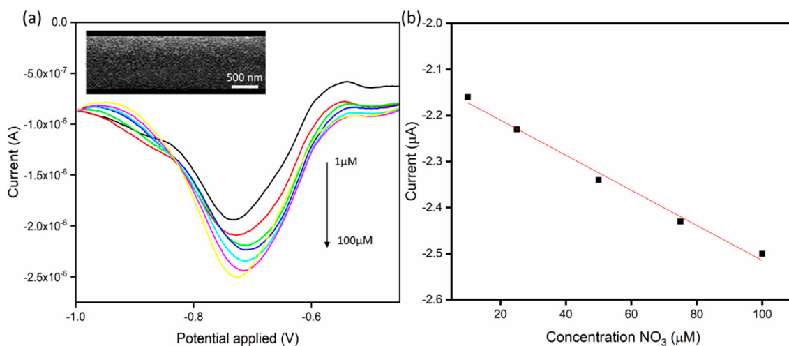
Figure 6. (a) SWV in increasing concentrations of \text{NaNO}_3 in 0.1 \text{ M Na}_2\text{SO}_4 at pH 2. SWV were performed from -0.4 to -1 \text{ V} at 10 \text{ mV/s} with an amplitude of 20 \text{ mV} and a frequency of 20 \text{ Hz} . A SEM image of the copper modified electrode is shown in the top inset. (b) The resultant calibration plot for the SWV measurements
