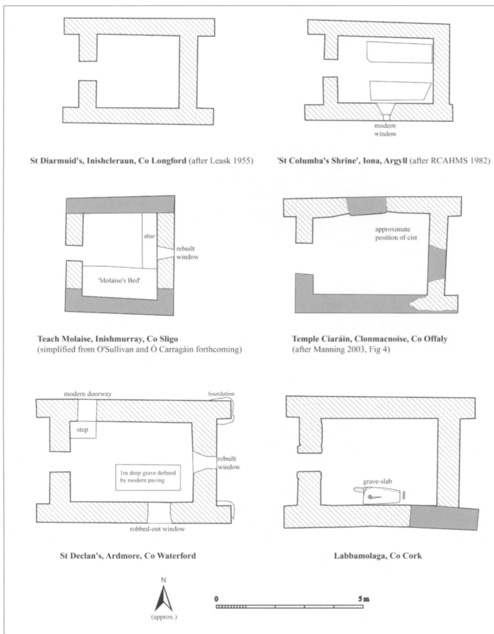
Fig. 1 Plans of six shrine chapels. Grey indicates stretches of wall that have been entirely rebuilt and do not follow the exact line of the original.
