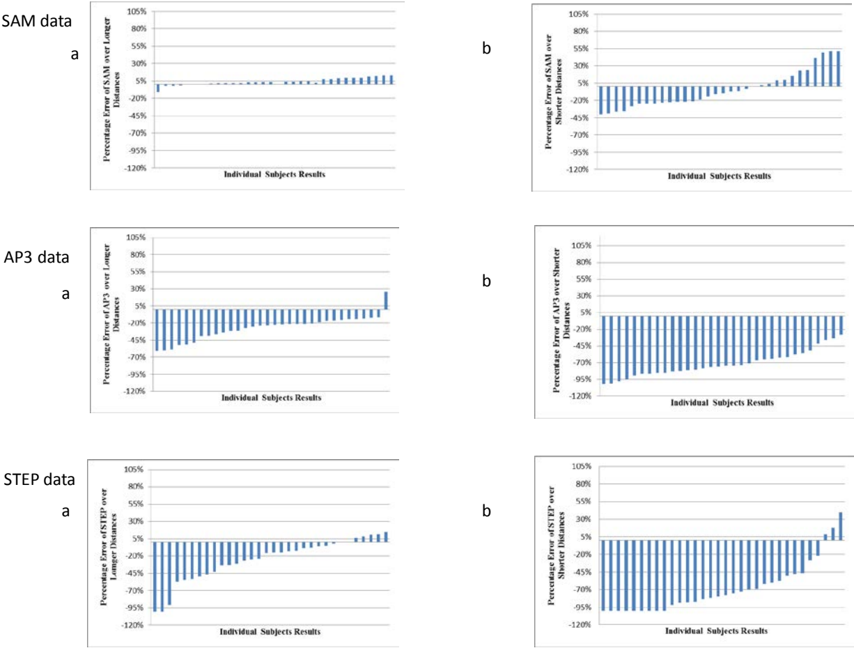
Figure 3.3: Percentage Error of SAM, AP3 and STEP Compared to Video Step-Count over (a) Longer (over 5 Metres) and (b) Shorter Distances (5 Metres or Less)
