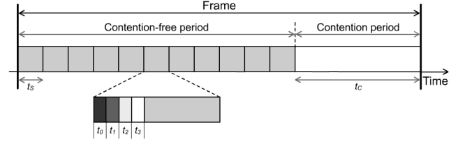
Figure 1: ER-MAC's frame structure
