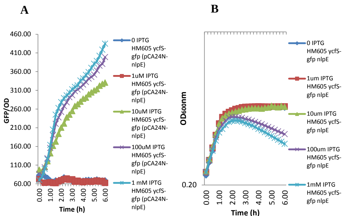
Figure 4.16: Activation of Cpx pathway in HM605 ycfS -gfp (pCA24N- nlpE ) using various concentrations of IPTG A) GFP/OD600 showing the levels of GFP expression. The expression of ycfS is significantly up-regulated at IPTG concentrations above 1 μM. Results are expressed as the amount of GFP expressed relative to growth (GFP/OD). B) Growth of all strains in LB with various concentrations of IPTG. 10 μM was the only concentration that activated the pathway but didn't affect growth. Each strain was represented by 3 individual cultures.
