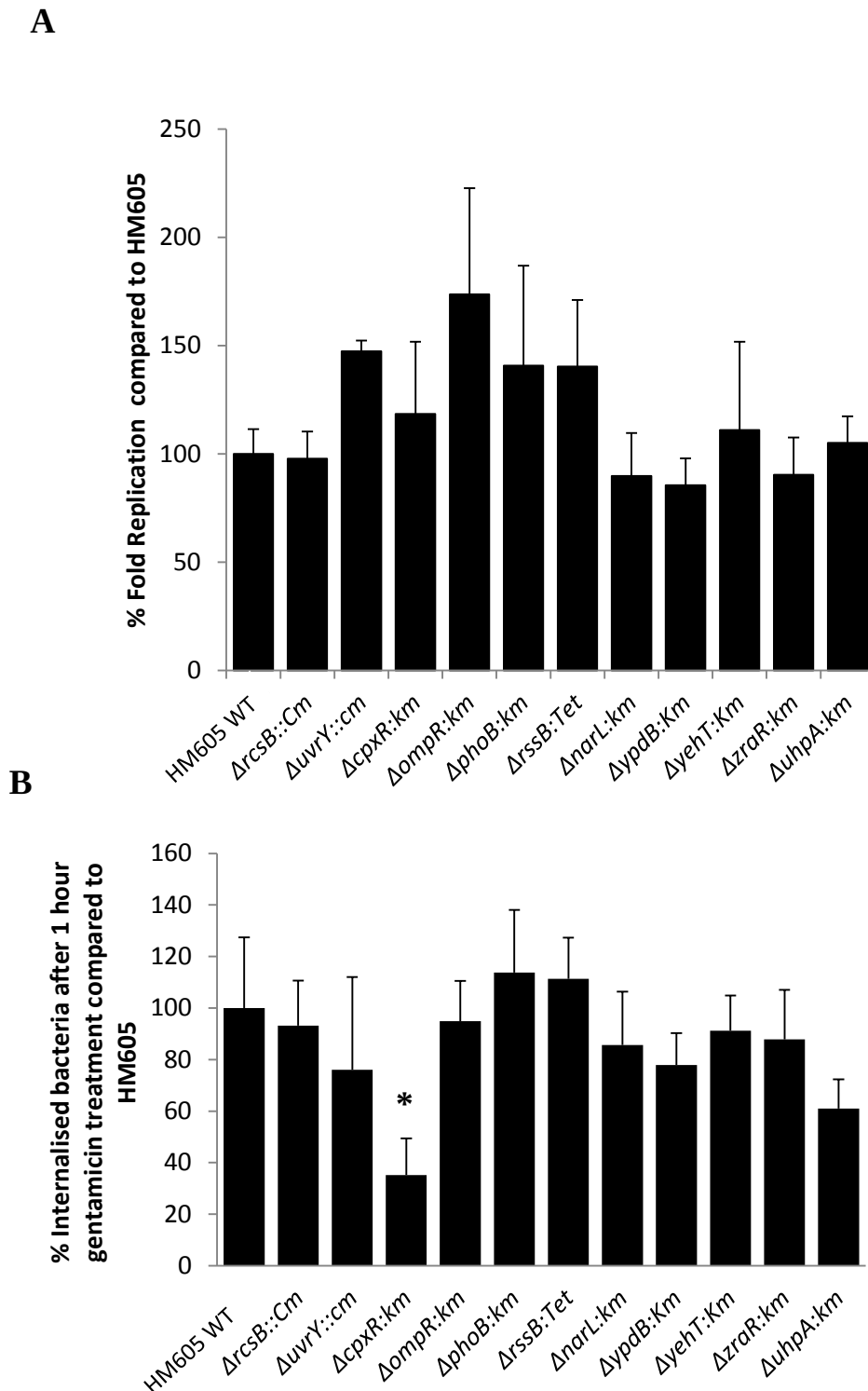
Figure 4.2: 11 response regulator mutants HM605 are examined for their ability to replicate in J774.A1 macrophages.
