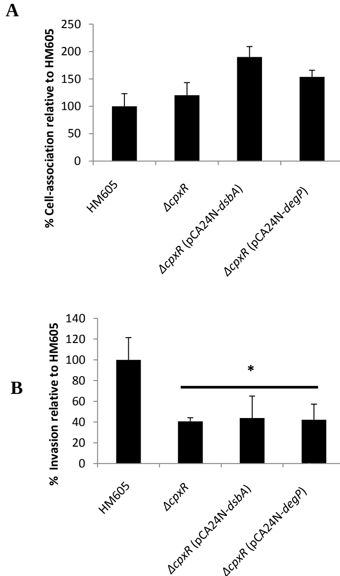
Figure 4.15: Phenotype of HM605 \Delta cpxR (pCA24N-dsbA) and HM605 \Delta cpxR (pCA24N-degP) in C2Bbe1 epithelial cells. (A) Adhesion to C2Bbe1 epithelial cells. Cell-associated bacteria were quantified after a 3-h infection period. The results are expressed as levels of cell-associated bacteria (adherent plus intracellular) relative to those obtained for wild-type strain HM605, taken as 100%. (B) Bacterial invasion of C2Bbe1 epithelial cells was determined after gentamicin treatment for an additional 1 h. Overproduction of DsbA and DegP in the cpxR mutant did not restore the invasion phenotype. The results are expressed as levels of intracellular bacteria/associated bacteria relative to those obtained for wild-type strain HM605, taken as 100%. For analysis of the significance of differences in association and invasion into C2Bbe1 epithelial cells, Student's t-test was used for comparison of two groups of data (* P-value \leq 0.05 ).
