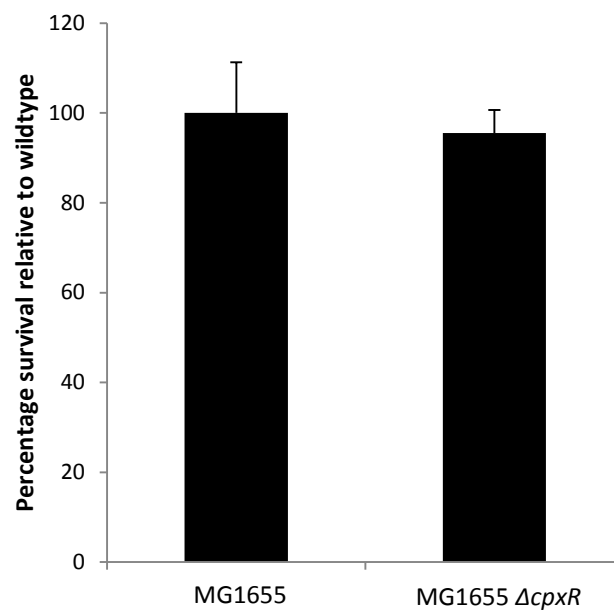
Figure 4.18: Acid challenge. The graph represents the mean results of 3 cultures per strain replicated in triplicate. HM605 \Delta cpxR is more tolerant to low pH than the wildtype. No differences were observed between MG1655 and MG1655 \Delta cpxR . For analysis of the significance of differences in numbers, Student's t-test was used for comparison of two groups of data (* P-value \leq 0.05 ).
