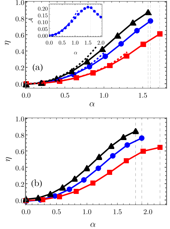
FIG. 4. Efficiency \eta vs \alpha with \Delta_0 = 0.5 (solid black), \Delta_0 = 1.0 (solid blue), and \Delta_0 = 2.0 (solid red); the dotted vertical lines denote the critical SOC strength \alpha_c(g, \Delta_0) . (a) g = 0 . Inset: Total work \mathcal{A} vs \alpha with \Delta_0 = 1.0 ; results based on perturbation theory in Eq. (15) (blue, red, and black dashed lines). (b) g = -1 .
