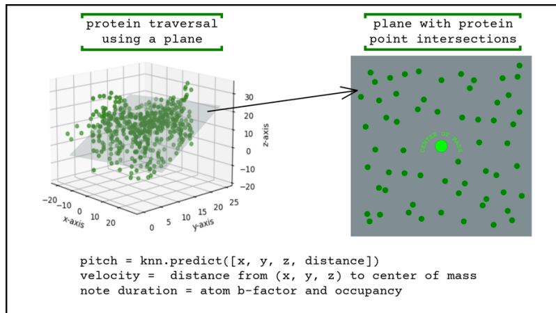
Figure 2. Protein Point Plane Traversal.
