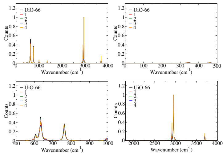
Figure S8: Raman spectra of non-defective UiO-66 with 1–4 linkers removed with acetic acid capping.
