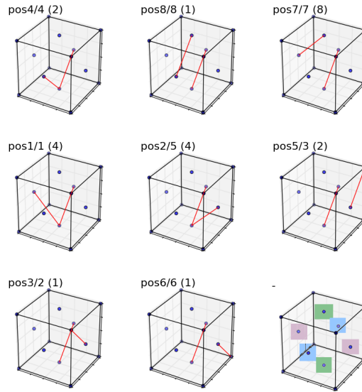
Figure S3: Configurations for 2 vacant BDC linkers. Red lines represent the missing linkers with the names of the configurations corresponding to those plotted in Figure 2 for the acetate/ \text{Cl}^- / \text{H}_2\text{O} capping mechanisms, respectively. Configurations are numbered in order of defect energy magnitude and therefore differ for either capping mechanism. In brackets is the degeneracy of configuration used to calculate the Boltzmann distributions. There are 4 metal nodes in the cubic unit-cell, individual metal nodes are highlighted as green, blue and pink with all 8 corners of the plotted cubic cell making the fourth metal node.
