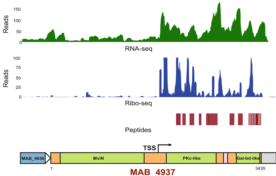
Fig. 2 Domain based alternate isoforms of MviN predicted in M. abscessus driven by an internal TSS. Presence of isoform is evidenced by a combination of RNA-Seq, Ribo-seq and LC-MS peptide data downstream of the internal TSS
