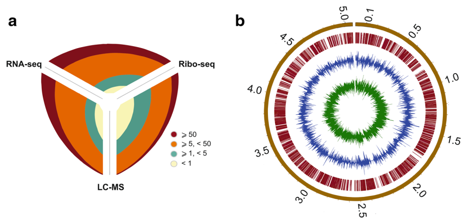
Fig. 1 An integrated approach combining RNA-seq/Ribo-seq and Proteomics identifies the coding potential of M. abscessus . a The breakdown of identified CDSs in MAB using the integrated data map represented as a hive plot. In the inset, expression values are given in color-coded RPKM or peptide counts. b Circos image of normalized whole-genome depth of coverage of RNA-seq (green), Ribo-seq (blue) and mass spectrometry (red) data. To aid visualisation, RNA-seq and Ribo-seq expression values are given on logarithmic scale (RPKM values < 1 are assigned a value of 0)
