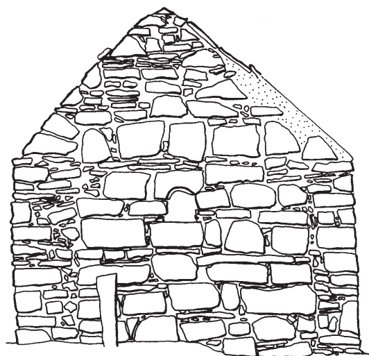
East Elevation
