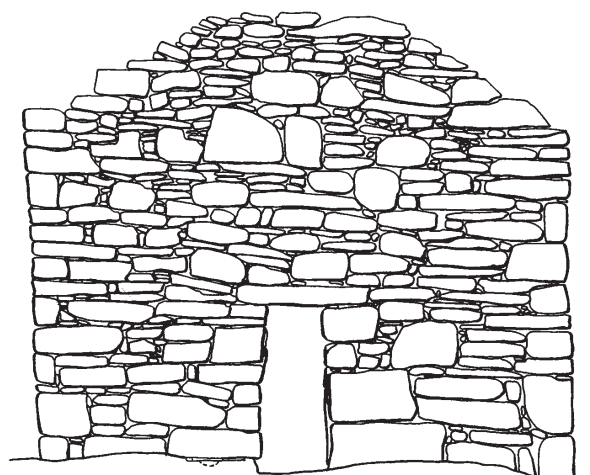
West Elevation
