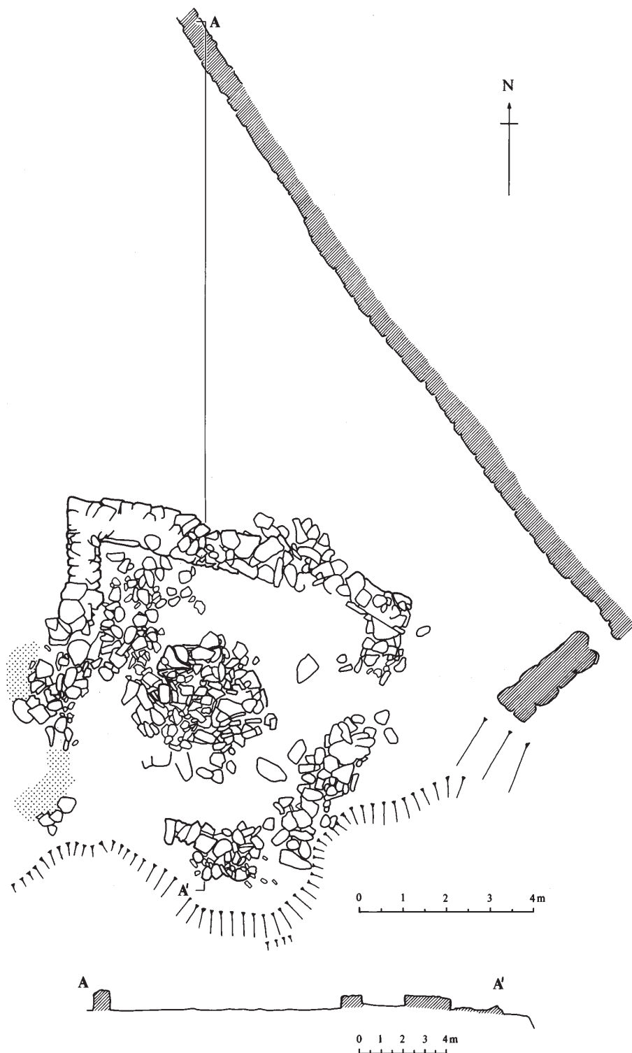
Figure 36 Ollamurray: survey plan (1998) of the leacht and eroding cliff-edge
