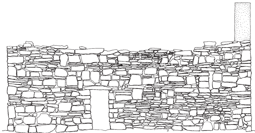
South Elevation
