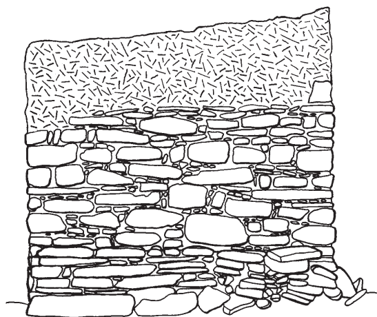
South Elevation
