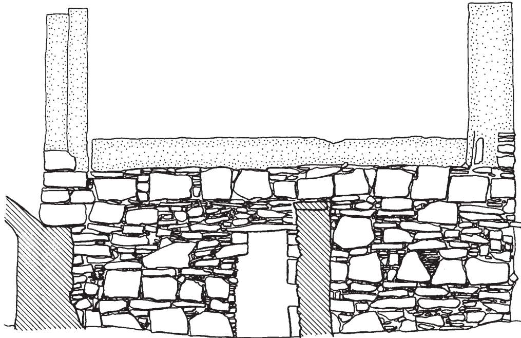
South Elevation
