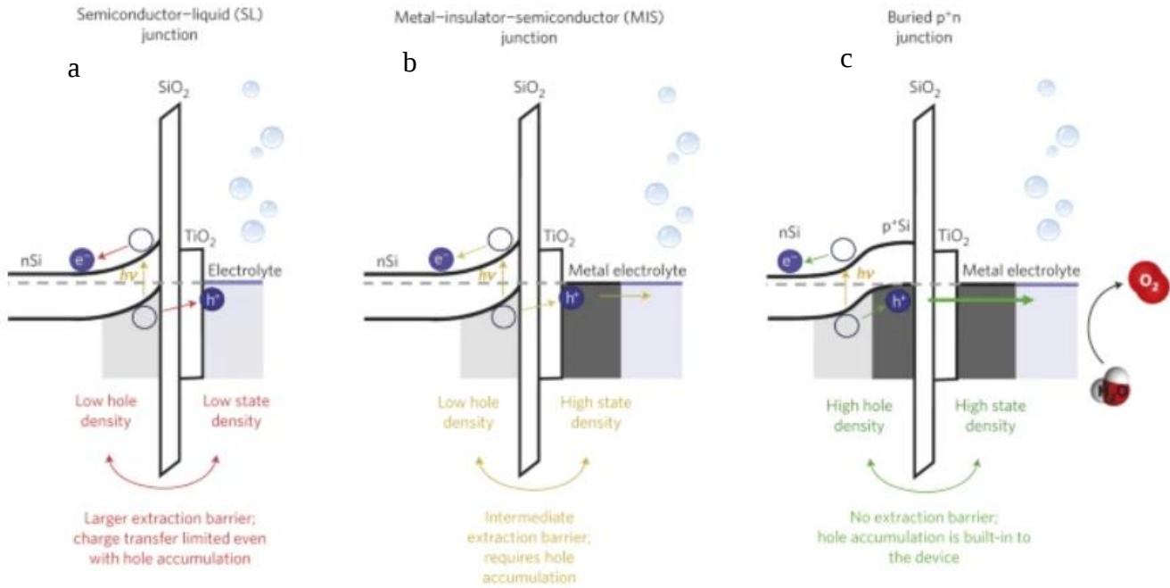
Figure 1.10: Schematic of different types of n type semiconductor in contact with a redox electrolyte each protected with a \text{TiO}_2 protective layer. (a) Regular semiconductor/liquid interface. A low density of holes is present at the interface due to the absence of a metal catalyst. (b) A metal-insulator-semiconductor device which increases density of states at the interface due to the catalyst present at the surface but is limited by the thickness of protective/catalyst layers blocking illumination. (c) buried p+n junction device where the p+ region ensures a high density of holes at the interface regardless of illumination thus greatly reducing the extraction barrier [58].
