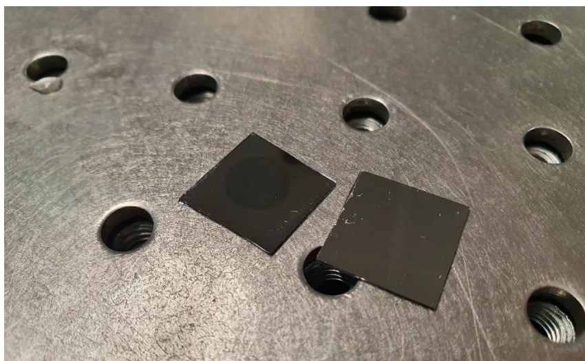
Figure 5.6: a side by side view of the Ni/ \text{TiO}_2 / \text{SiO}_2 /Si anodes used in this work with a used sample on the left and an unused sample on the right. The circle of darker colour seen in the centre of the used sample was the area of contact with the electrolyte during experiments.
