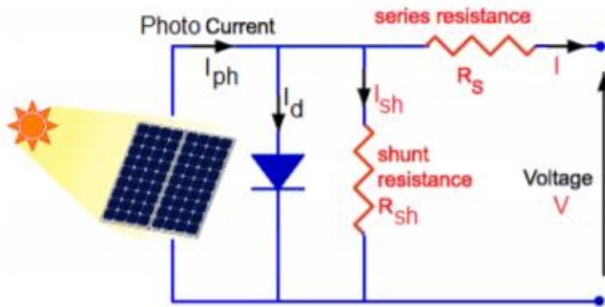
Fig 1.5: Simplified circuit diagram of a typical solar cell [16]
