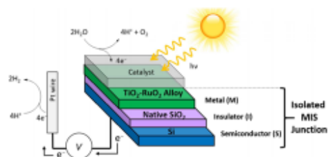
Photoanode using the isolated MIS structure
