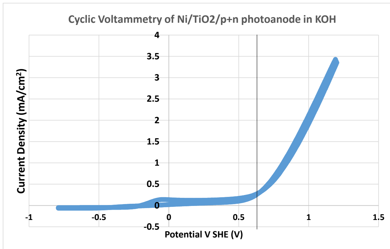
Figure 5.11: KOH cyclic voltammetry response for a Ni/TiO 2 /SiO 2 /p+n-Si sample showing the water oxidation curve. The calculated oxidation potential of water at this pH is \sim 0.6 V. The black line is located at this E_{O_2} potential.
