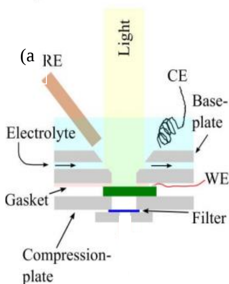
Figure 3.1: (a) a schematic cross-sectioned view of the PTFE cell used in this work. (b) Photograph of the cell setup within the lab in this instance with a high powered LED on top.
