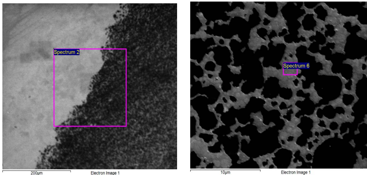
Figure 5.7: SEM images of a used Ni/TiO 2 /Si anode; (a) the border region of the area under test (b) higher magnification view of the surface of a photoanode after CA experiments.
