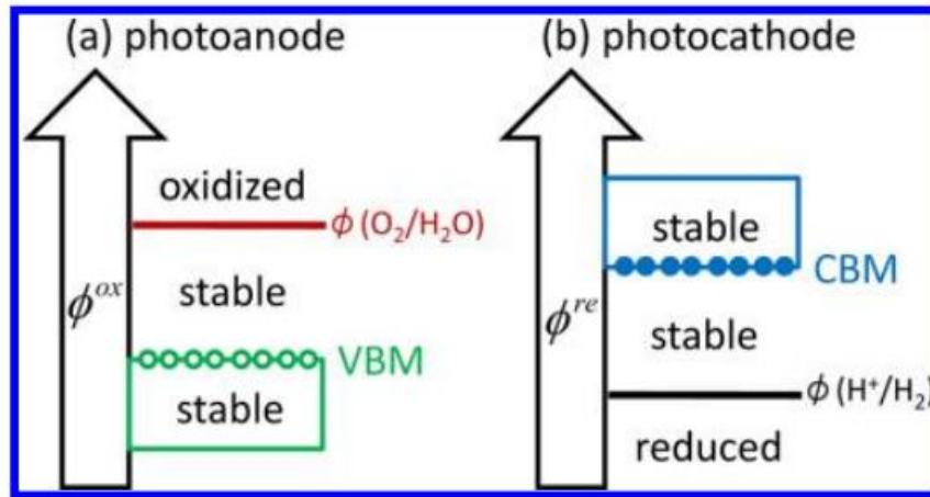
Figure 1.8: Diagram showing (a) how the stability of a photoanode will decrease as its oxidation potential shifts from its VBM (valance band maximum) to the water oxidation potential \phi(O_2/H_2O) and (b) how the stability of a photocathode will decrease as its reduction potential shifts from its CBM (conduction band minimum) to the water reduction potential \phi(H^+/H_2) [96]
