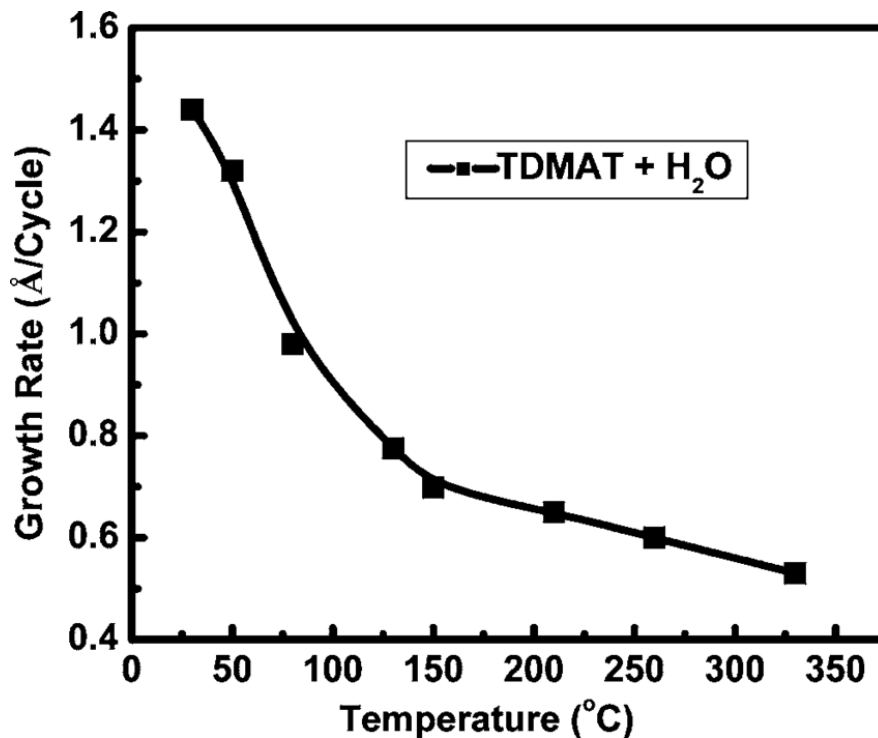
Figure 2.3: GPC of \text{TiO}_2 deposited using TDMAT and \text{H}_2\text{O} as a function of deposition temperatures. [37]
