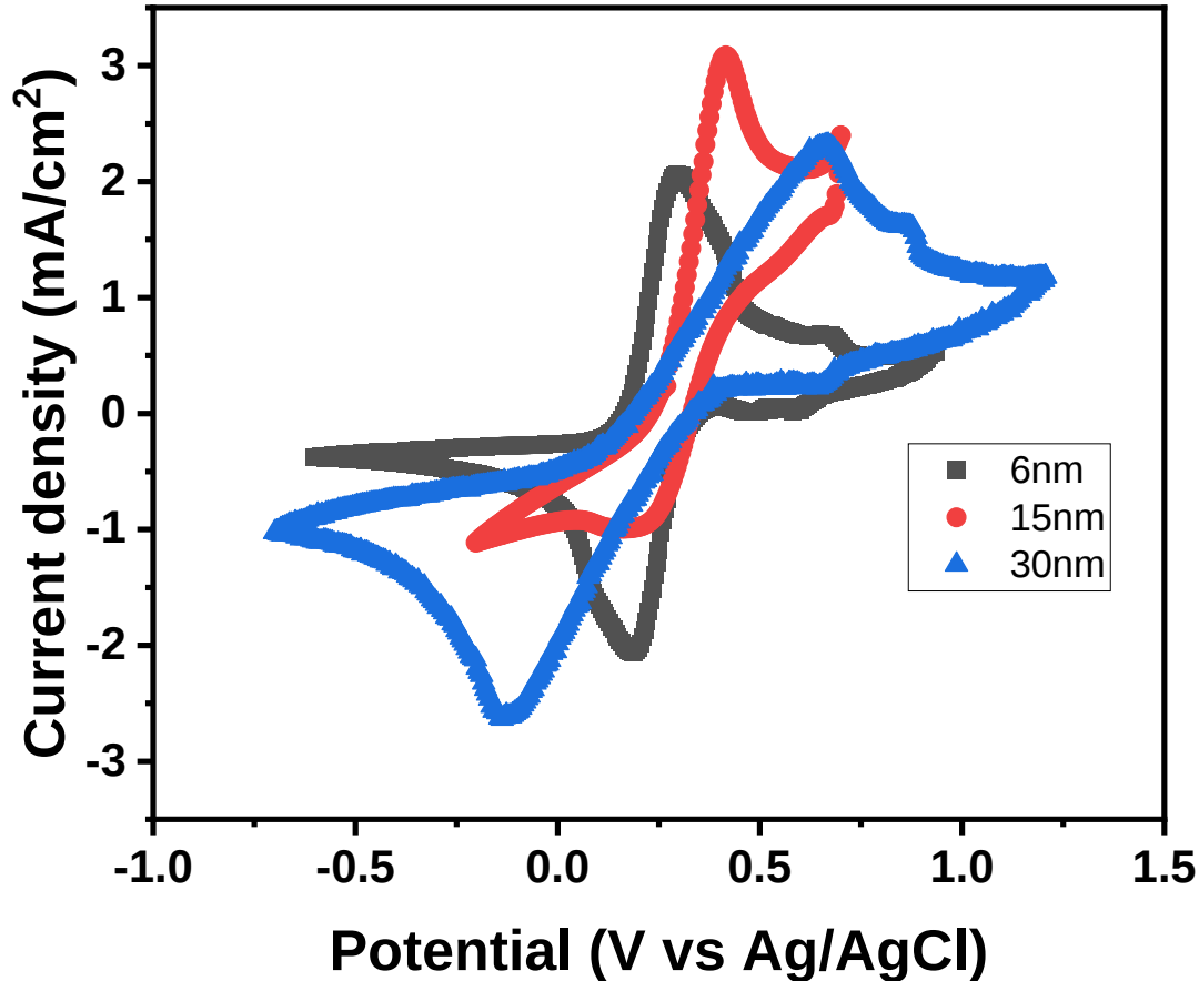
Figure 5.3: Ferri/ferrocyanide response for a \text{Ni}/\text{TiO}_2/\text{SiO}_2/\text{p}^{++}\text{-Si} sample in the dark showing the peak to peak voltage dependence on protective layer thickness.
