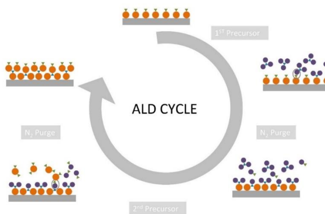
Figure 2.1 Schematic of the full ALD cycle including the surface reactions and precursor pulse [36]
