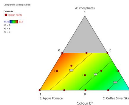
Figure 3-4: Contour plots of instrumental colour parameters L* (a), a* (b) & b* (c).
