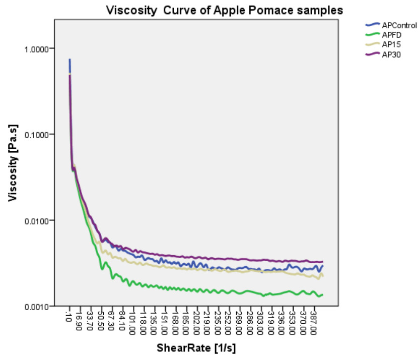
Figure 4-1: Viscosity curve of the apple pomace ingredient obtained from high-speed homogenisation using Anton Paar rheometer.
