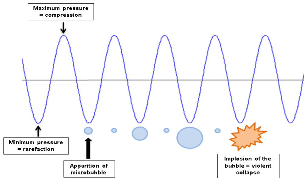
Figure 1-5: Schematic representation of cavitation produced by direct field pressure from US probe.
