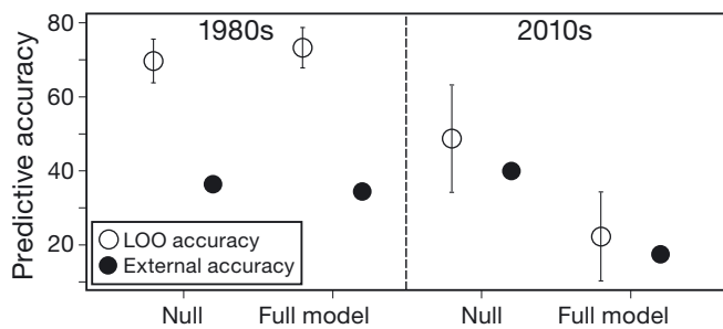
Fig. 5. Predictive accuracy (%) of null models (fit with latitude and longitude only) and full models of clan identity of sperm whales off the Galápagos Islands in the 1980s (1987 and 1989) and 2010s (2013 and 2014). Predictive accuracy was measured through leave-one-out (LOO) and external cross-validation. Standard errors are shown for LOO accuracy
