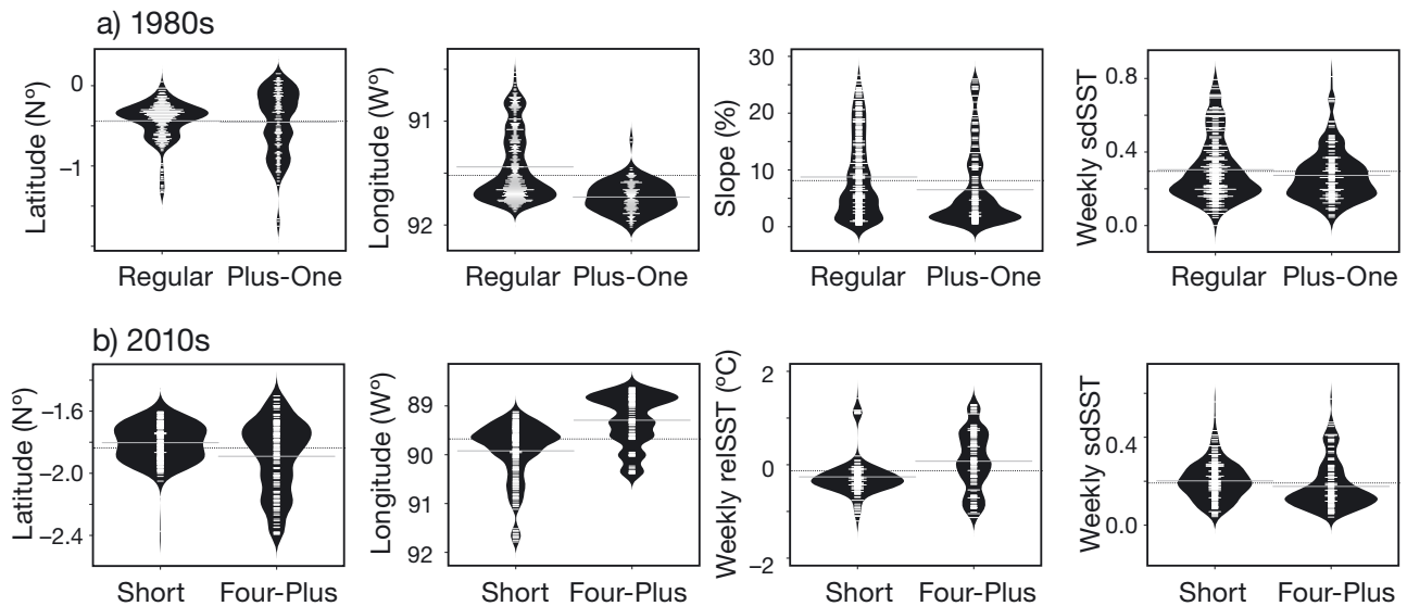
Fig. 3. Observed geographic and oceanographic variables by clan. (a) 1980s distribution of variables in which Plus-One and Regular clan whales were found off the Galápagos Islands: latitude, longitude, slope incline, and weekly standard deviation of sea surface temperature (sdSST). (b) 2010s distribution of variables in which Four-Plus and Short clan sperm whales were found: latitude, longitude, weekly relative mean SST (relSST), and weekly sdSST. Clan types are defined in Fig. 1
