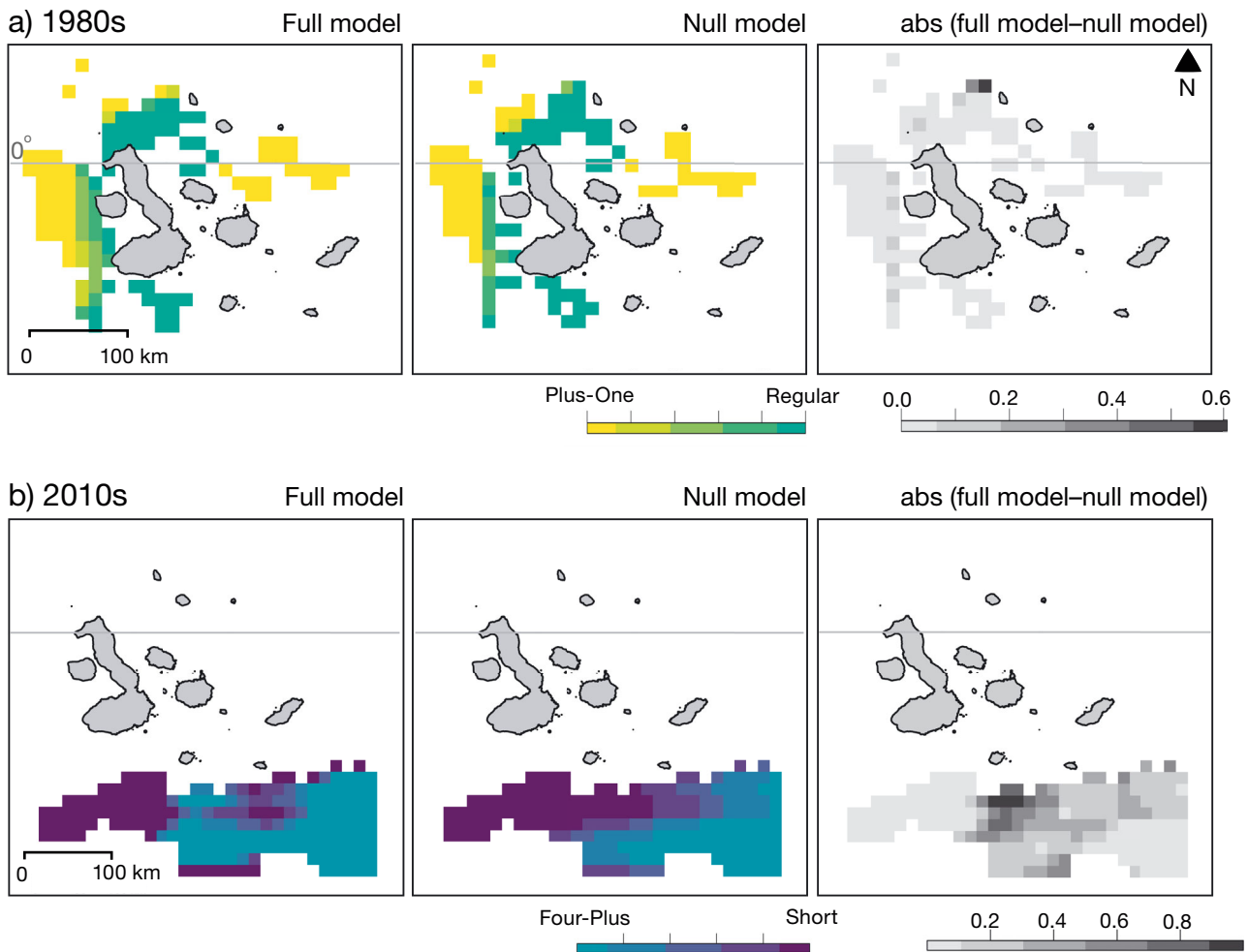
Fig. 4. Predicted probability of sperm whales belonging to different clans off the Galápagos Islands mapped at 0.12^\circ resolution. (a) Sperm whales of the Plus-One and Regular clans in 1987 and 1989 as a function of the full model, the null model (latitude and longitude only), and the absolute difference between the full and null models. (b) Sperm whales of the Short and Four-Plus clans in 2013 and 2014 as a function of the full model, the null model (latitude and longitude only), and the absolute difference between the full and null models. Clan types are defined in Fig. 1
