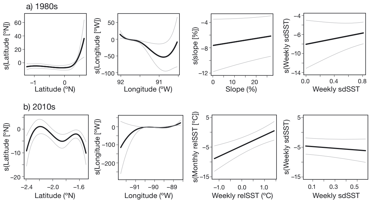
Fig. 2. Partial plots of \log_e(\text{odds}) of female and juvenile sperm whales found off the Galápagos Islands belonging to (a) the Plus-One clan in the 1980s study period and (b) the Four-Plus clan in the 2010s study period. Clan types are defined in Fig. 1. In the 1980s, clan identity = Plus-One is modelled as a function of latitude, longitude, slope incline, and weekly standard deviation of SST (sdSST). In the 2010s, clan identity = Four-Plus is modelled as a function of latitude, longitude, weekly relative mean SST (relSST), and weekly sdSST. Grey lines represent 95 % confidence intervals
