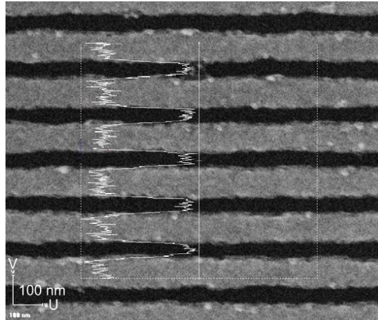
Figure 1.7. Line and space pattern: 90 nm wide gold lines on a SiO 2 substrate spaced 70 nm apart (80 nm half-pitch), structured with the after lift-off process. The sample was developed for 60 s in a developer diluted with 40 % vol. DI water. 30
