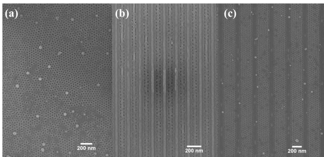
Figure 5.9. SEM images of a Ge surface treated with 1 M citric acid prior to BCP processing. DSA of the PEO cylinders in (a) open area showing PEO cylinders, (b) a 135 nm HSQ trench and (c) a 270 nm HSQ trench.
