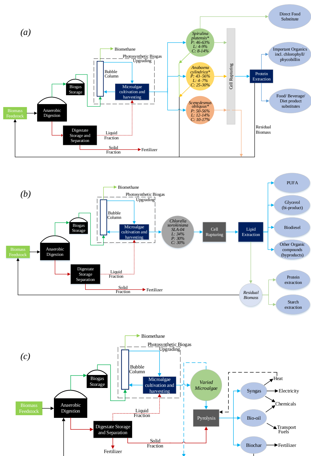
Figure 6-5 Cascading Algal Biomethane Biorefinery System (CABBS) (a) with protein-rich microalgae for photosynthetic biogas upgrading; (b) with lipid-rich microalgae for photosynthetic biogas upgrading; (c) integrating pyrolysis with AD systems and photosynthetic biogas upgrading *Microalgae composition obtained from Becker (2007) [85] and Lizzul et al., (2018) [86], where, P is protein, L is lipid and C is carbohydrate
