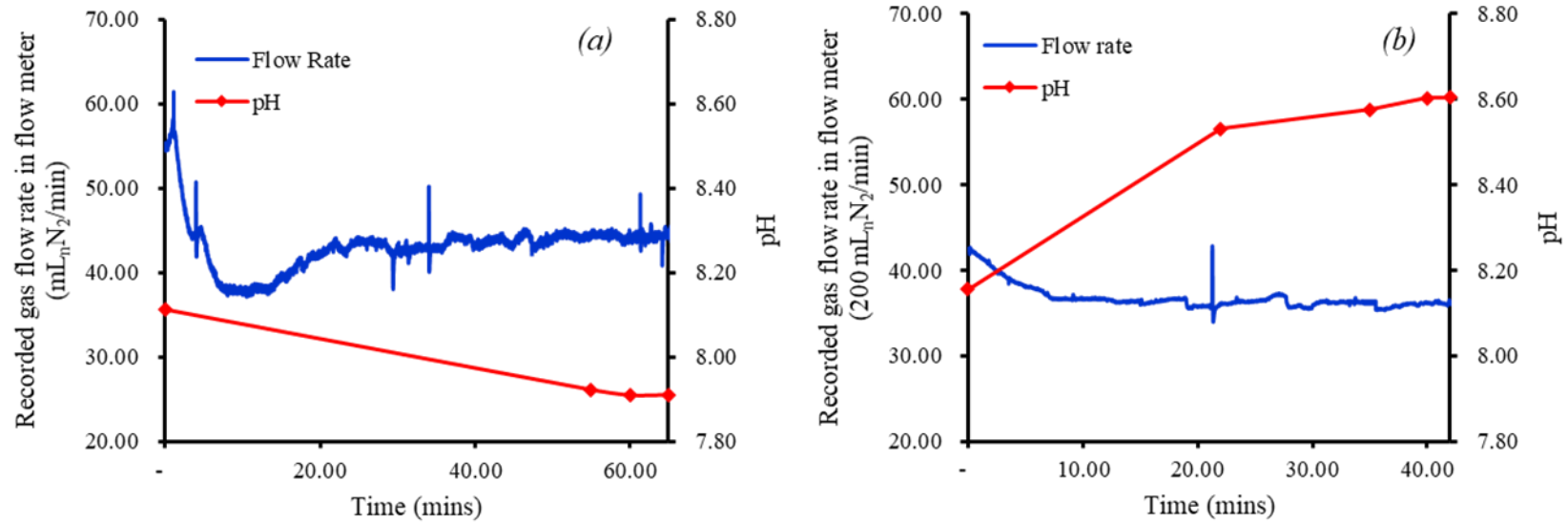
Figure 3-4 Variation in outlet biomethane flow and liquid pH before reaching steady-state. The examples chosen are (a) L/G 0.1 and (b) L/G 0.3 for experiment LON. It is to be noted that, the initial pH for (a) was 8.113, while for (b) it was 8.16 from respective preceding experiments. The data are from the pre-modified setup, chosen for better representation.
