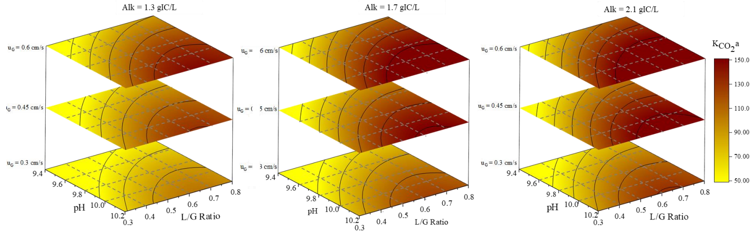
Figure 5-7 Two dimensional contour plots of mass transfer coefficient of CO 2 ( K_{CO_2} a ) versus pH and L/G ratio for at different superficial gas velocities and alkalinity. The contour lines correspond to the values indicated in the legend.
