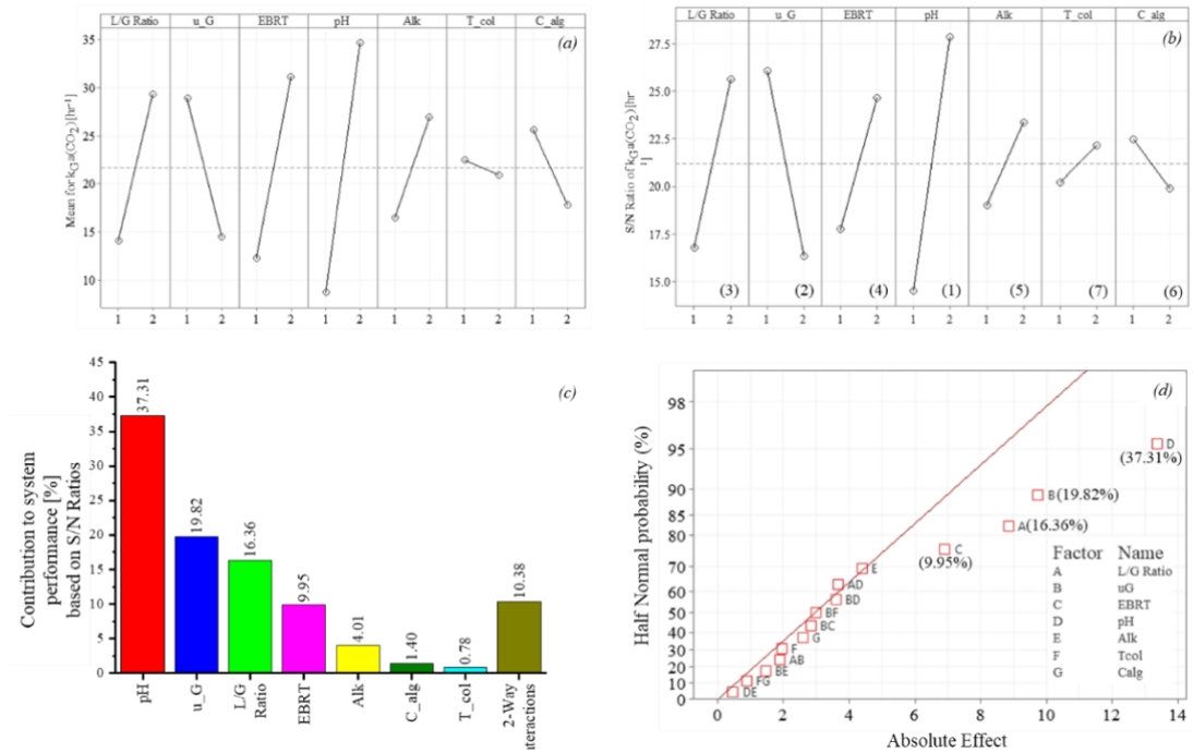
Figure 4-8 Analysis plots for the relative influence of design factors on the gas side volumetric mass transfer coefficient for CO 2 : (a) Main effects plot with means; (b) Main effects plots with S/N ratio. The rank of each design factor is included in parenthesis; (c) Contribution of each design factor and interactions on the overall system outcome; and (d) Half normal probability plot with the relative contribution of major effects highlighted in brackets.
