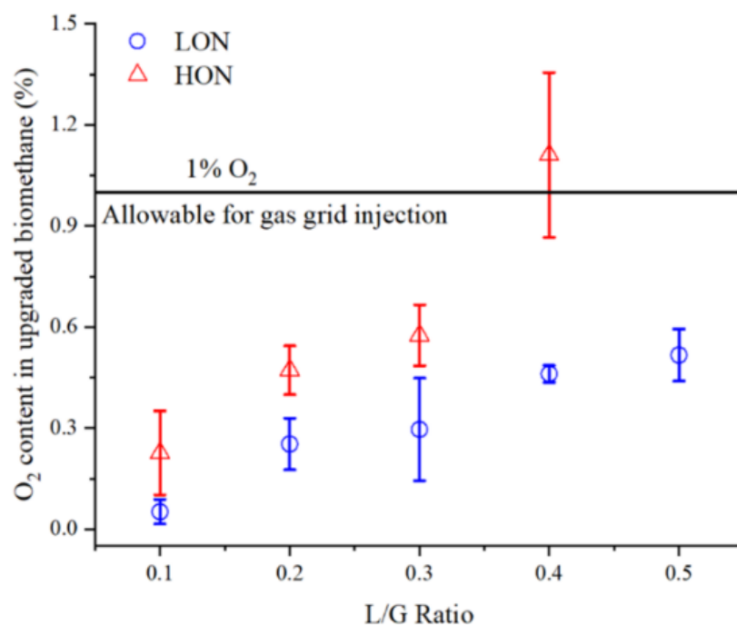
Figure 3-8 Oxygen concentration in the upgraded biomethane under different operating conditions in the lab-scale bubble column
