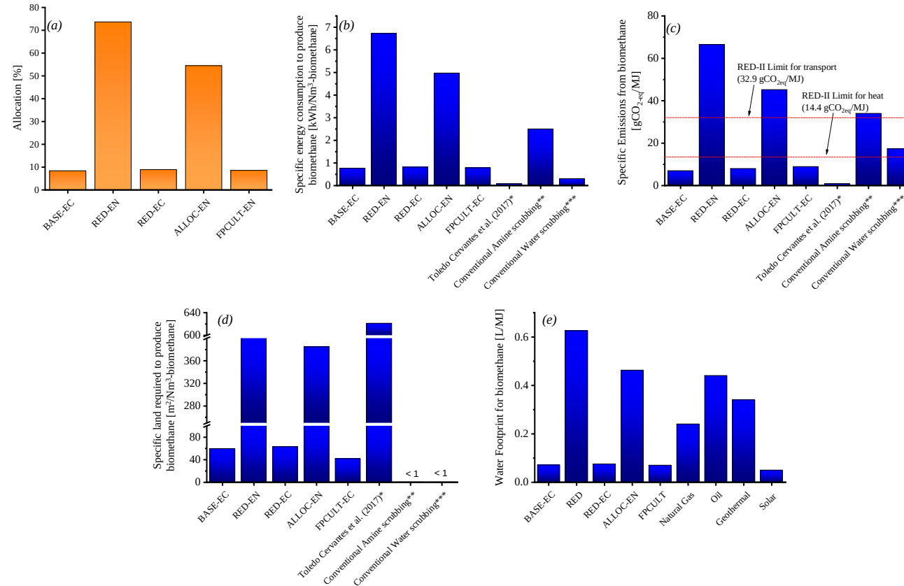
Figure 7-14 (a) Allocation and performance of biomethane based on (b) Specific energy consumed [kWh/Nm 3 -biomethane]; (c) Specific GHG emissions [gCO 2-eq /MJ]; (d) Specific land footprint [m 2 /Nm 3 -biomethane]; and (e) Specific water footprint [L/MJ]. The values of specific water footprint for the production of conventional and renewable energies shown in (e) were compiled from Mekonnen et al. (2015) [135].
