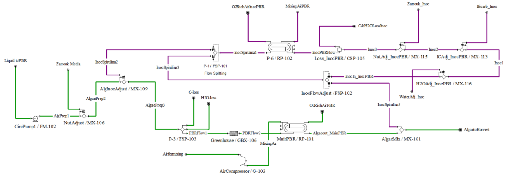
Figure 7-6 Simulated model of the microalgae cultivation section including the inoculum reactor and accessories. The air compressor for circulating air would be necessary only when closed photobioreactors are concerned. However, it has been included in the general model to maintain generality.
