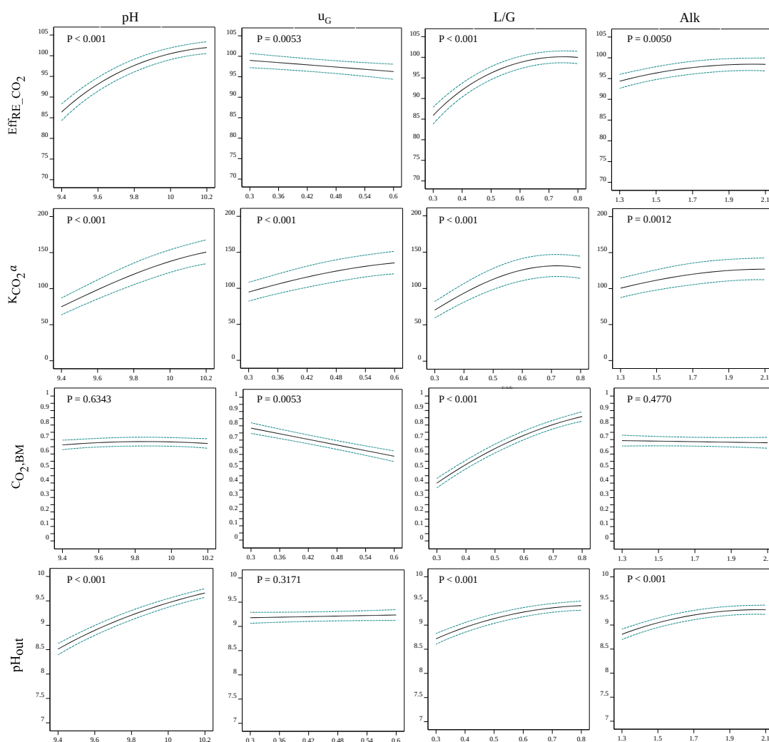
Figure 5-4 Main effects plot of the mean responses of Eff_{RE\_CO_2} , K_{CO_2a} , C_{O_2,BM} and pH_{out} against the four independent design factors, namely, liquid inlet pH, superficial gas velocity, L/G ratio and liquid inlet alkalinity. Except for the factor that is being varied, all the other factors are placed at their centre points, namely, pH at 9.8; u_G at 0.45 cm/s, L/G at 0.55 and Alk at 1.7 gIC/L
