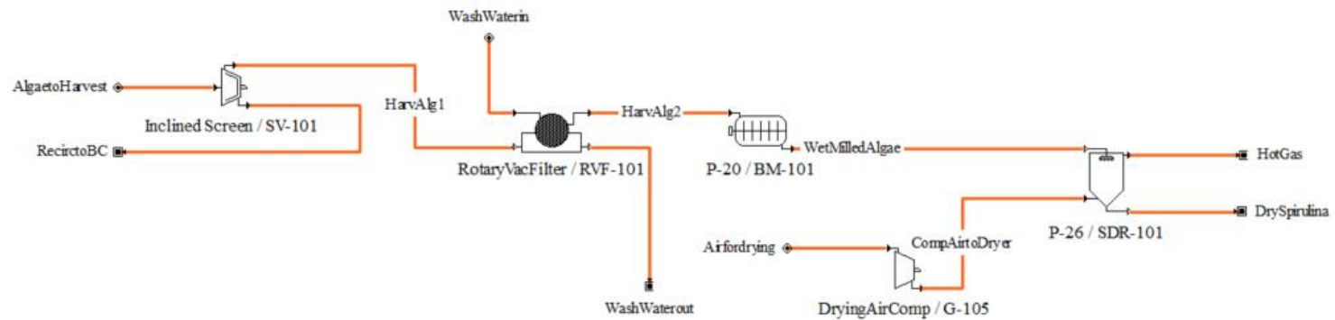
Figure 7-7 Simulated model of the microalgae harvesting and processing section towards obtaining dry Spirulina.
