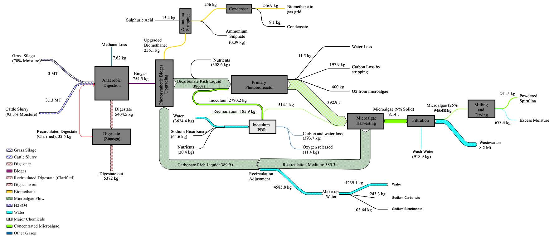
Figure 7-9 Mass flow diagram for co-generation of biomethane and Spirulina powder in a cascading polygeneration system utilising photosynthetic biogas upgrading for the base case scenario (BASE-EC)
