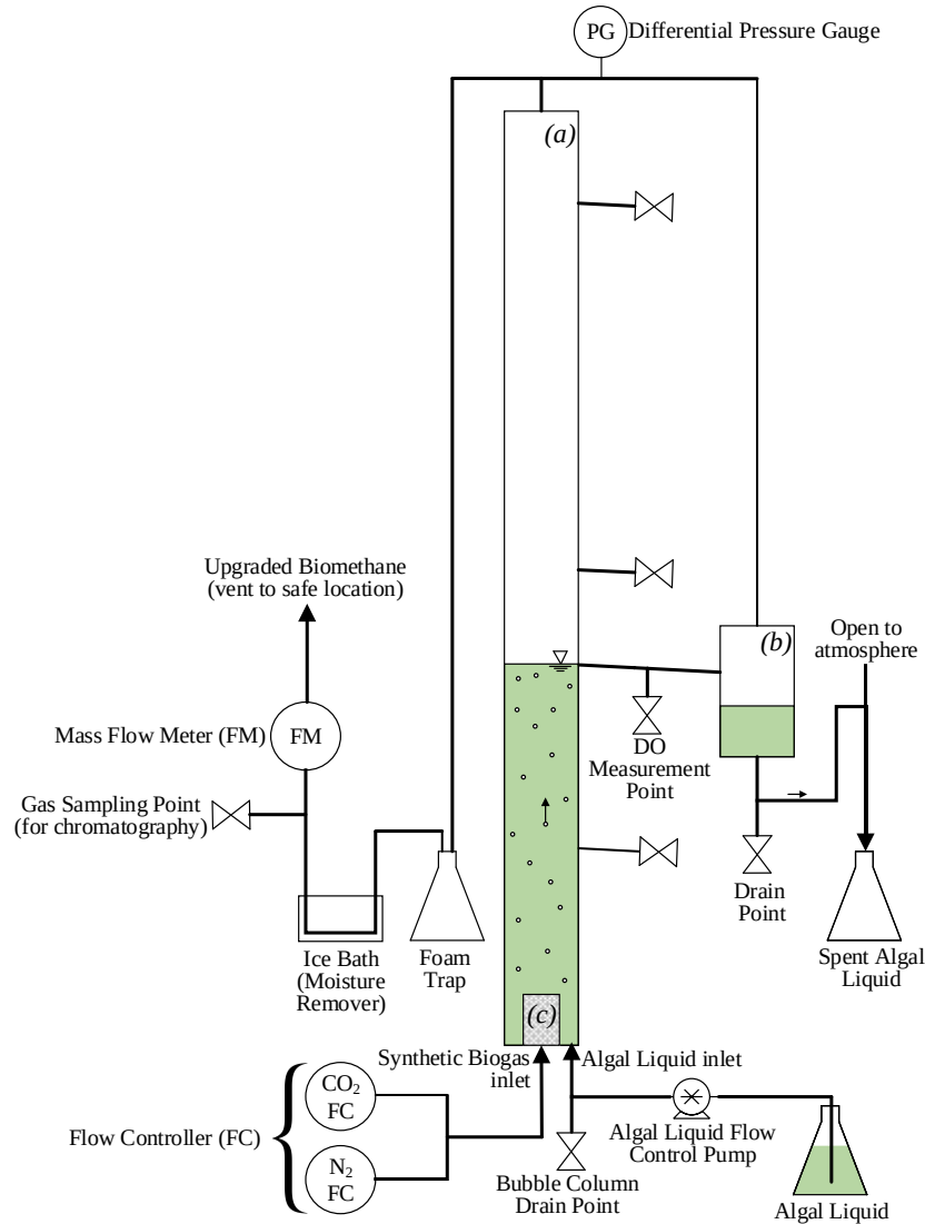
Figure 4-2 Diagrammatic representation (not to scale) of the experimental setup for the screening design of experiments where (a) is the primary bubble column, (b) is the gas-liquid separator and (c) is the gas diffuser
