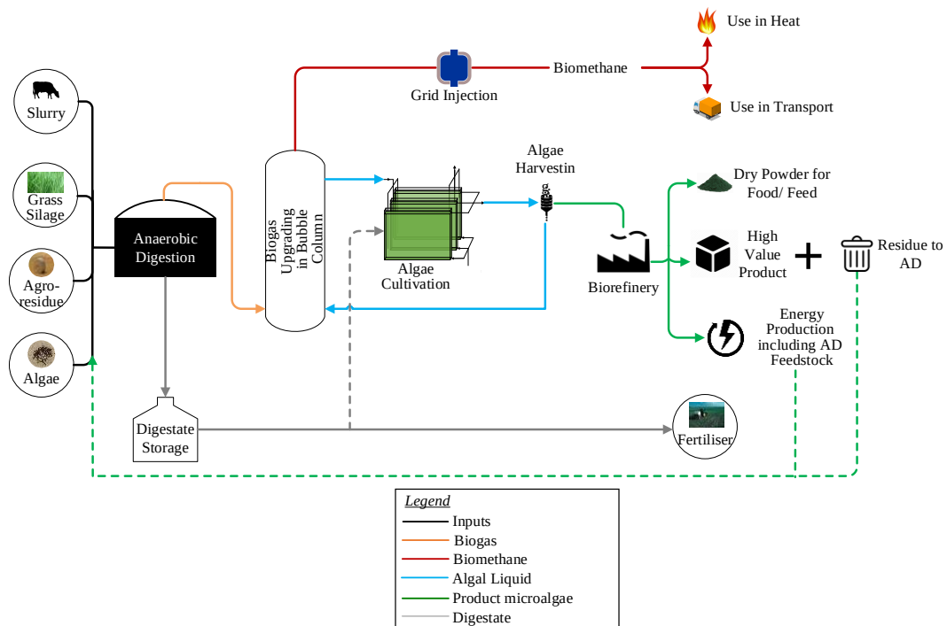
Figure 8-1 Concept layout of cascading biomethane-biorefinery with agricultural feedstock using anaerobic digestion and photosynthetic biogas upgrading.
