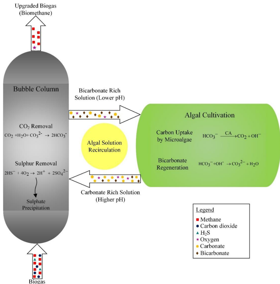
Figure 2-3 Biogas upgrading by microalgae in an alkaline (carbonate) algal solution via carbonate/bicarbonate cycle (The number of markings of each chemical species are indicative only to their relative quantity and not in absolute terms.
