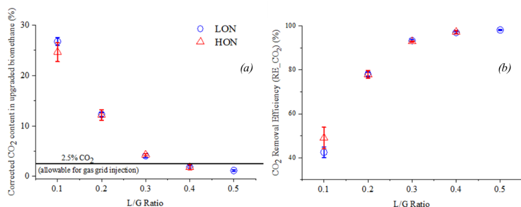
Figure 3-5 CO 2 content (a) and removal efficiency (b) of the bubble column operated under different L/G ratios at higher and lower algal concentrations; where LON: Low concentration with lights on; HON: High concentration with lights on.
