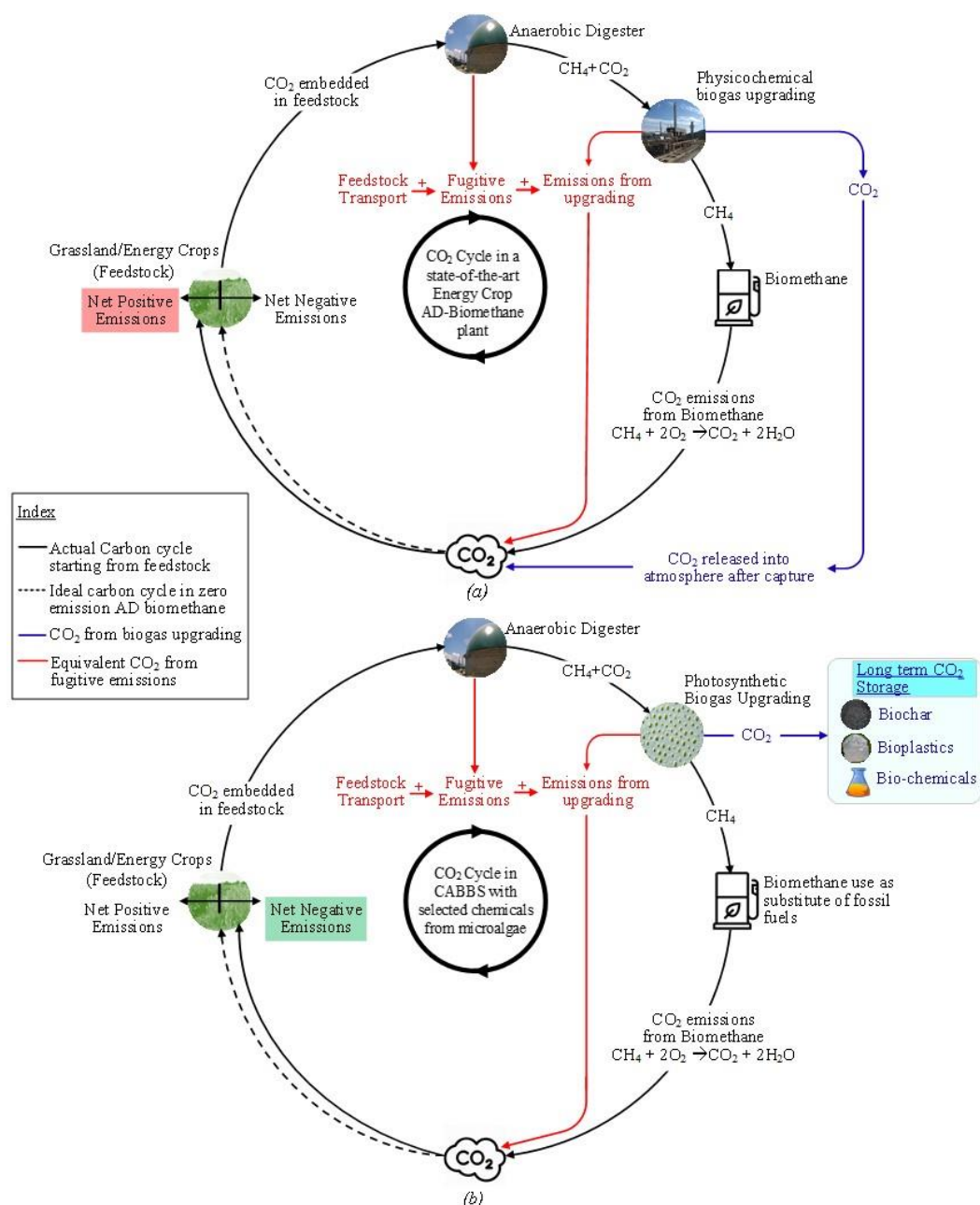
Figure 6-6 Comparison of net CO 2 flow in (a) state-of-the-art grass/energy crop based AD plant with physicochemical biogas upgrading and (b) proposed CABBS layout with the production of selected chemicals from microalgae to be regarded as a potential Bioenergy with Carbon Capture and storage (BECCS) system.
