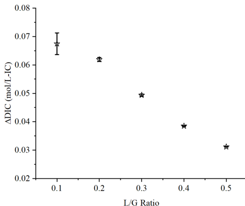
Figure 3-9 Variation in the rate of carbon addition with respect to the L/G ratio
