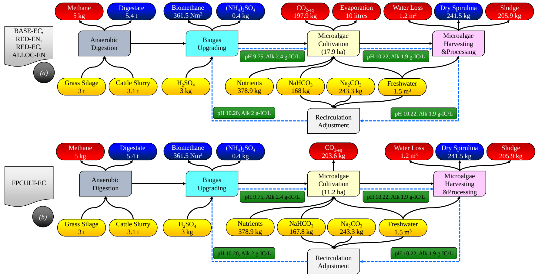
Figure 7-10 Hourly mass balance of the proposed polygeneration plant producing biomethane, Spirulina powder and digestate for (a) scenarios BASE-EC, RED-EN, RED-EC and ALLOC-EN, (b) scenario FPCULT-EC
