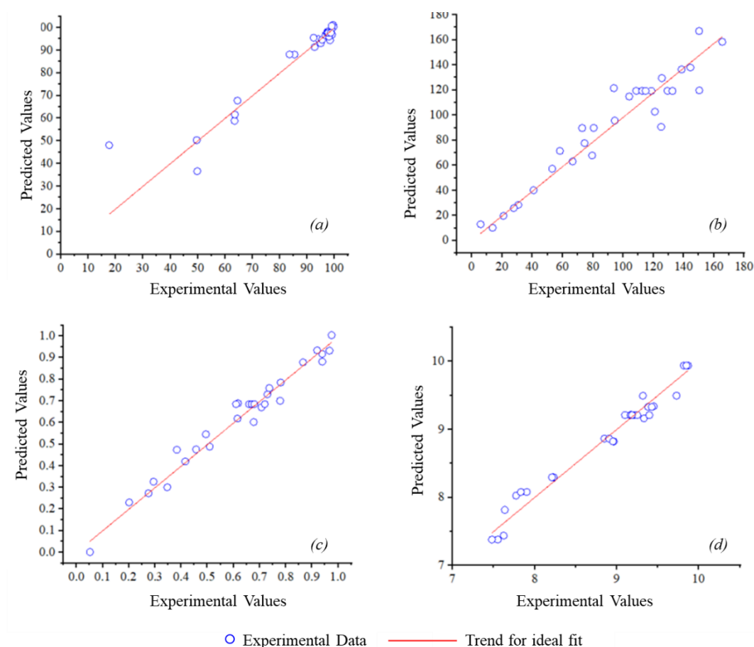
Figure 5-3 Predicted vs actual plot of the regression models for (a) \text{Eff}_{\text{RE\_CO}_2} ; (b) K_{\text{CO}_2}a ; (c) C_{\text{O}_2,\text{BM}} ; and (d) \text{pH}_{\text{out}} . The circular dots indicate the experimental data while the lines indicate the trend for ideally fit data.
