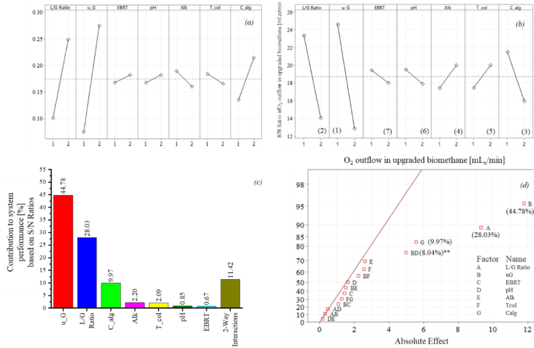
Figure 4-11 Analysis plots for the relative influence of design factors on O_2 flow rate in biomethane: (a) Main effects plot with mean; (b) Main effects plots with S/N ratio. The rank of each design factor is included in parenthesis; (c) Contribution of each design factor and interactions on the overall system outcome; and (d) Half normal probability plot with the relative contribution of major effects highlighted in brackets.
