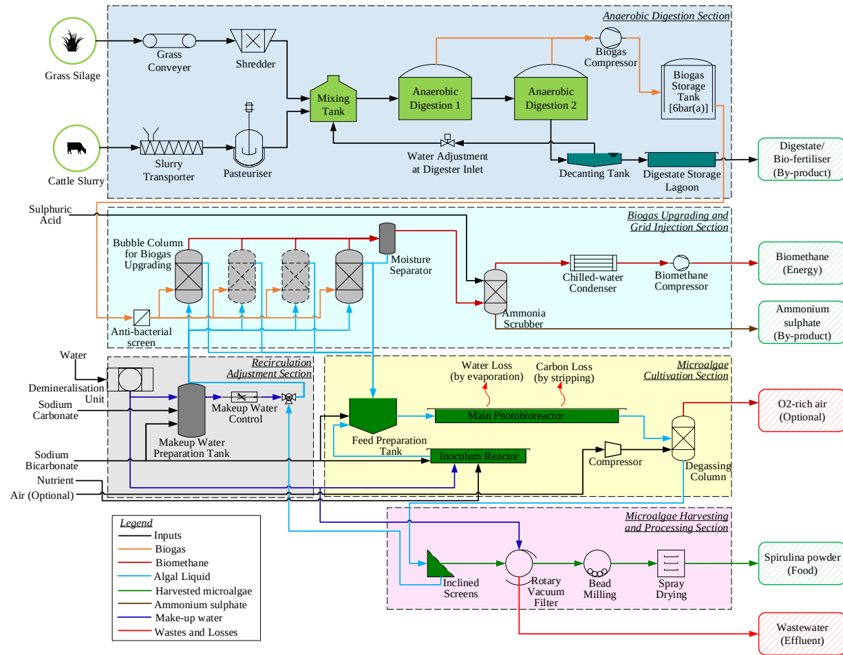
Figure 8-2 General process flow diagram of biomethane and dietary protein production as food-grade Spirulina platensis using agricultural feedstock and photosynthetic biogas upgrading
