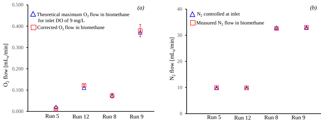
Figure 4-4 Comparison between expected and measured values of (a) \text{O}_2 and (b) \text{N}_2 to validate the bubble column operations and measurement techniques utilised.
