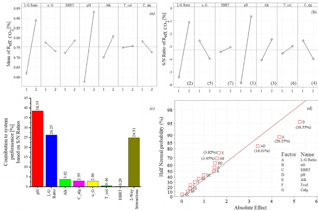
Figure 4-5 Analysis plots for the relative influence of design factors on CO 2 removal efficiency: (a) Main effects plot with mean; (b) Main effects plots with S/N ratio. The rank of each design factor is included in parenthesis; (c) Contribution of each design factor and interactions on the overall system outcome; and (d) Half normal probability plot with the relative contribution of major effects highlighted in brackets.
