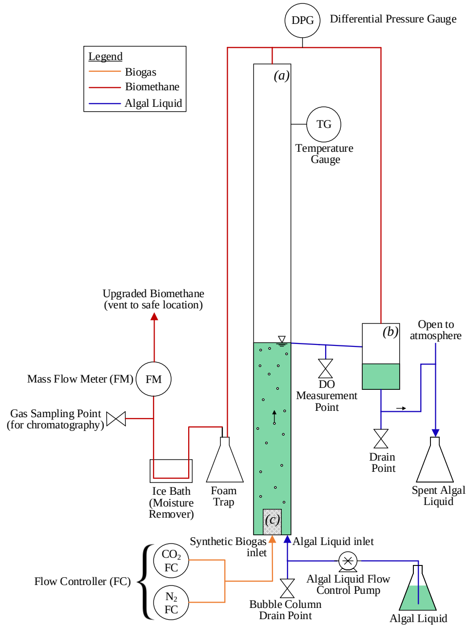
Figure 5-2 Schematic representation of the experimental setup for the optimisation of the bubble column performance (not to scale) in which (a) represents the bubble column, (b) represents the gas-liquid separator and (c) represents the gas diffuser. Adapted from Bose et al. (2021)[8]
