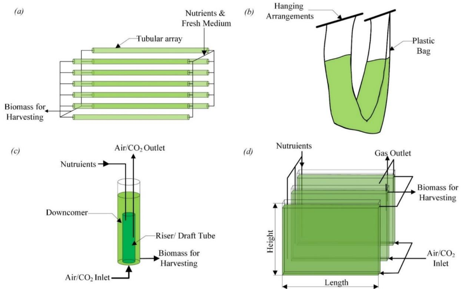
Figure 2-6 Simplistic schematic representation of closed photobioreactors, (a) Horizontal Tubular photobioreactor; (b) Plastic Bag photobioreactor; (c) Air-lift Bubble Column photobioreactor; (d) Flat Plate photobioreactor.
