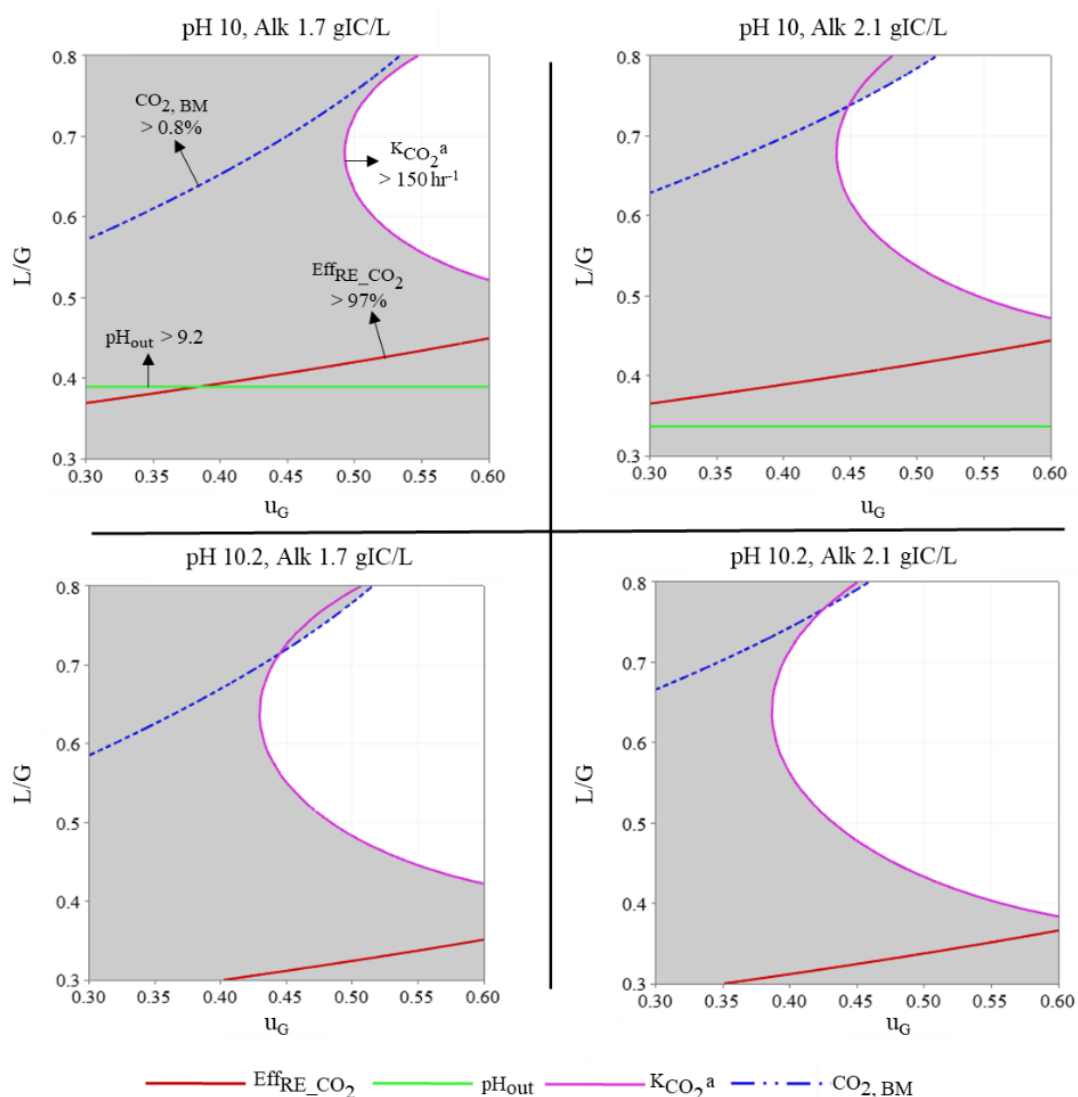
Figure 5-10 Overlaid contour plots to identify the optimal operating region of the bubble column for photosynthetic biogas upgrading for liquid inlet pH and alkalinity (Alk) ranging between 10 and 10.2 and 1.7 gIC/L and 2.1 gIC/L respectively. The un-shaded area indicates the optimal operating regions to achieve a CO_2 removal efficiency above 97% and oxygen concentration in biomethane less than 0.8%.
