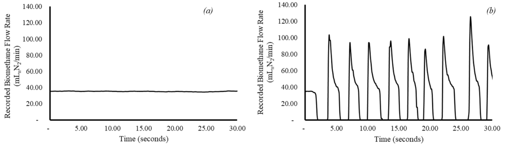
Figure 3-3 Recorded biomethane mass flow profiles at similar L/G ratio (0.3) (a) without (low algal concentrations) and (b) with foaming (high algal concentrations).
