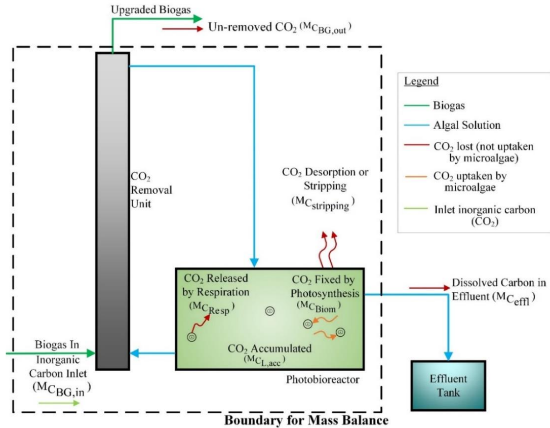
Figure 2-4 Schematic representation of overall biogas upgrading process with microalgae Indicating flow of inorganic carbon for mass balance within the system.
