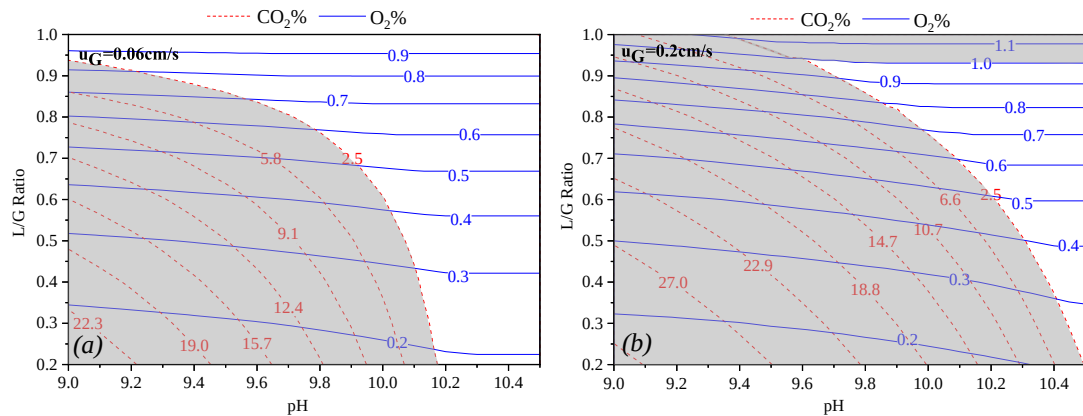
Figure 4-13 Prediction of biomethane composition at (a) u_G 0.06 cm/s (c. 0.98 L/hr) and (b) u_G 0.2 cm/s (c. 3.29 L/hr). The constant setting of other design factors are as follows: Alk 2.5gIC/L; T_{col} 20°C; C_{alg} 0.05gDW/L; and EBRT 6 mins. The acceptable region of operation is indicated in white
