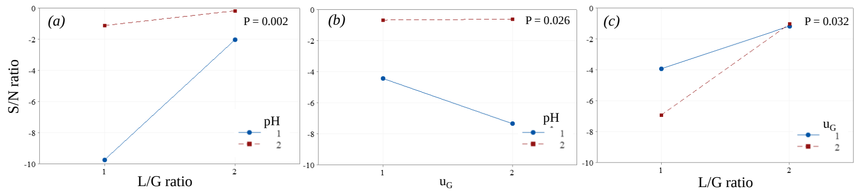
Figure 4-6 Interactive effects between (a) pH and L/G ratio; (b) superficial gas velocity ( u_G ) and pH; and (c) superficial gas velocity ( u_G ) and L/G ratio on CO_2 removal efficiency.
