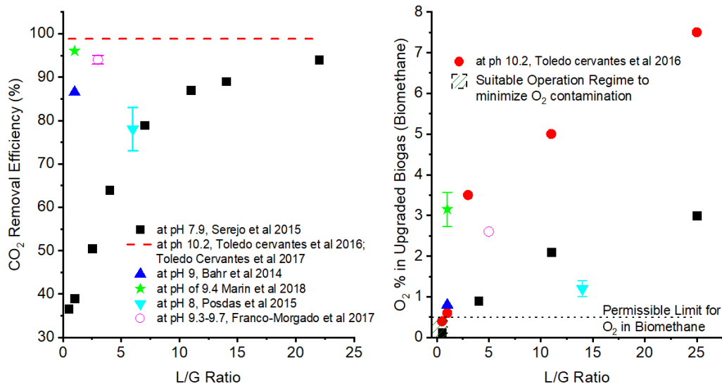
Figure 2-5 Influence of pH and L/G ratio on the mass transfer performance of the absorber column.
