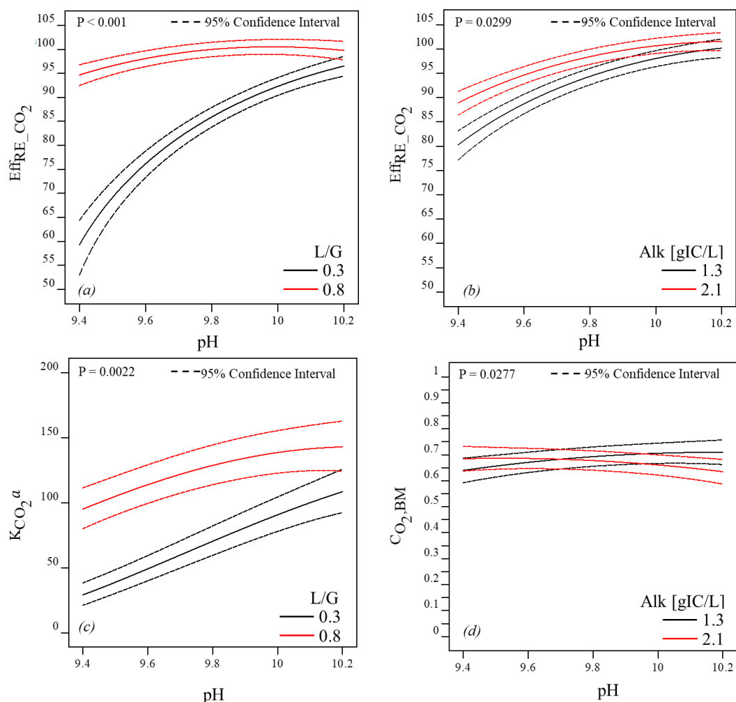
Figure 5-5 Interactive effects between (a) pH and L/G ratio on Eff_{RE\_CO_2} ; (b) pH and alkalinity on Eff_{RE\_CO_2} ; (c) pH and L/G ratio on K_{CO_2a} ; and (d) pH and alkalinity on CO_{2,BM} . Except for the factors that are being varied, all the other factors are placed at their centre points, namely, pH at 9.8; u_G at 0.45 cm/s, L/G at 0.55 and Alk at 1.7 gIC/L
