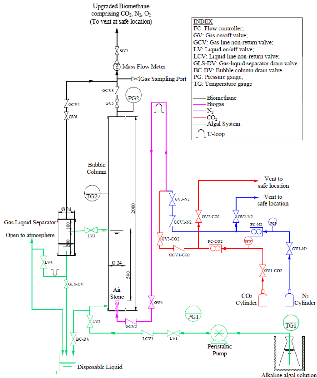
Figure 3-1 Process flow diagram and design details of the lab-scale bubble column for photosynthetic biogas upgrading (Not to scale)
