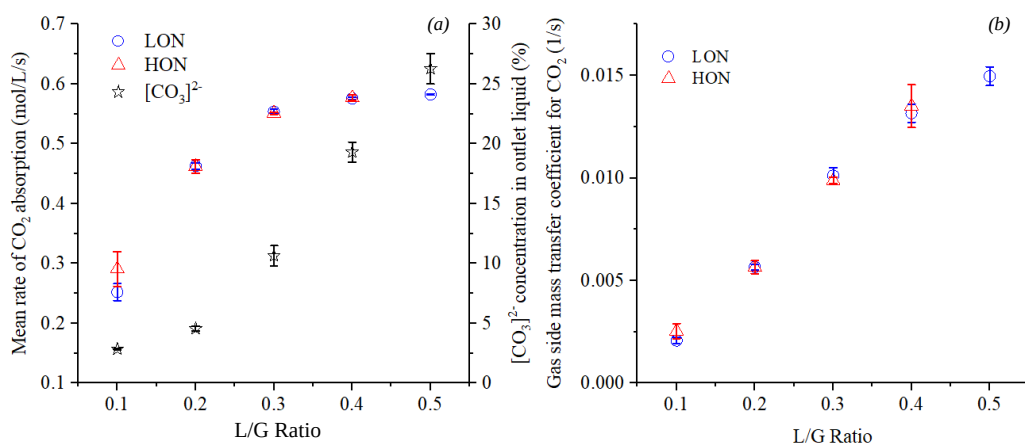
Figure 3-6 Effect of L/G ratio and algal concentration on the (a) absorption rate of CO 2 alongside mean carbonate concentration in solution and (b) overall mass transfer coefficient ( k_{G_{CO_2}}a ).
