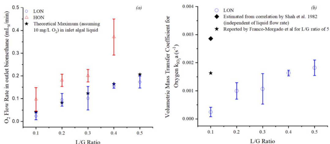
Figure 3-7 Effect of the L/G ratio and the algal concentration on (a) the theoretical and measured oxygen outflow rates [mL n /min] and (b) the overall mass transfer coefficient for oxygen ( k_{lO_2}a ) [s -1 ].
