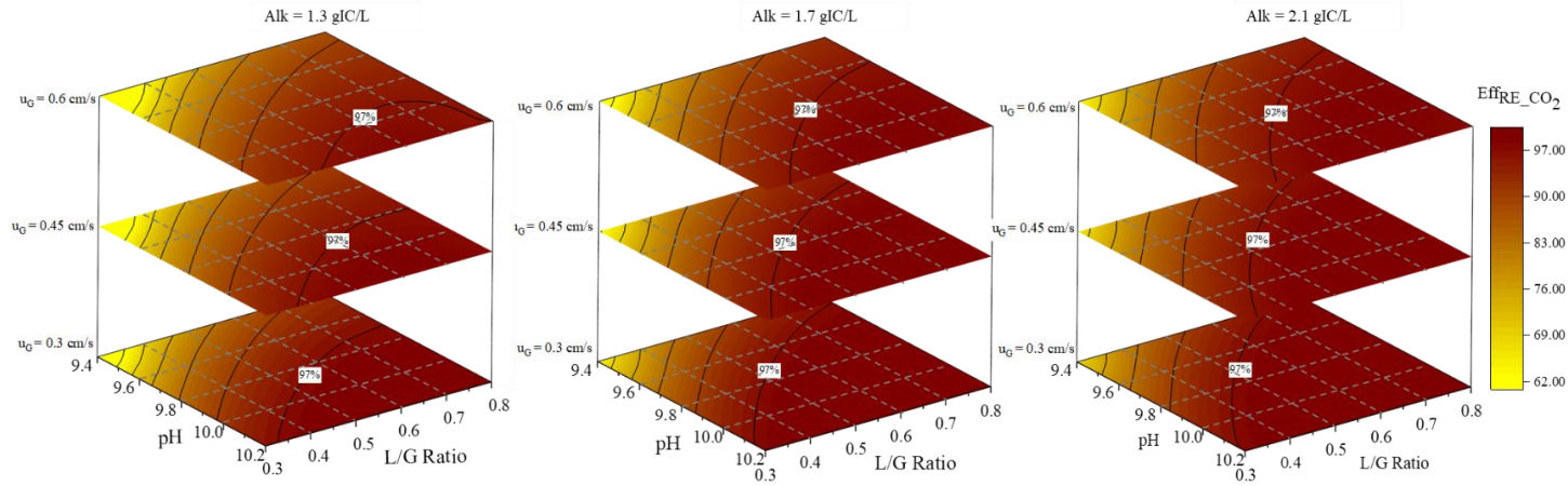
Figure 5-6 Two dimensional contour plots of CO 2 removal efficiency ( Eff_{RE\_CO_2} ) versus pH and L/G ratio at different superficial gas velocities and alkalinity. The contour lines correspond to the values indicated in the legend.
