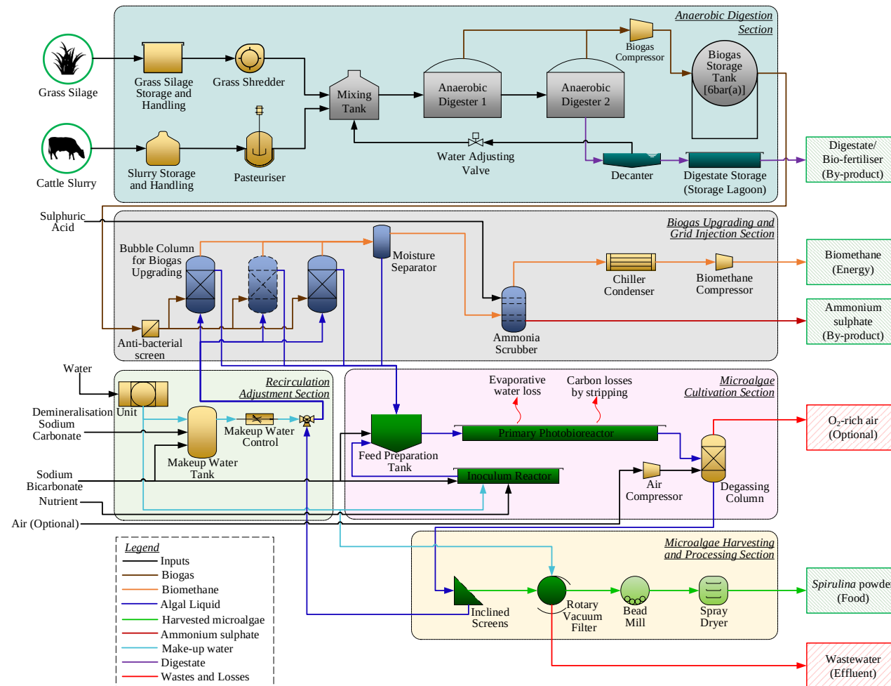
Figure 7-2 General process flow diagram of biomethane and dietary protein production as food-grade Spirulina platensis alongside biofertiliser as digestate using agricultural feedstock and photosynthetic biogas upgrading
