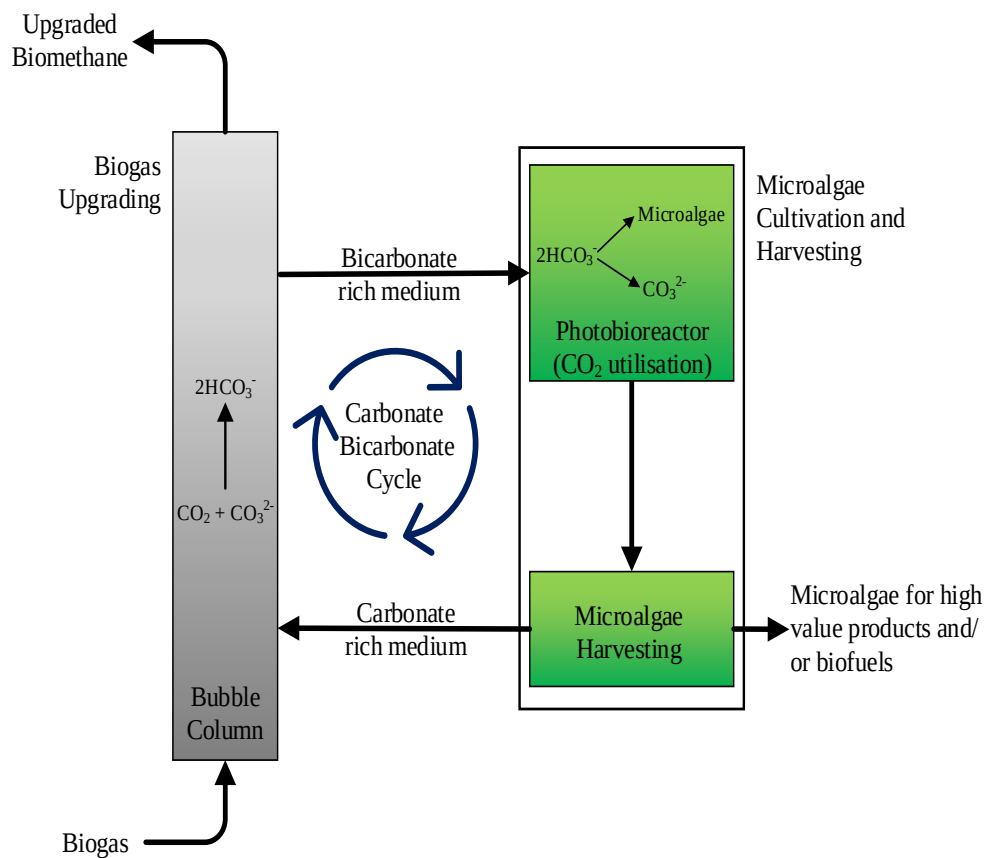
Figure 4-1 Diagrammatic representation of the two-step bubble column-photobioreactor photosynthetic biogas upgrading system using the carbonate bicarbonate cycle for the production of biomethane and microalgae for high-value products and/or biofuels.
