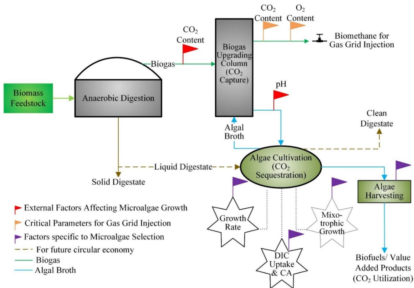
Figure 2-1 Process flow diagram and system configuration for biogas upgrading with microalgae where DIC: dissolved inorganic content; CA: Carbonic anhydrase
