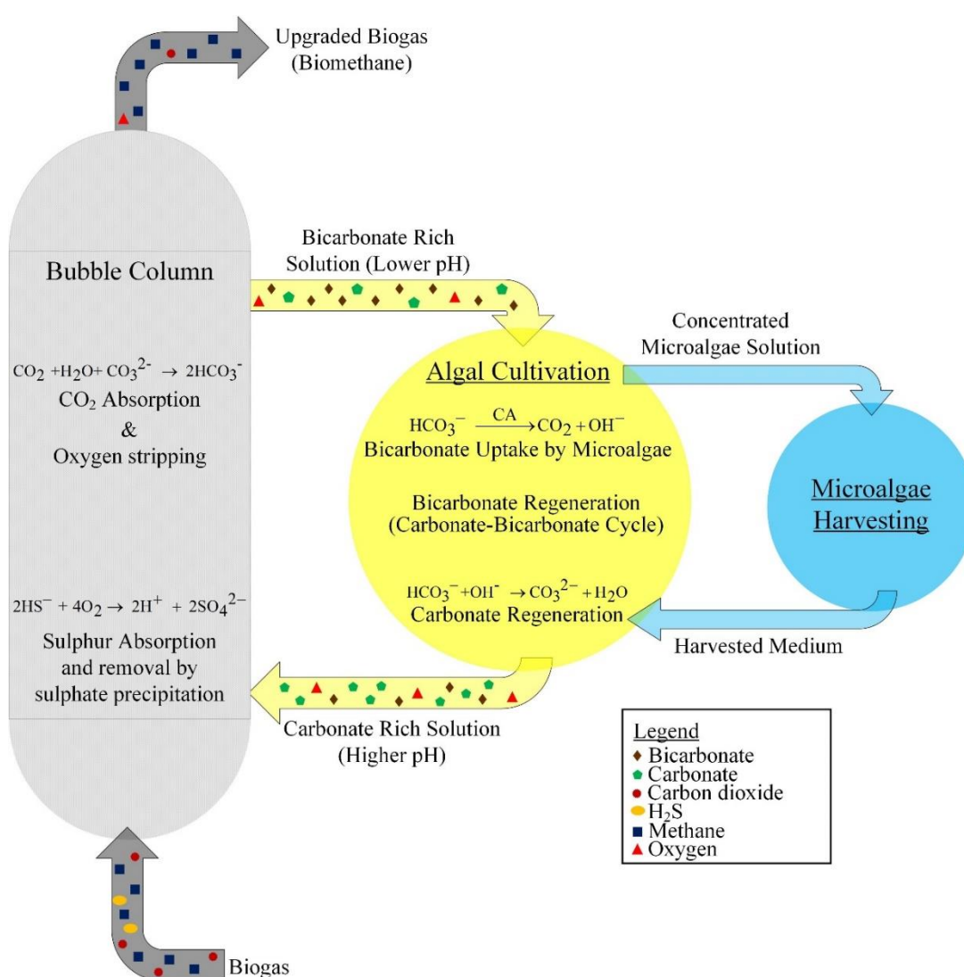
Figure 6-2 Schematic of photosynthetic biogas upgrading in an alkaline (carbonate) algal solution via carbonate/bicarbonate cycle followed by microalgae harvesting (The number of markings of each chemical species are indicative only to their relative quantity and not in absolute terms) [8]
