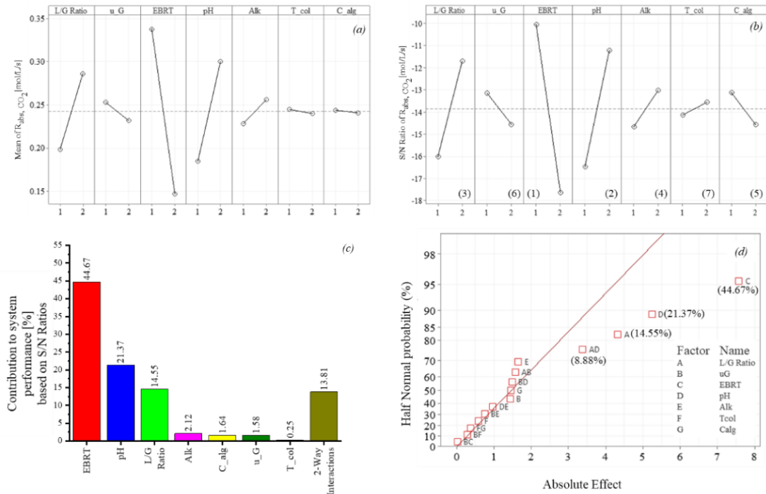
Figure 4-7 Analysis plots for the relative influence of design factors on mean steady state rate of CO 2 absorption: (a) Main effects plot with means; (b) Main effects plots with S/N ratio. The rank of each design factor is included in parenthesis; (c) Contribution of each design factor and interactions on the overall system outcome; and (d) Half normal probability plot with the relative contribution of major effects highlighted in brackets.
