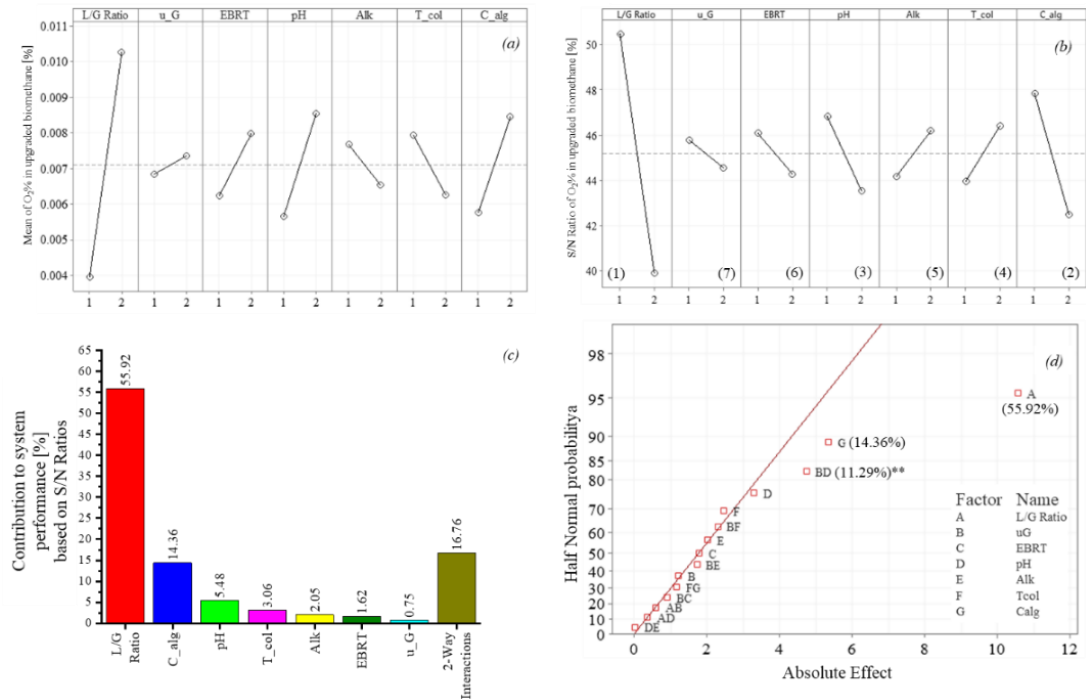
Figure 4-9 Analysis plots for relative influence of design factors on O_2 concentration in biomethane: (a) Main effects plot with mean; (b) Main effects plots with S/N ratio. The rank of each design factor is included in parenthesis; (c) Contribution of each design factor and interactions on the overall system outcome; and (d) Half normal probability plot with the relative contribution of major effects highlighted in brackets.
