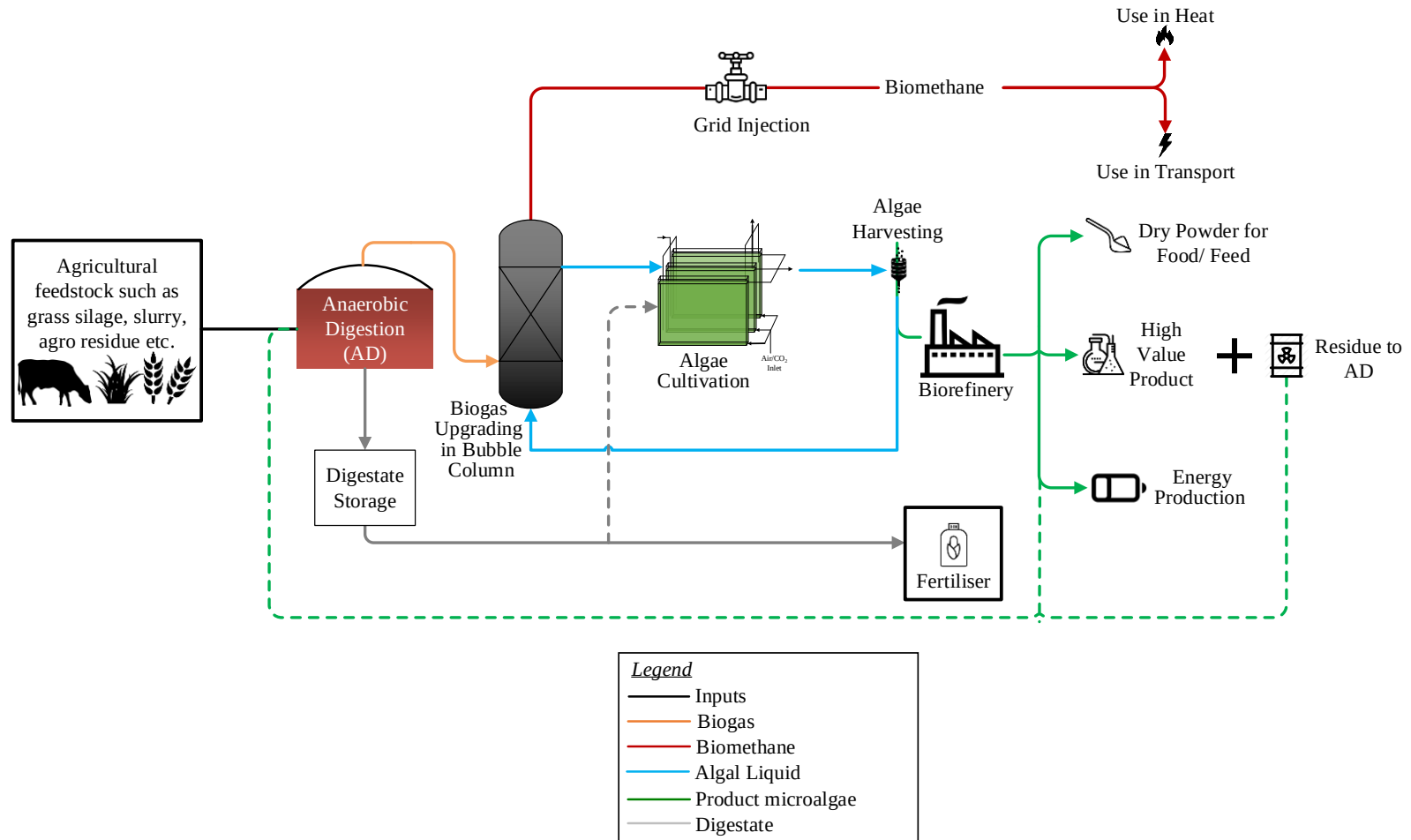
Figure 7-1 Concept layout of cascading algal biomethane-biorefinery systems (CABBS) with agricultural wastes using anaerobic digestion and photosynthetic biogas upgrading
