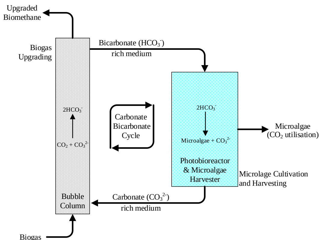
Figure 5-1 Concept diagram of the two-step bubble column-photobioreactor photosynthetic biogas upgrading system using the carbonate bicarbonate cycle for the production of biomethane and microalgae.
