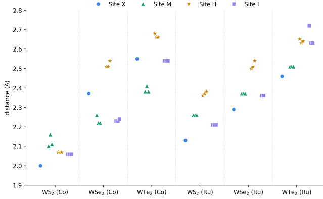
Figure 4: Adatom-chalcogen distances for single atom adsorption.
