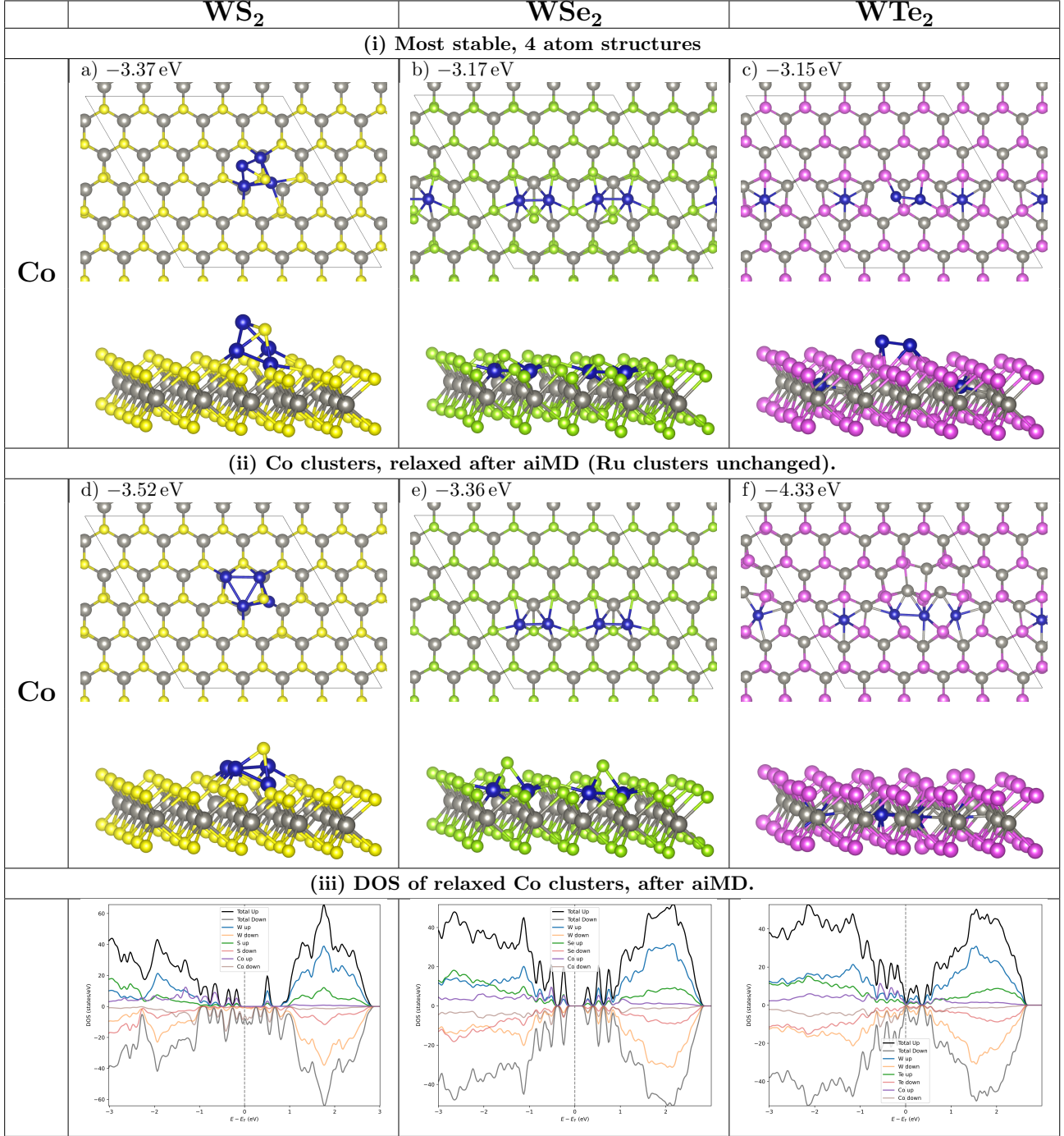
Figure 7: Four-atom adsorption. (i) Most stable Co 0 K structures on (a) WS 2 , (b) WSe 2 , and (c) WTe 2 . (ii) Co structures after 500 K aiMD on (d) WS 2 , (e) WSe 2 , and (f) WTe 2 . The tetrahedron transitions to 2D (WS 2 ), Se vacancies form (WSe 2 ), and WTe 2 distorts to a local orthorhombic phase. Ru clusters do not alter the monolayer or transition to alternative structure during aiMD, see figure 8. (iii) Total DOS of relaxed structures, after aiMD. E_{bind}/atom in eV. Colours as in Fig. 2.
