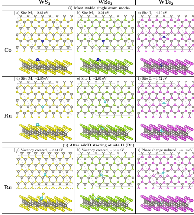
Figure 2: Single-atom adsorption on WX 2 . (i) Most stable single atom sites for Co on (a) WS 2 , (b) WSe 2 , (c) WTe 2 , and Ru on (d) WS 2 , (e) WSe 2 , (f) WTe 2 . (ii) Ru structures after relaxing final frame of aiMD, where the monolayer is altered by chalcogen migration ((g) WS 2 , (h) WSe 2 ) or a local phase change ((i) WTe 2 ). Co atoms do not alter the monolayer during the course of relaxation. Only one migration is seen for Co and its path is shown in figure 5. E_{bind/atom} in eV. Colours: blue = Co; cyan = Ru; grey = W; yellow = S; green = Se; purple = Te.
