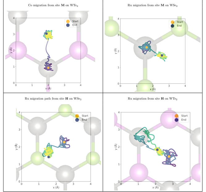
Figure 5: Plot of the migration path for single Co and Ru adatoms in the aiMD simulations. Specifically Co at site M on \text{WTe}_2 (top left), Ru at site M on \text{WSe}_2 (top right), Ru at site H on \text{WSe}_2 (bottom left), and Ru at site H on \text{WTe}_2 (bottom right).
