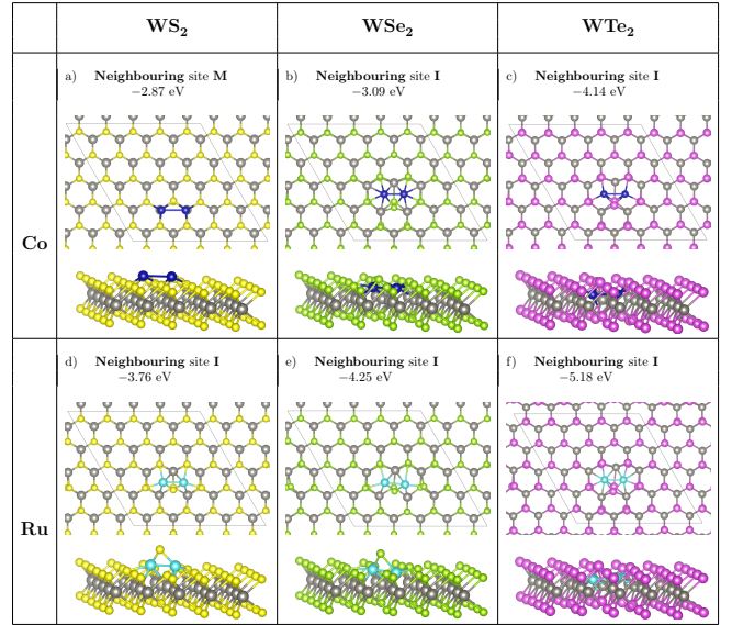
Figure 6: Most stable 2 atom adsorption modes: Co on (a) WS 2 , (b) WSe 2 , (c) WTe 2 , and Ru on (d) WS 2 , (e) WSe 2 , (f) WTe 2 . Ru shows a preference for adsorption at site I , making chalcogen atoms migrate from their original site on WS 2 and WSe 2 . E_{bind}/atom shown in eV in this figure. Atomic colours are as follows: blue = Co; cyan = Ru; grey = W; yellow = S; green = Se; purple = Te.
