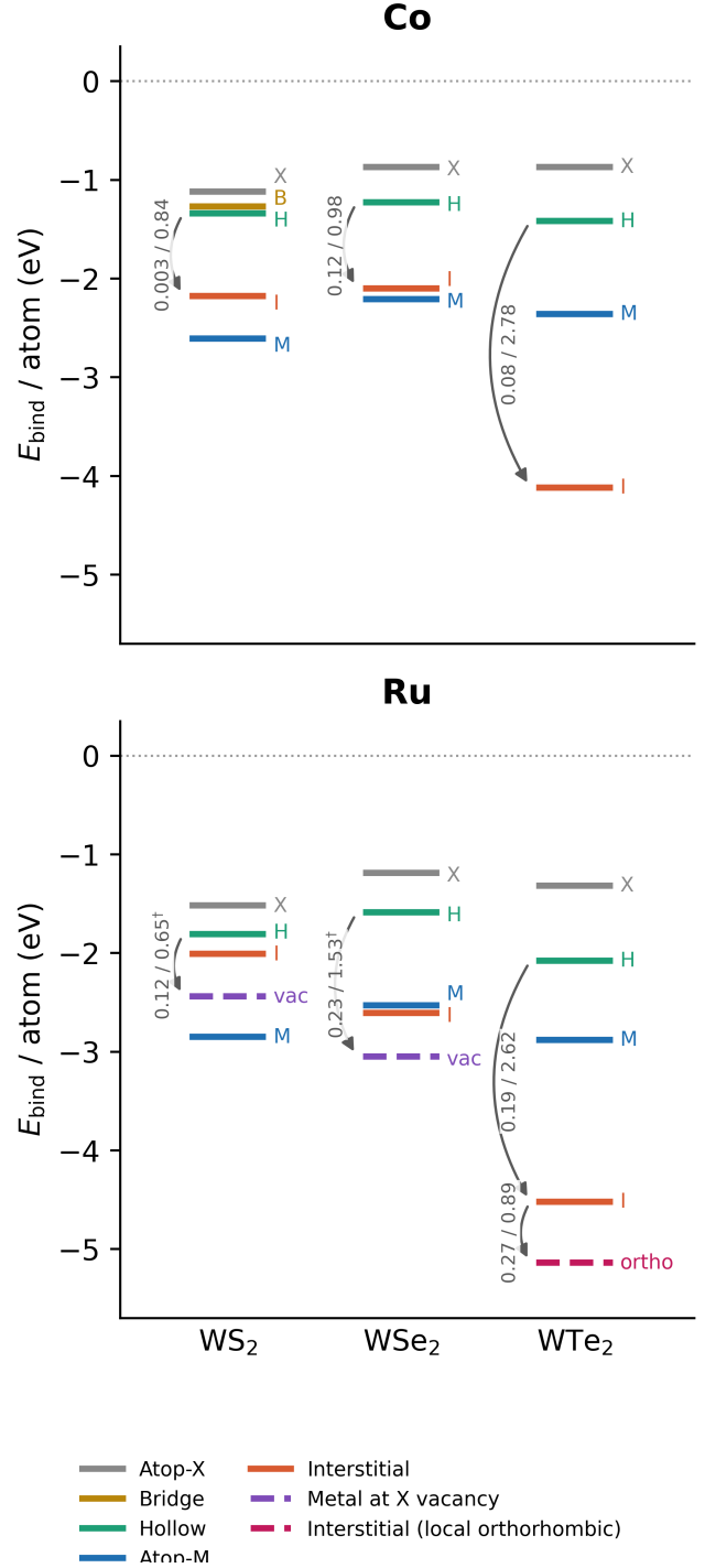
Figure 3: Schematic showing relative energies of sites, and activation barriers between sites for single atom Co (top) and Ru (bottom) structures. Arrows display the forward and reverse NEB barriers, with largest barrier shown for two step processes (denoted by †). “vac” denotes the metal occupying a chalcogen-vacancy site and “ortho” the interstitial site in the locally orthorhombic structure.
