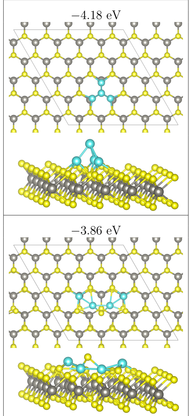
Figure 8: Examples of Ru adsorption structures containing 4 atoms. Tetrahedron adsorption structure at site M , the most stable Ru 4 atom structure on each monolayer (top). Ru structure forming a sulphur vacancy (bottom).
