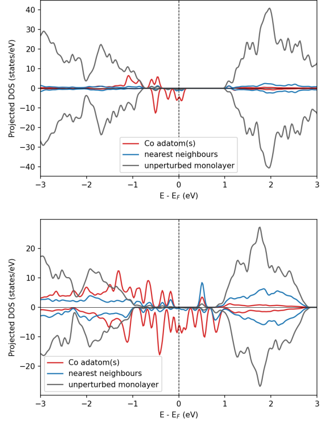
Figure 10: Total (summed over all orbitals) projected density of states of Co adatoms, nearest neighbours, and atoms far from the adsorbed Co atoms. Although Co atoms induce states crossing the Fermi level, this is only a local perturbation. DOS corresponds to Co-S-M (top, figure 2 (a)) and Co-S-Htet-vac (bottom, figure 7 (a)).
