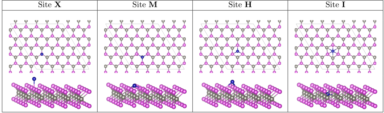
Figure 1: Adsorption structures of a single Co atom on WX_2 to illustrate the four main adsorption sites. The example used is a single cobalt atom on WTe_2 . Site B can be seen in Figure S2 of the Supporting Information. Atomic colours are as follows: grey = W; purple = Te; blue = Co.
