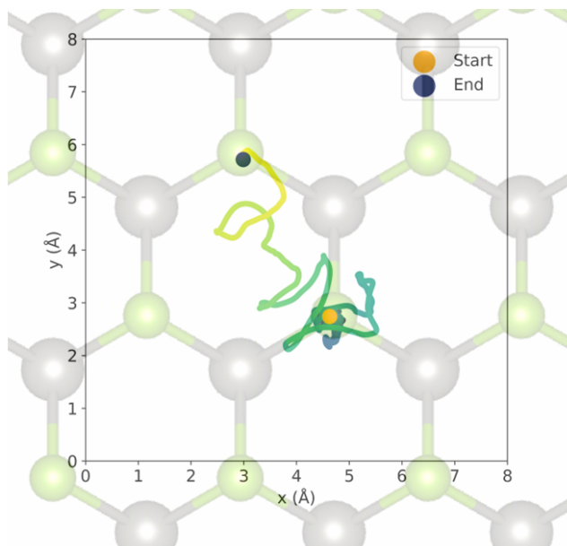
Figure 9: Migration path of the centre of mass of Ru tetrahedron from 15 ps aiMD simulation on WSe 2 .
