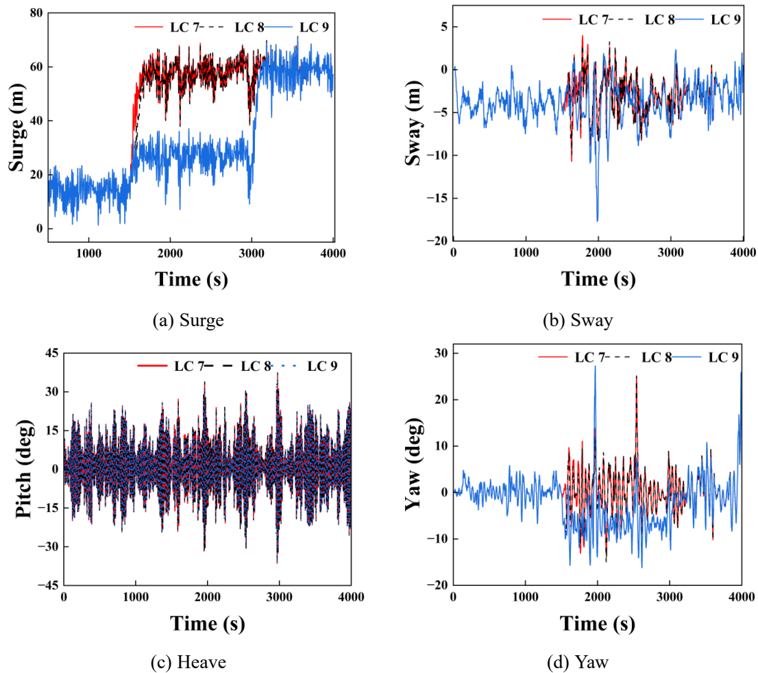
Fig. 14 Dynamic response of the platform after the failure of mooring #4 and #5 in extreme sea conditions
