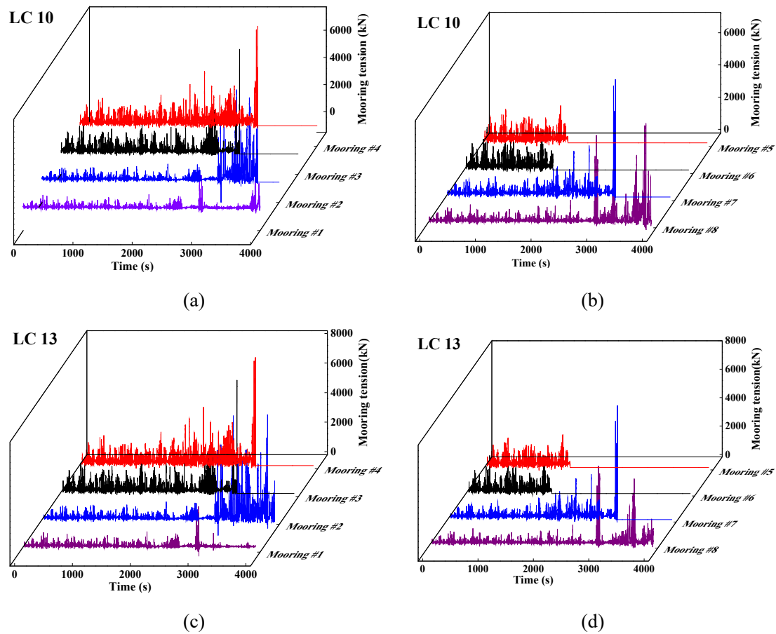
Fig. 19 Comparison of the mooring tensions
