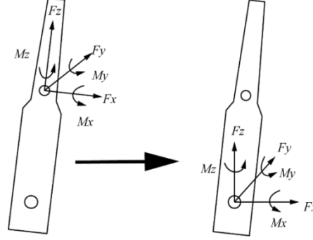
Fig. 5 Coordinate transformation
