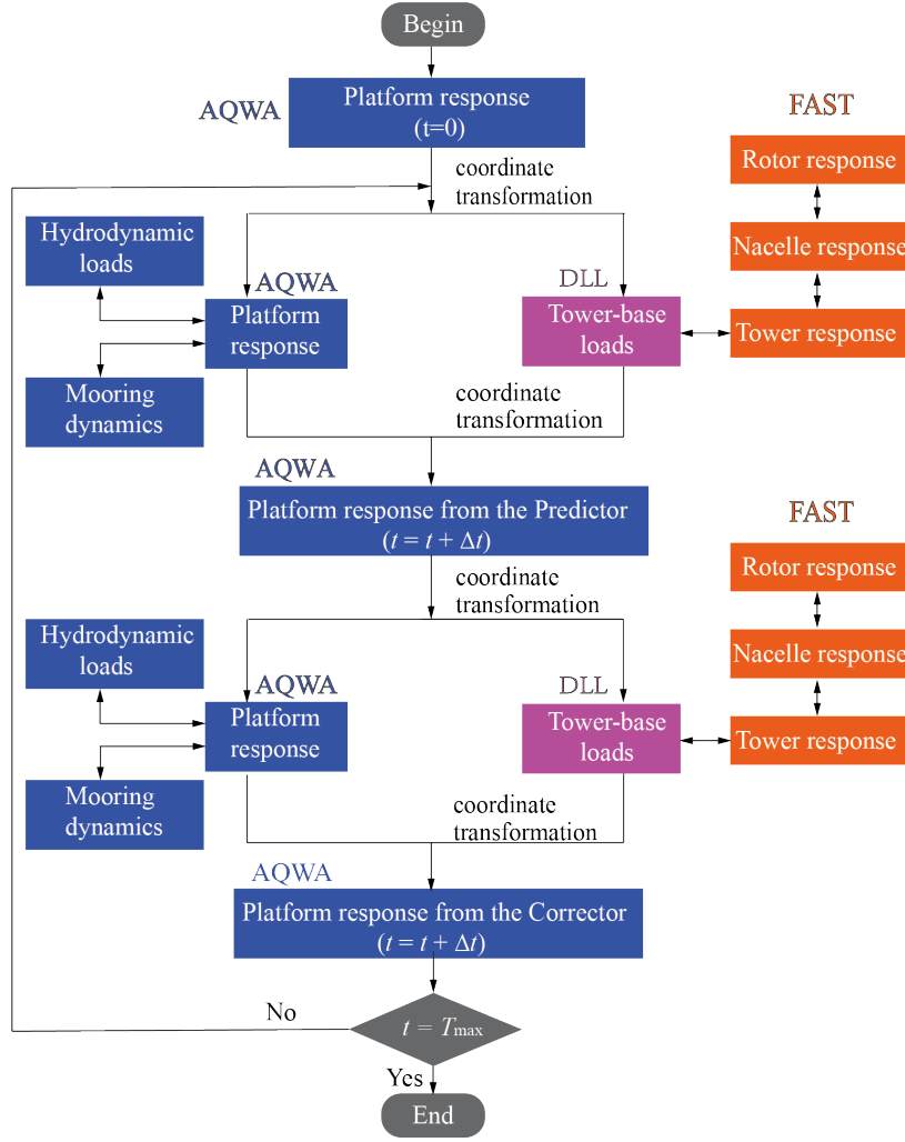
Fig.4 Calculation flowchart of the numerical simulation.
