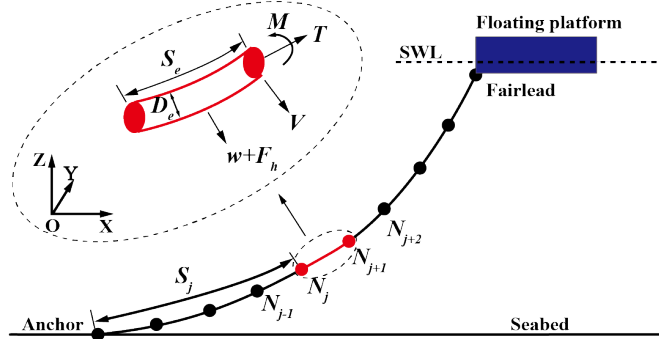
Fig. 3 Schematic diagram of the dynamic model of a mooring line
