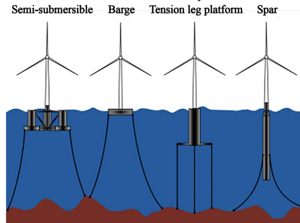
Fig.1 Comparative overview of the four principal FOWT configurations: (L-R) Semi-submersible, Barge, Tension leg platform and Spar
