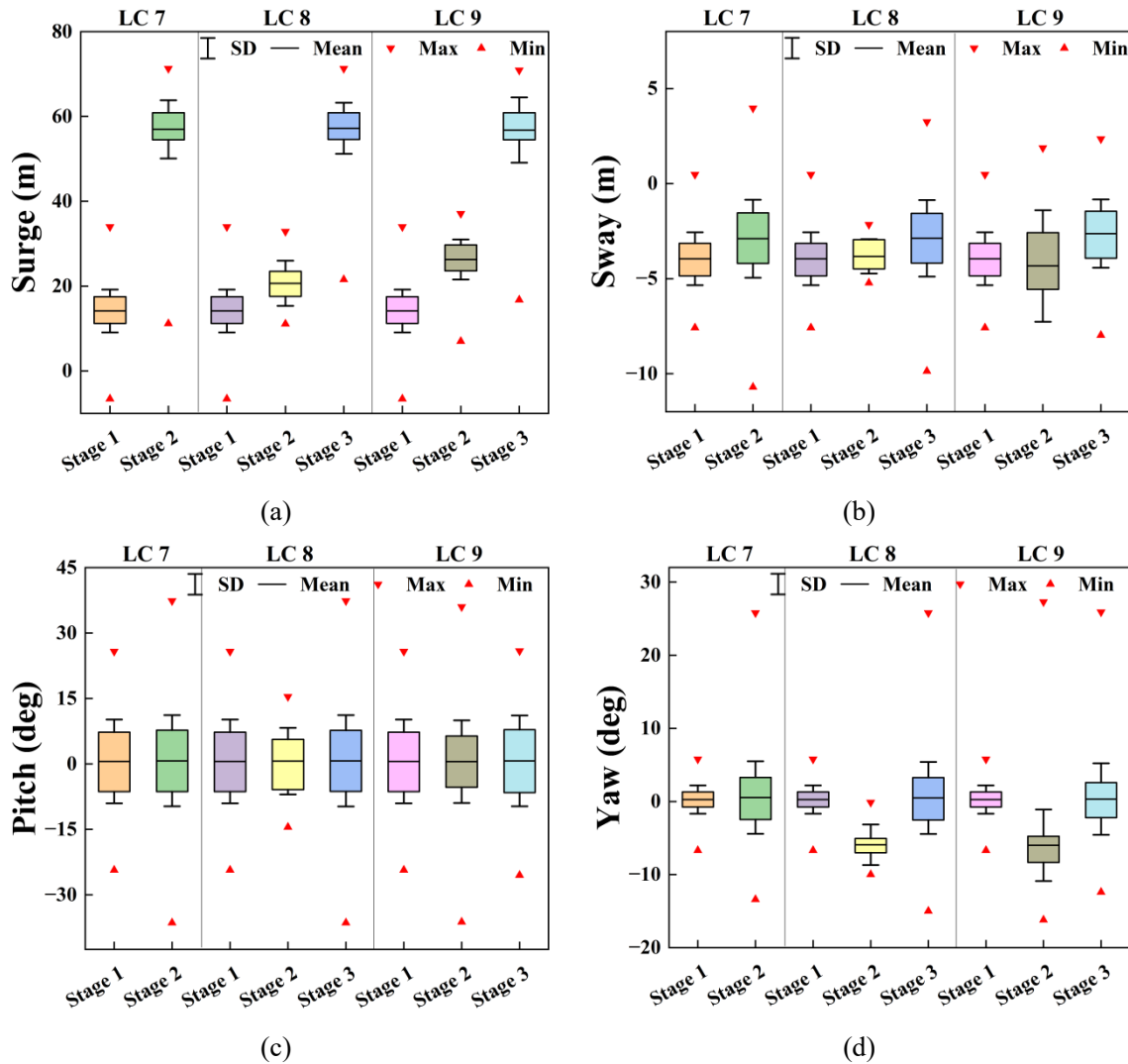
Fig. 15 Statistics for motion responses of the platform after the failure of mooring # 4 and # 5 in extreme sea conditions
