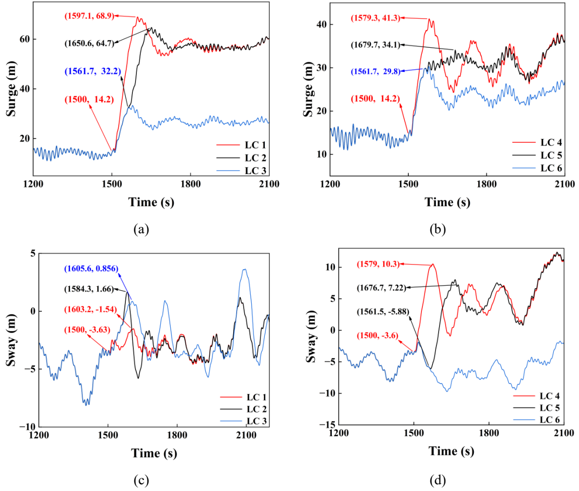
Fig. 9 Local time-domain response in rated sea conditions
