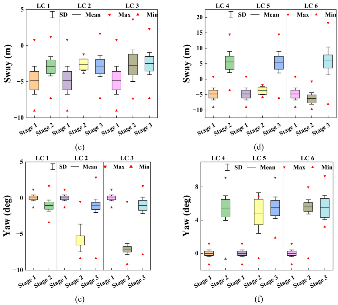
Fig. 10 Statistics for motion responses in rated sea conditions
