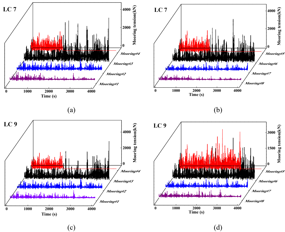
Fig. 16 Comparison of mooring tension in extreme sea conditions of LC 7 and LC 9
