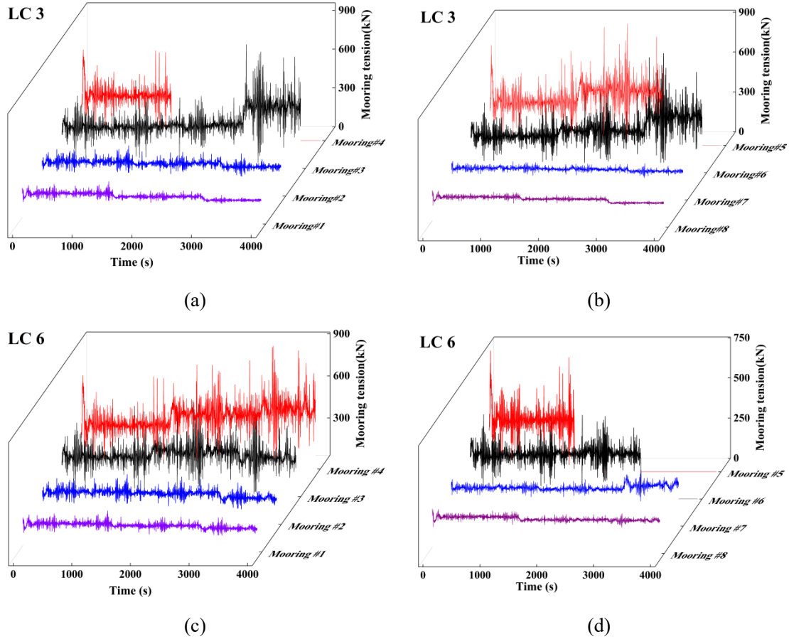
Fig. 12 Comparison of mooring tension between LC3 and LC 6 in rated sea conditions
