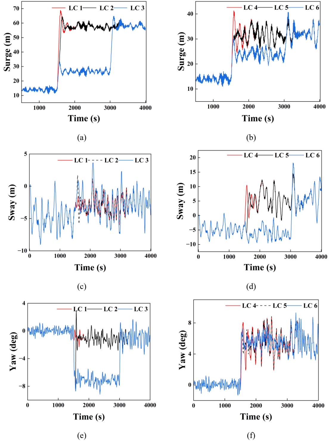
Fig. 8 Platform motions in rated sea conditions
