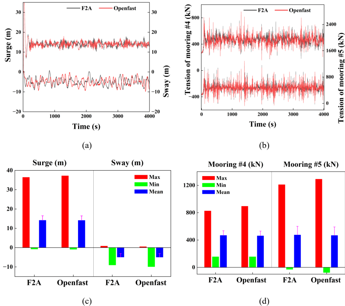
Fig. 7 Comparison between coupled responses of F2A and OpenFAST.
