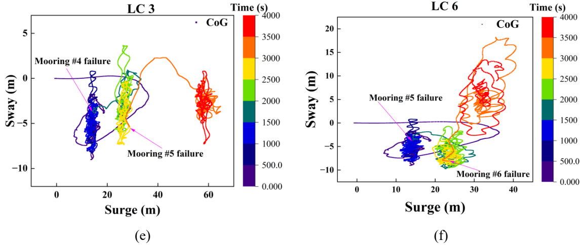
Fig. 11 Platform motion trajectory of CoG in rated sea conditions
