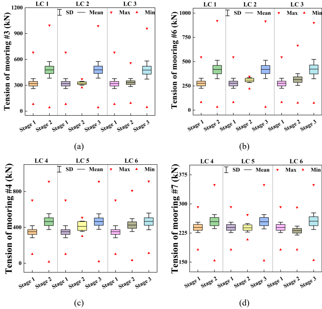
Fig. 13 Statistics for mooring tension in rated sea conditions
