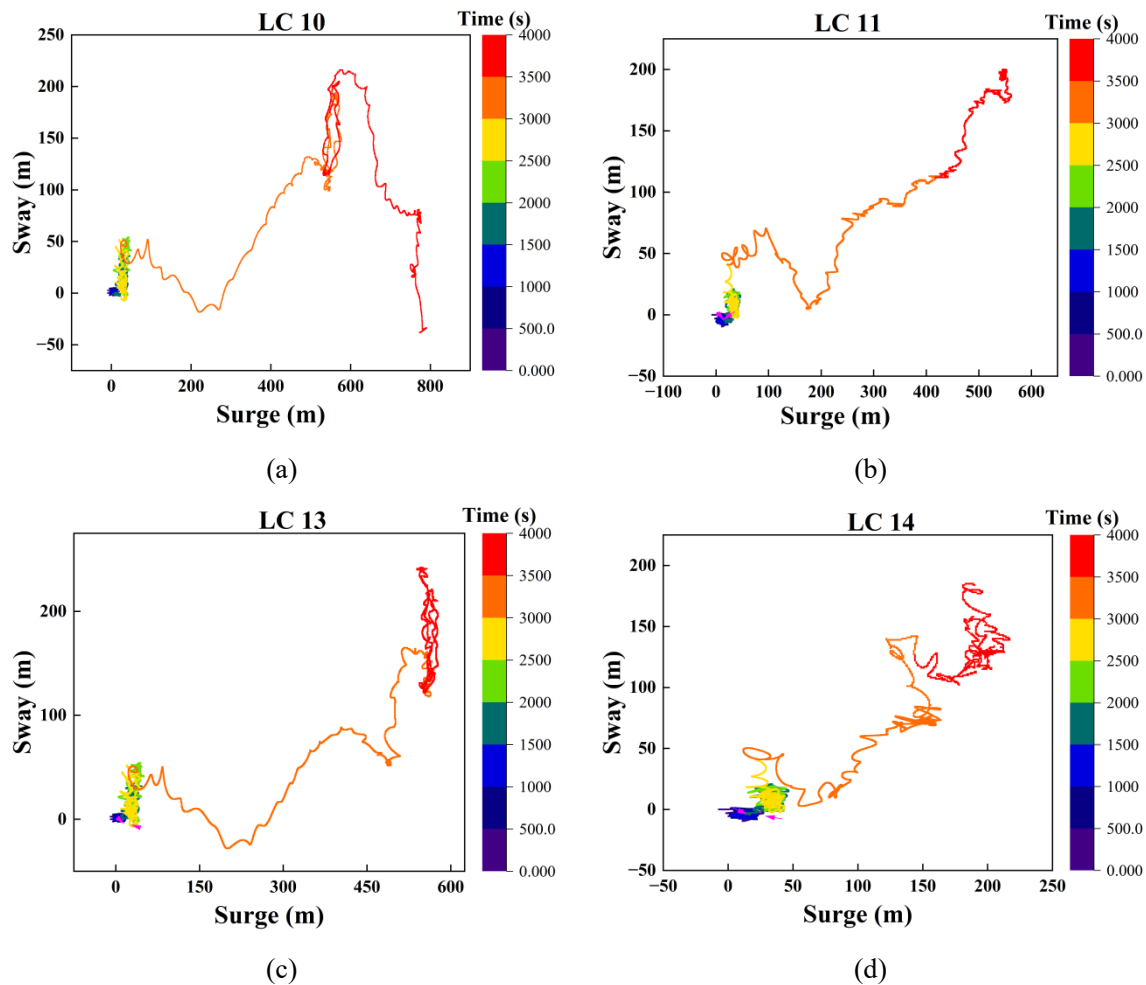
Fig. 18 Platform motions trajectory after the failure of mooring # 5 and # 6 in extreme sea conditions
