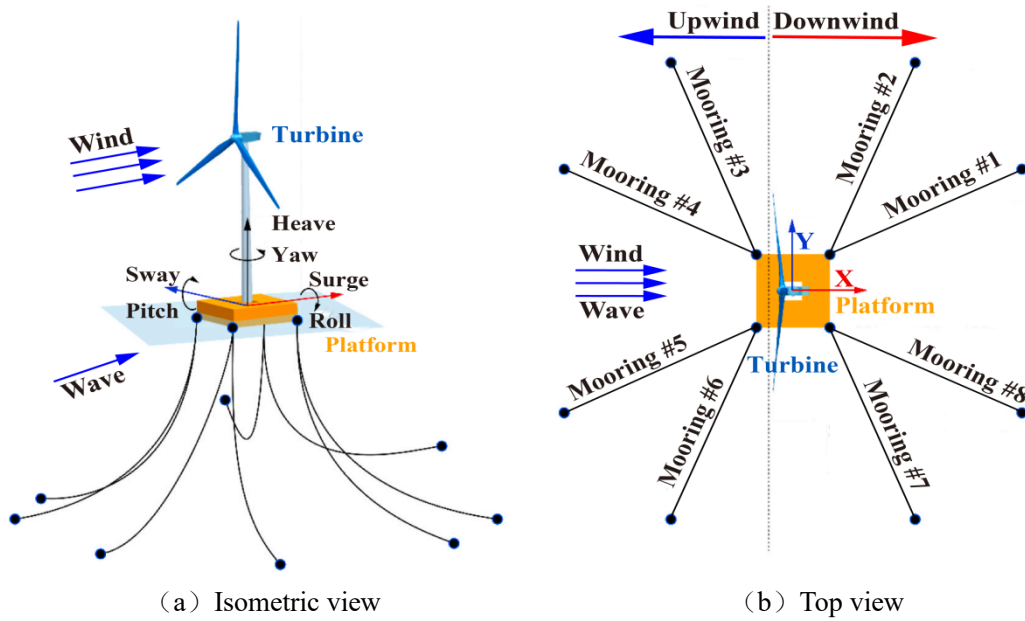
Fig. 2 The NREL 5 MW wind turbine supported by the barge platform
