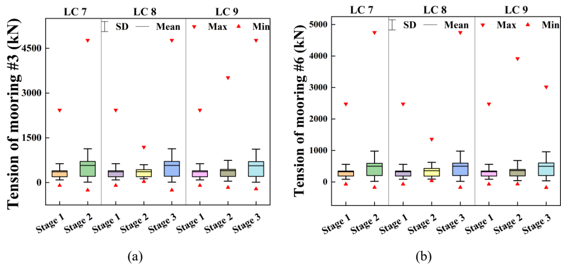
Fig. 17 Statistics for mooring tension in extreme sea conditions
