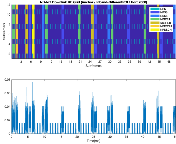
Fig. 4: NB-IoT waveform generated by the Matlab simulation environment. The upper representation displays the channels and signal assign to each subframe. The lower figure display the allocation of the same signals and channels in a time-frequency domain.
