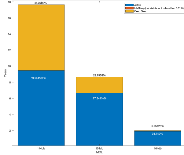
Fig. 5: Achievable battery lifetime of an NB-IoT node in our baseline scenario using communication parameter settings of t = 2h , b_{up} = 200byte and b_{up} = 60byte under different MCL scenarios. No jamming attack is present (Baseline Scenario).
