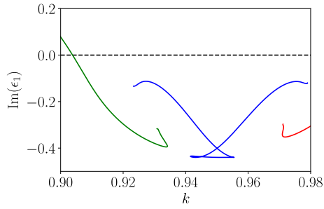
(c) \Lambda_2, k plane with \Lambda_1 = 1.22 .
