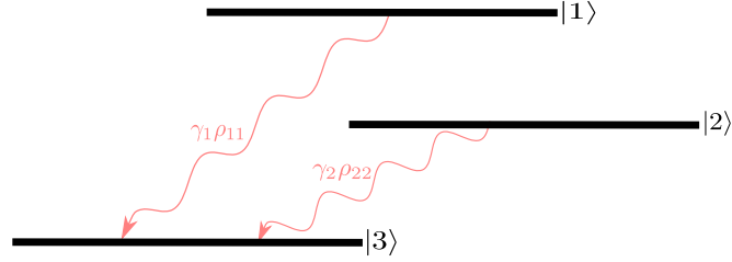
Figure 2.2: Two-level atom with the excited state |1\rangle and lower state |2\rangle . Both decay to a level |3\rangle at decay rates \gamma_1 and \gamma_2 from levels |1\rangle and |2\rangle respectively.
