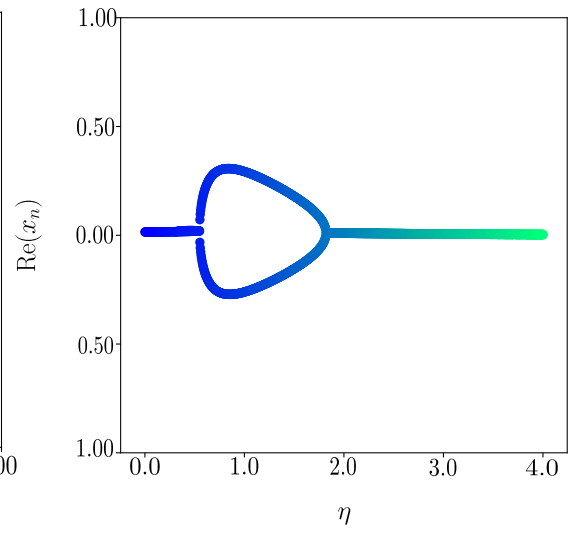
(b) Real part of x_n(\omega) with varying \eta .
