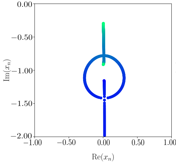
(a) Real and imaginary parts of x_n(\omega) .
