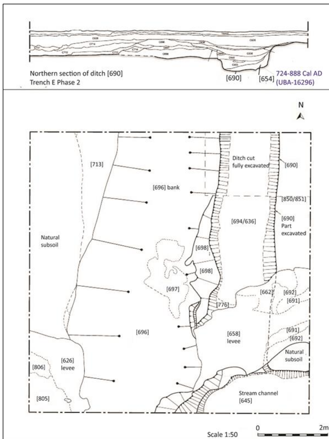
Figure 5.4.6 Ground plan and section of enclosure ditch [690] in Trench E (after O’Carragáin 2008)
