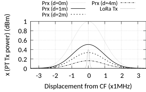
Fig. 4. LoRa ED theoretical received power ( Pr_x ) at 0, 1, 2, and 4m distance away from the PT and different frequencies as an expression of the PT transmitted power. For example, "1" means 1MHz away from the CF (CF=915MHz).
