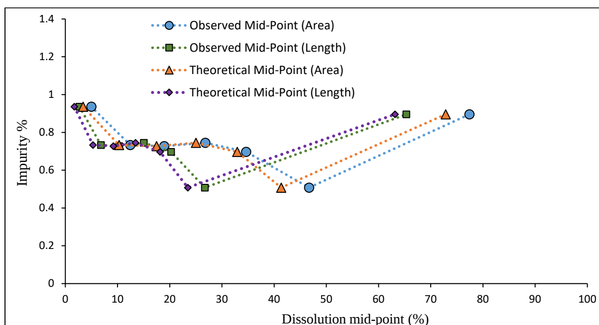
Fig. 12 Graph comparing the dissolution mid-points for 4.0 mol % 2 -doped 1 . The 'theoretical' mid-points were calculated using the microscope image analysis data to determine the volumes of equivalent spheres, reducing these by 10% for each dissolution step, and then re-calculating the lengths and areas.
