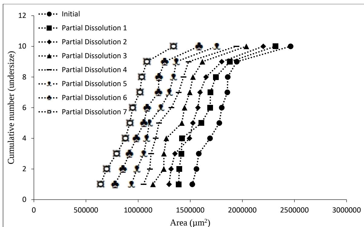
Fig. 13 Chart comparing particle area versus the ranking of each particle in a partial dissolution series of 1 doped with 4.5 mol % of 3 .
